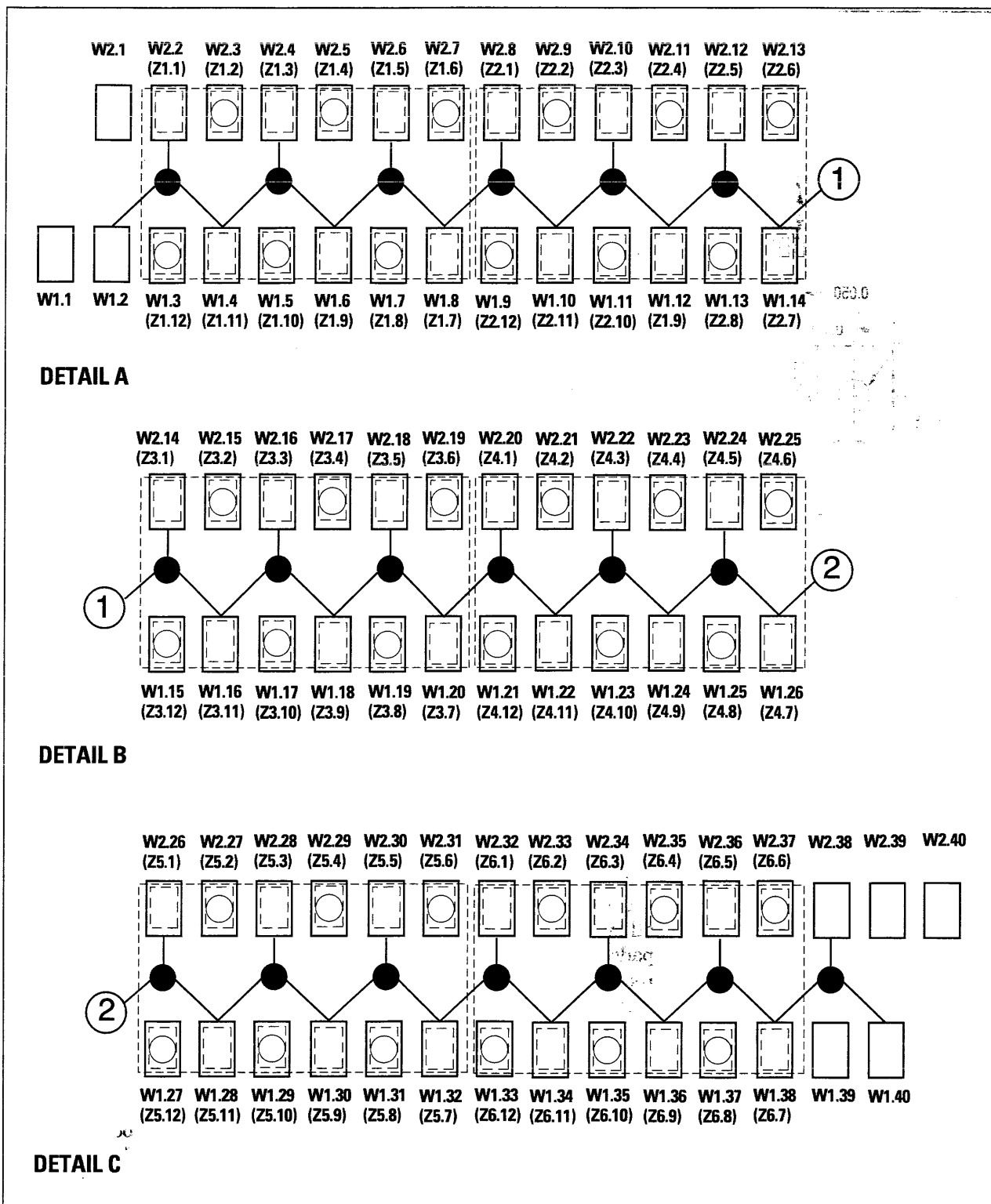
Figure 13b. Recommended PC board pattern for ribbon cable termination (when using the SMT network)
