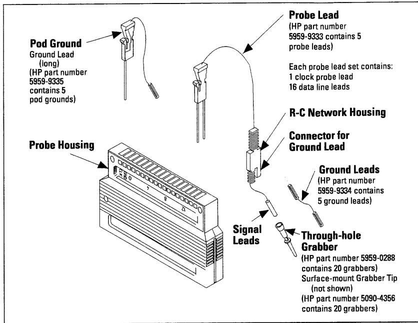
Figure 2. 16-channel probe lead set (HP part number 01650-61608)
