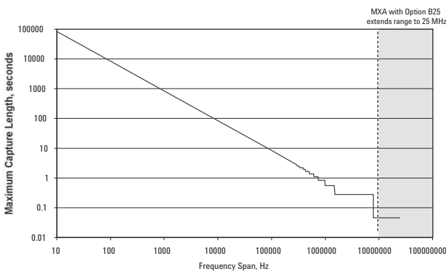
Figure 3. MXA and EXA capture length
