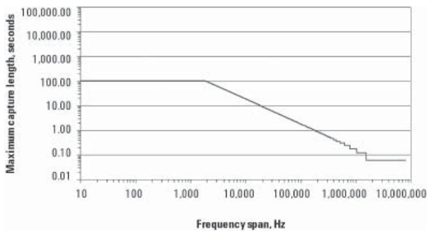
Figure 2. PSA capture length
