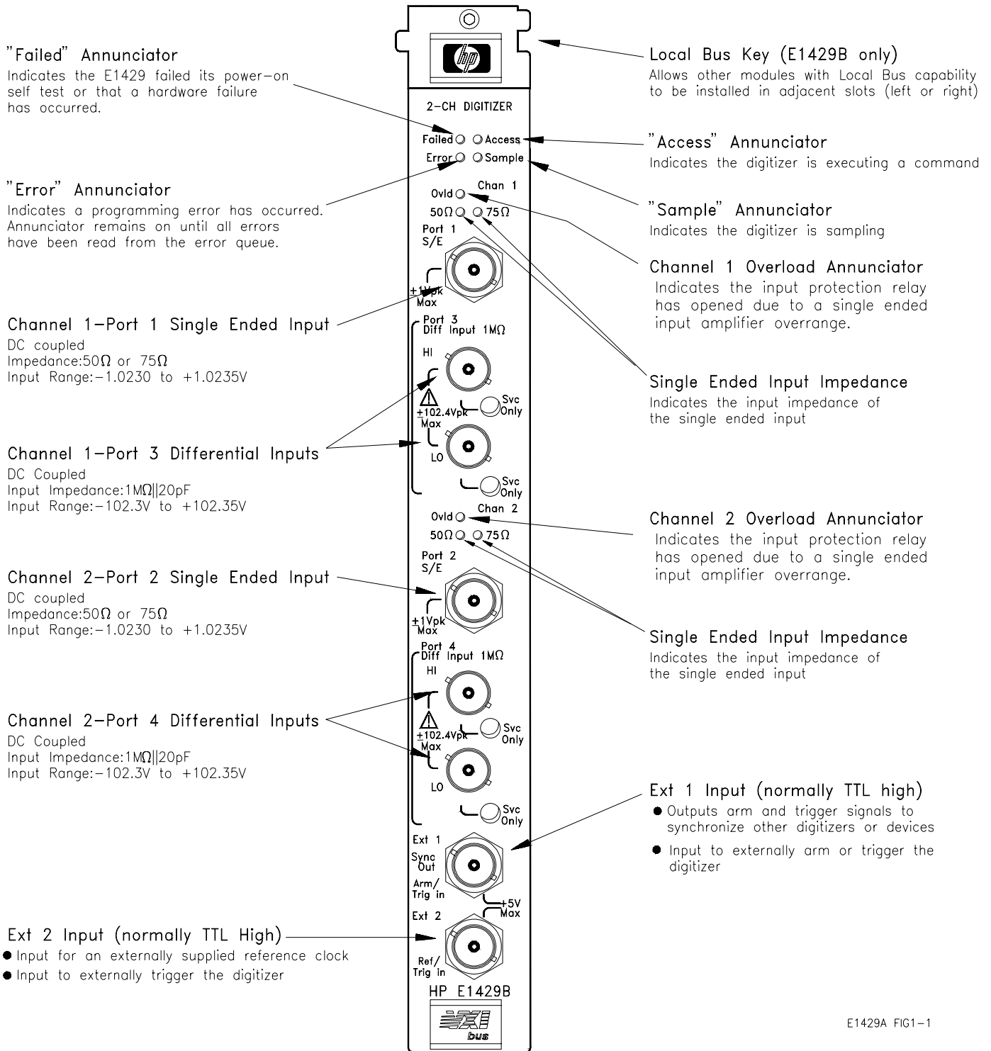
Figure 1-1. The HP E1429A/B Digitizer
