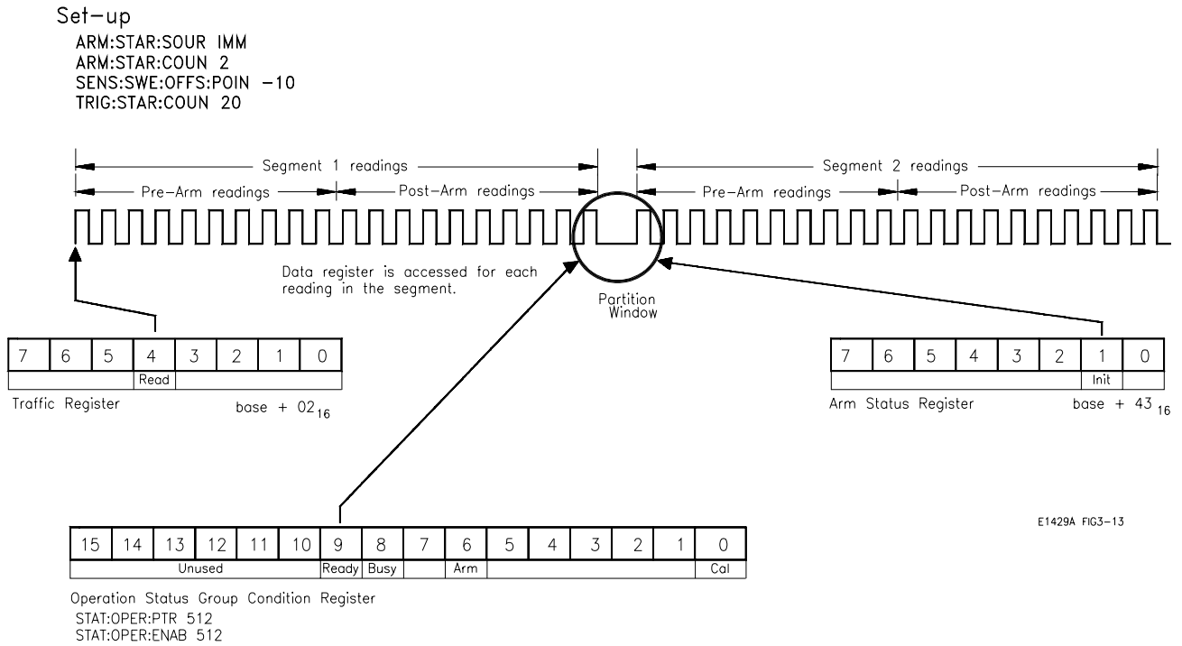
Figure 3-13. Monitoring the Partition Window During Segmented Reading Transfers
