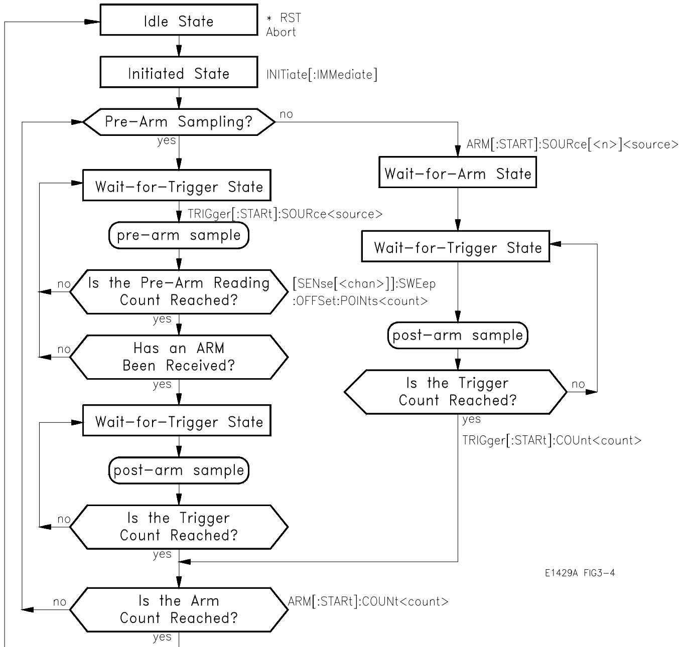
Figure 3-4. HP E1429 Digitizer State Diagram
