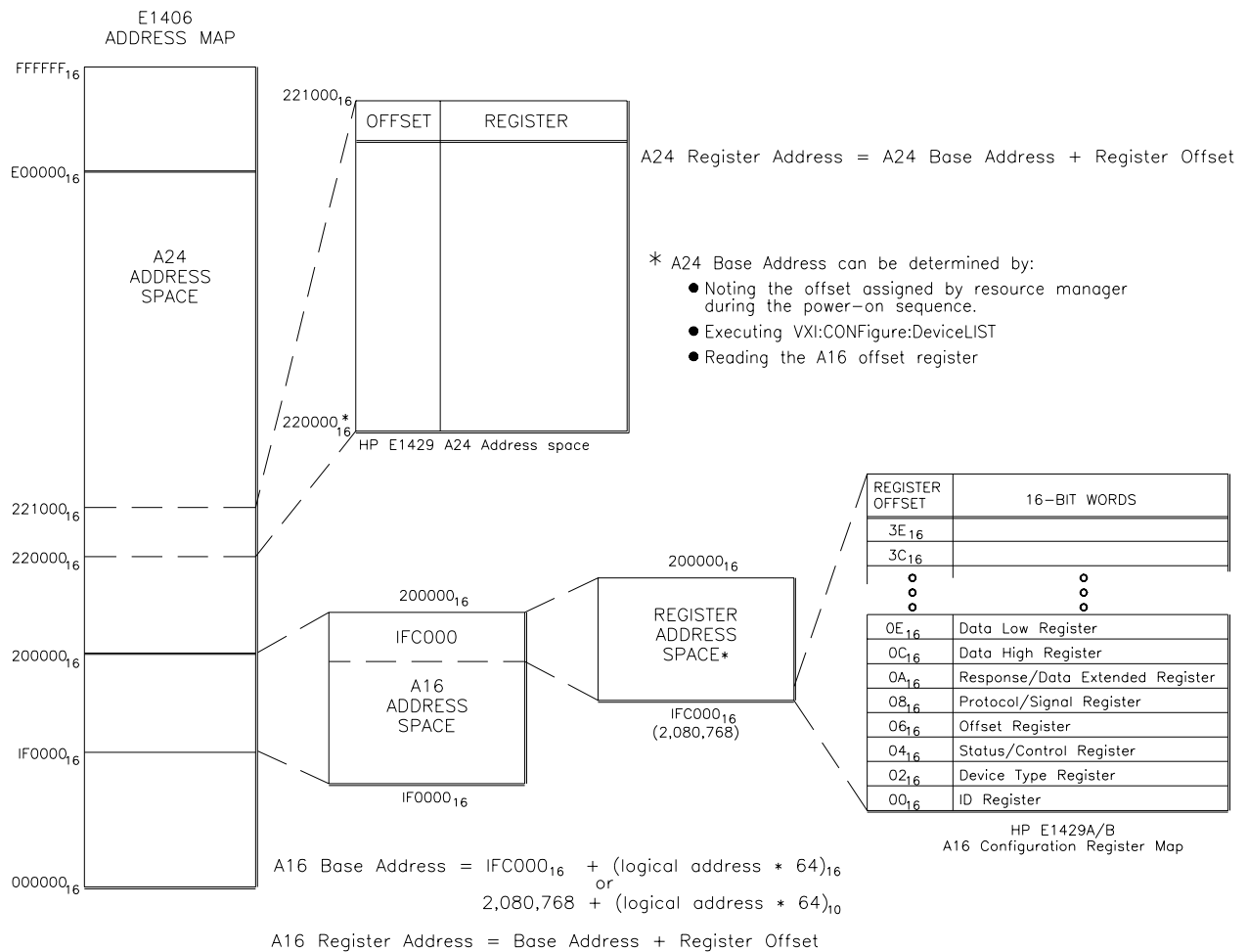
Figure C-1. HP E1429A/B A24 Address Space
