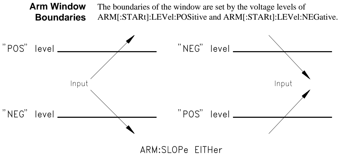
Figure 3-6. Arm Window Boundaries
