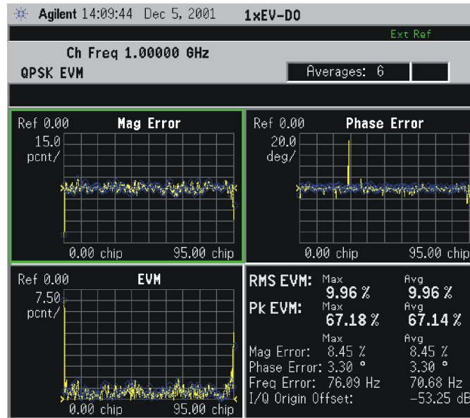
Figure 3-26 QPSK EVM Measurement - I/Q Error Quad View
