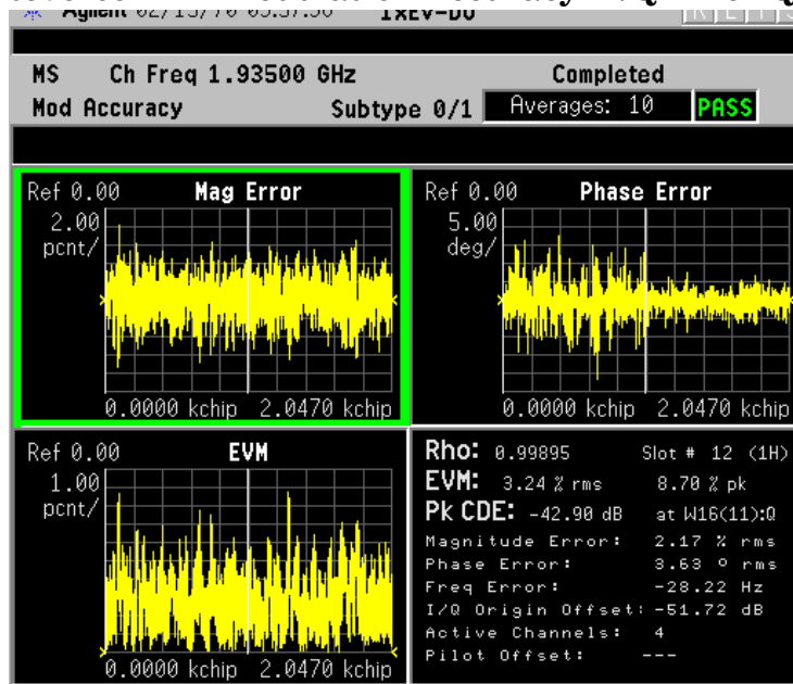
Figure 3-20 Reverse Link Modulation Accuracy - I/Q Error Quad View
