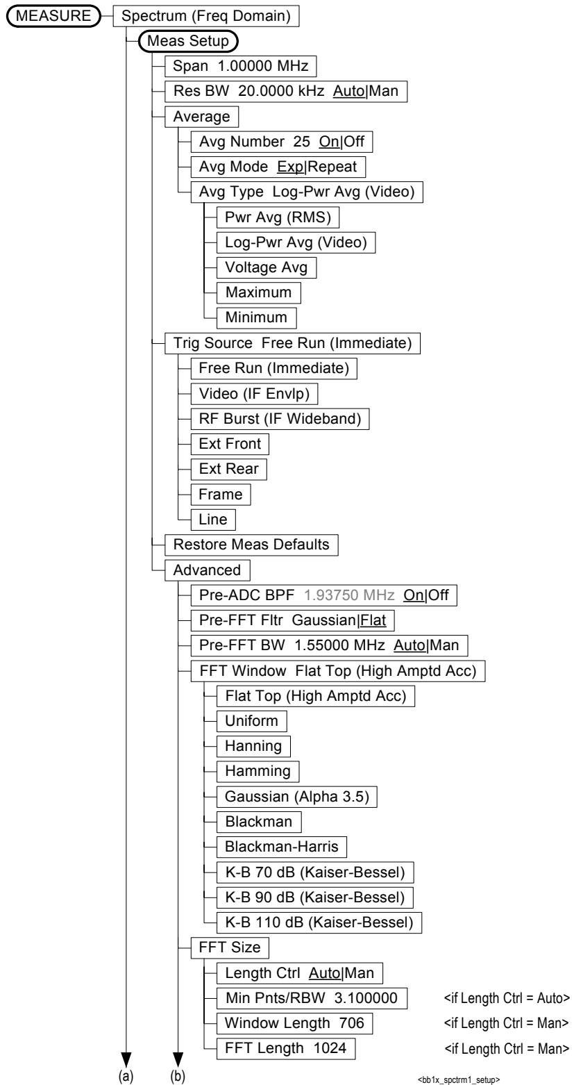
Figure 6-29 Spectrum (Freq Domain) Measurement Key Flow (1 of 4)
