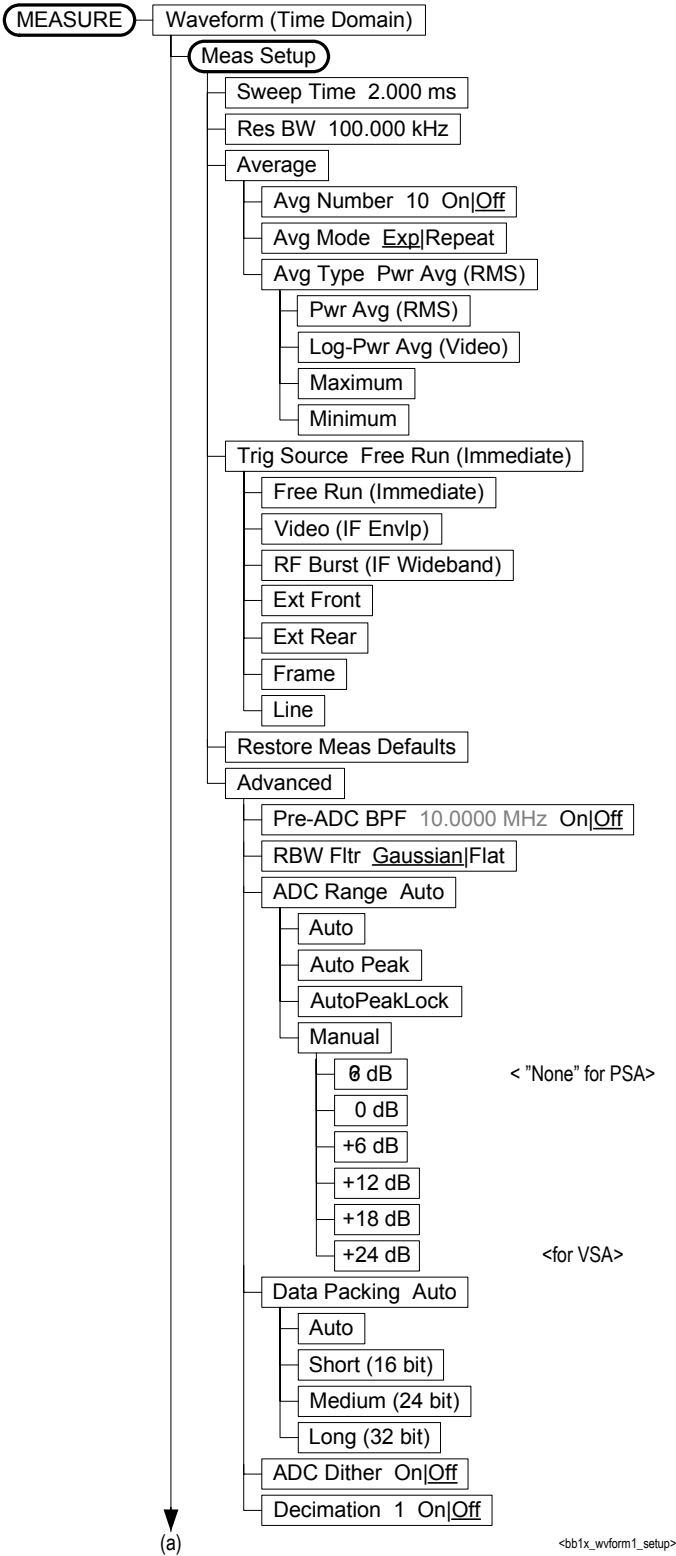
Figure 6-36 Waveform (Time Domain) Measurement Key Flow (1 of 2)
