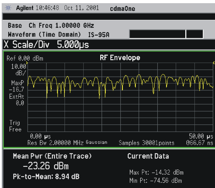
Figure 2-77 Waveform Measurement - RF Envelope (Default View)
