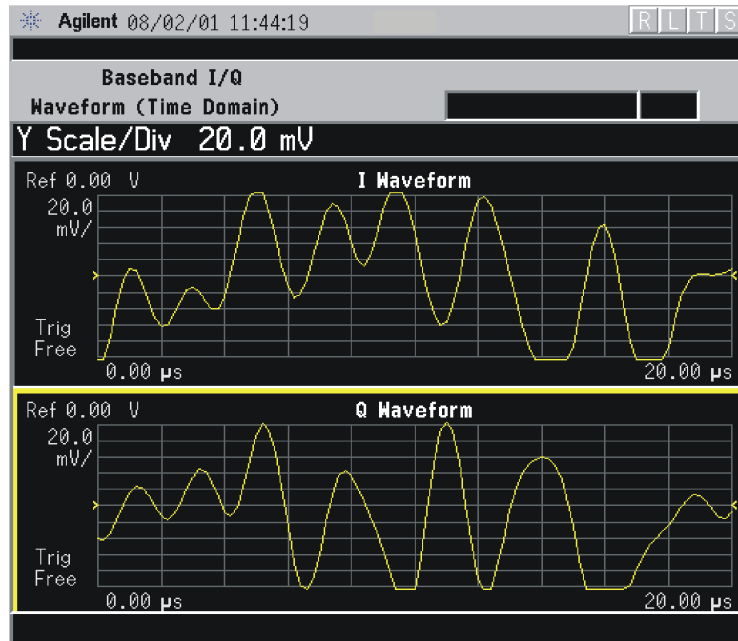
Figure 2-83 Waveform Measurement - I and Q Waveform View
