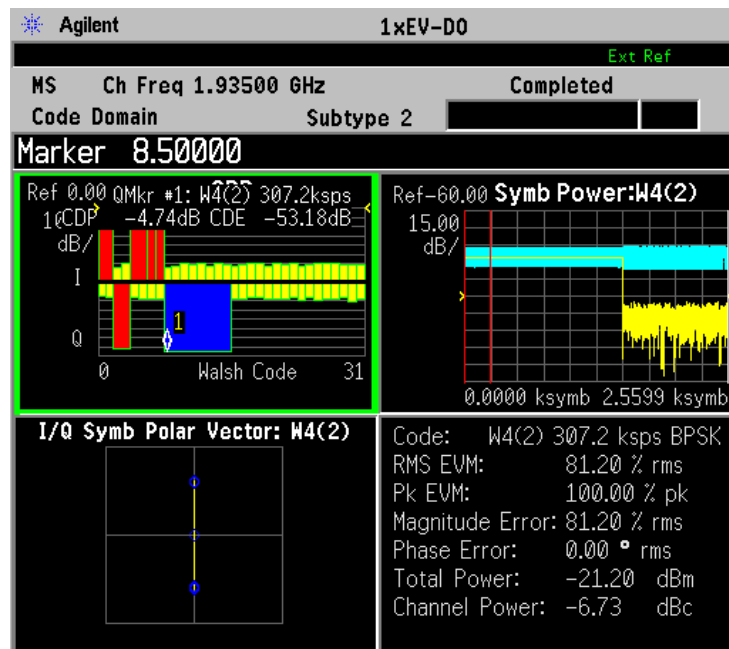
Code Domain Measurement - Code Domain (Quad View)
