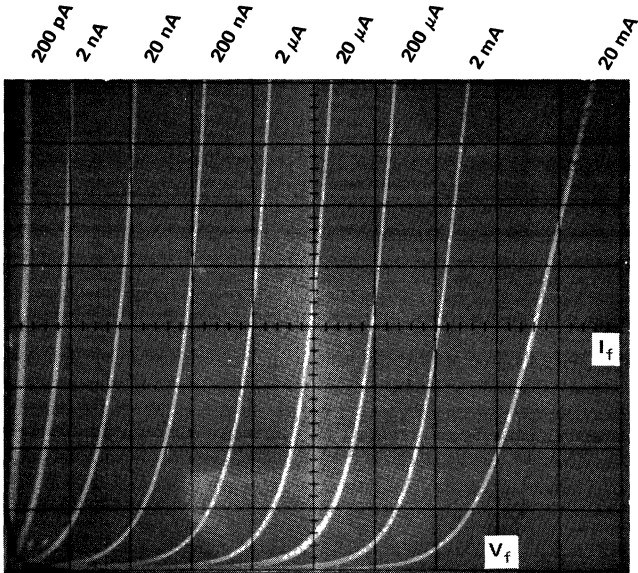
Fig. 30. Display of I_f vs. V_f for a typical diode. Each curve was traced by sweeping collector voltage manually at each current level. Photo from stored display.
