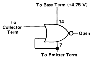
Fig. 52. TTL evaluation, I_{in}(1) condition.
