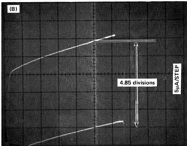
Fig. 13. Illustration of steps 14 and 15, \beta calculation.
