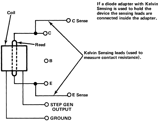
Fig. 38. Method of connecting the relay to the 177 Test Fixture.
