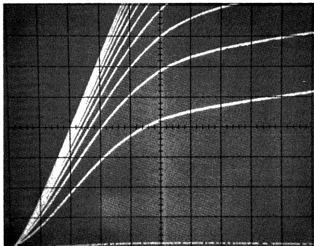
Fig. 15. Typical display of saturation Region characteristics.
