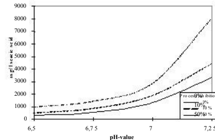
Figure 2: Interdependence of acetic acid concentration and pH-value for process inhibition
