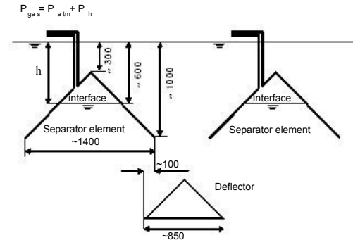
Figure 5: Submerged separators and deflector (Source: [8])
