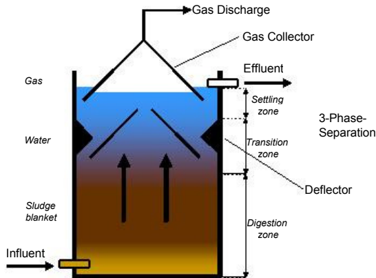
Figure 1: The UASB-Reactor (Source: TBW, modified after [6])
