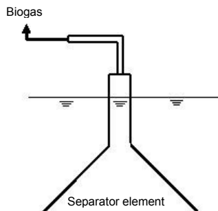
Figure 7: Separator with atmospheric gas pressure (Source: [8])
