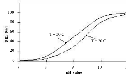
Figure 3: Dissociation rate of ammonia
