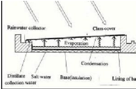
Figure 2: Solar Still Concept Diagram (Scharl, 1993)
