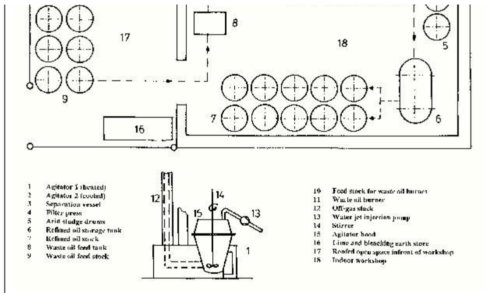
Fig. 3: Possible layout for an improved small scale Acid-Clay waste oil refining plant
