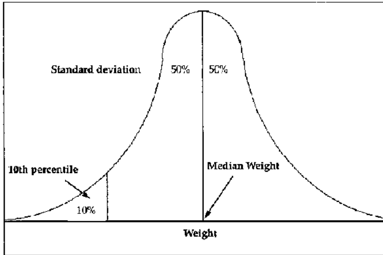
Figure 9: Normal distribution curve
