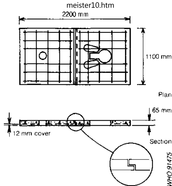
Fig. 7.15. Reinforced concrete rectangular slab (for details of reinforcement see Table 7.1)
