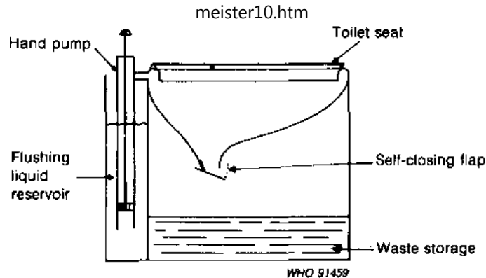
Fig. 6.40. Manually flushed chemical toilet
