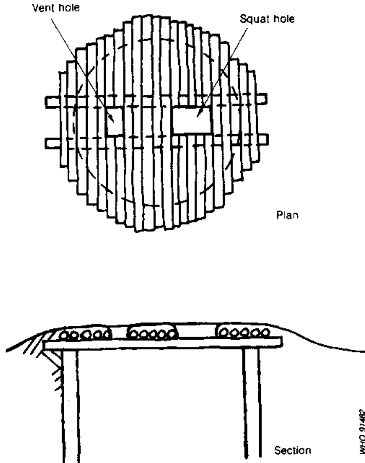
Fig. 7.22. Timber and earth slab
