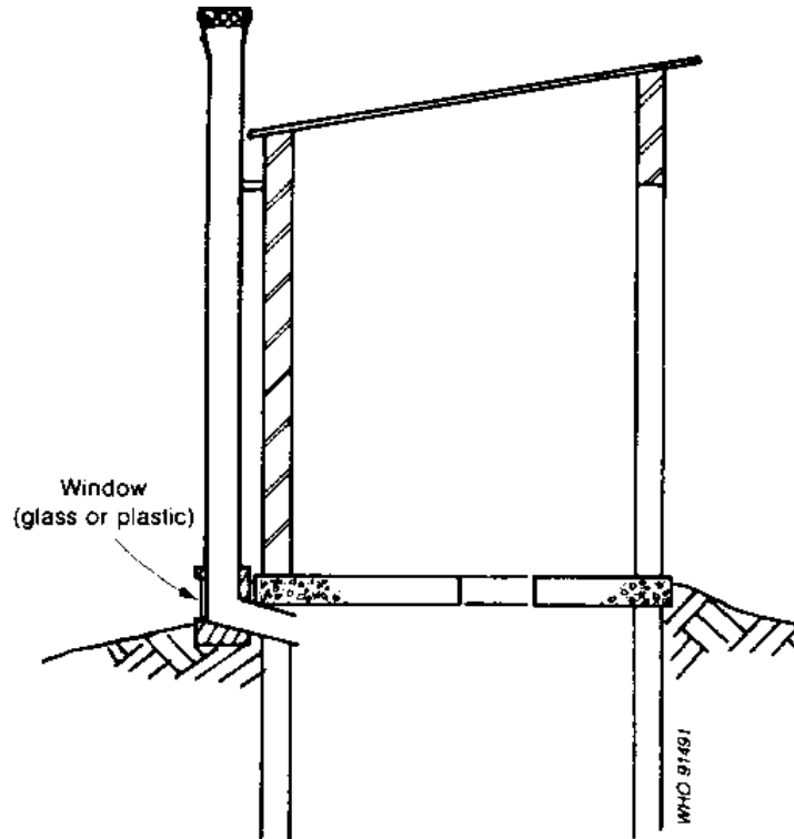
Fig. 7.31. Angled vent pipe with window
