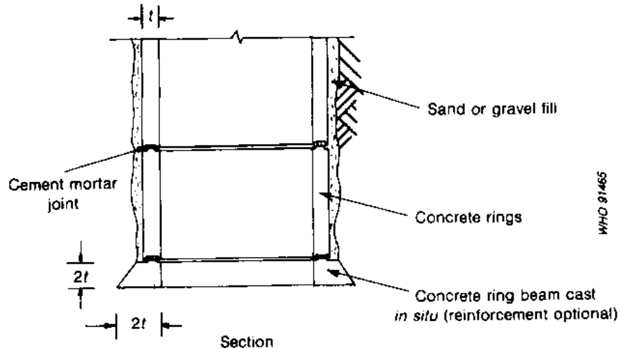
Fig. 7.5. Pit bottom lined with precast concrete rings
