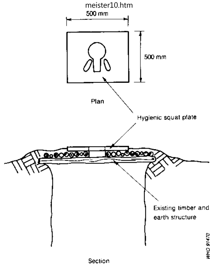
Fig. 7.10. Small slabs for upgrading timber and earth structures
