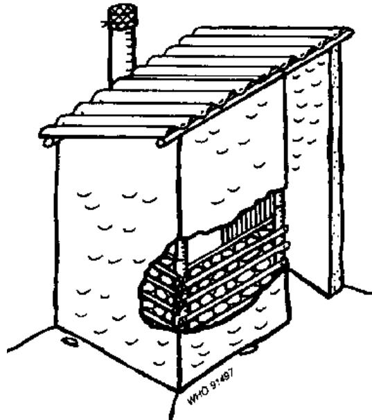
Fig. 7.37. Reinforced mud and wattle superstructure
