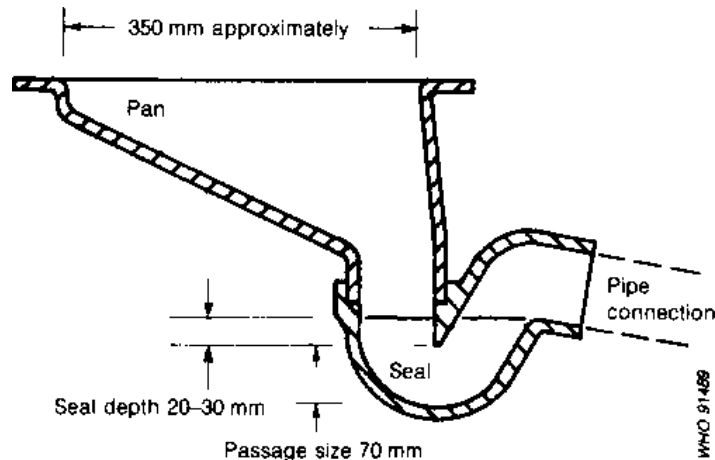
Fig. 7.29. Pan and seal for offset pour-flush latrine
