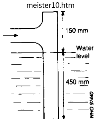
Fig. 6.21. Septic tank Inlet pipe
