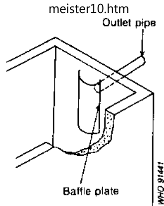
Fig. 6.22. Septic tank outlet baffle plate
