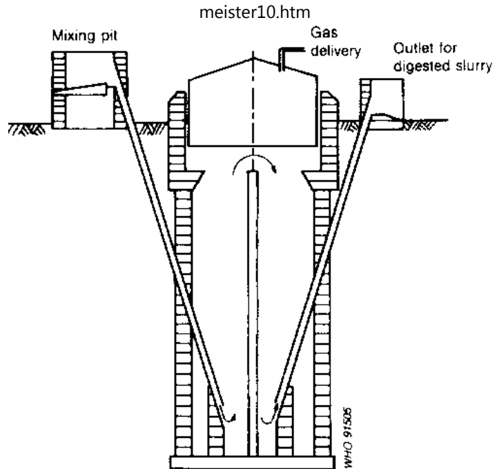
Fig. A1.5. Biogas plant with floating dome
