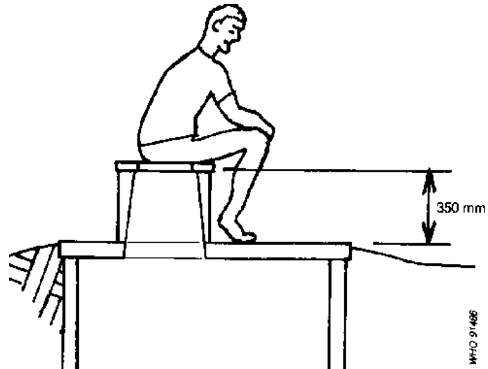
Fig. 7.26. Latrine seat
