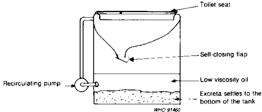
Fig. 6.41. Recirculating oil toilet
