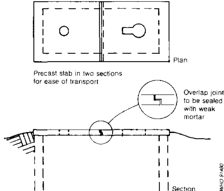
Fig. 7.20. Rectangular slab In two sections
