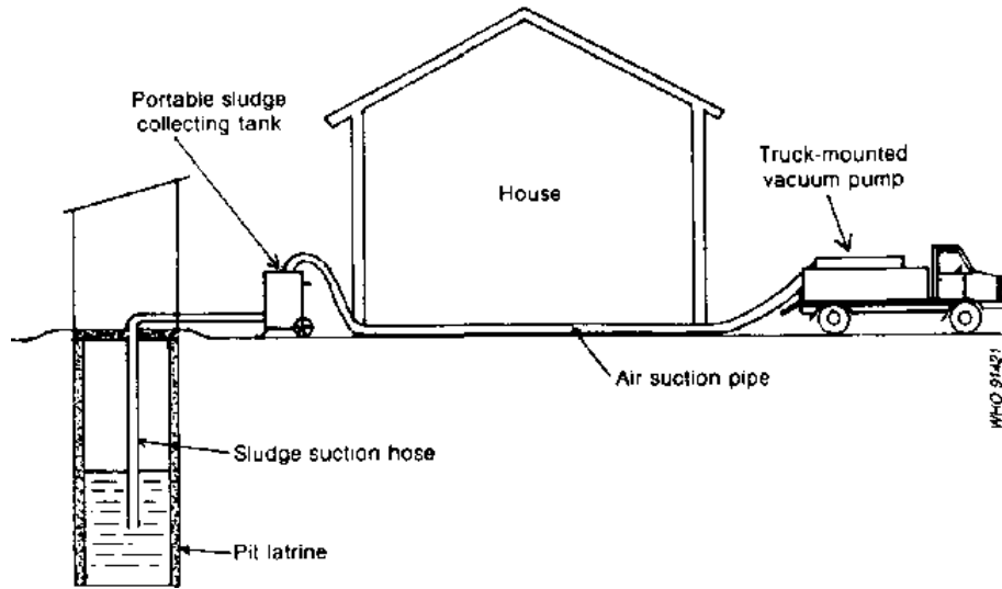
Fig. 6.2. Remote vacuum pump emptying system
