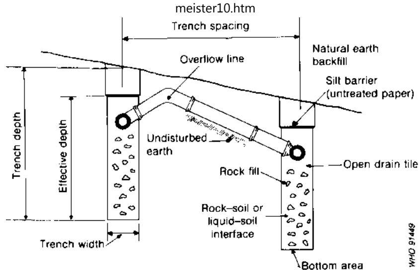
Fig. 6.30. Drainage trench
