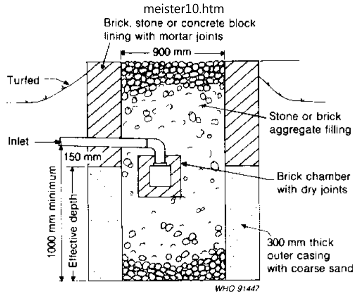
Fig. 6.28. Unlined soakpit
