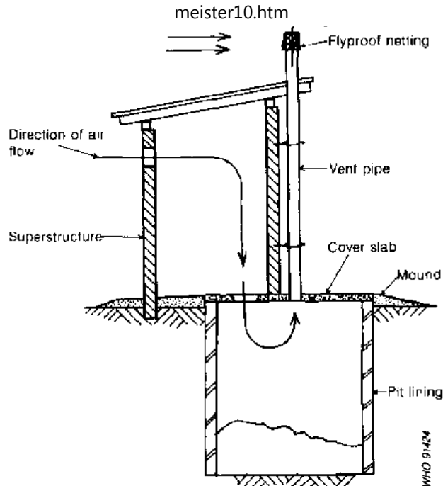
Fig. 6.5. Ventilated improved pit (VIP) latrine
