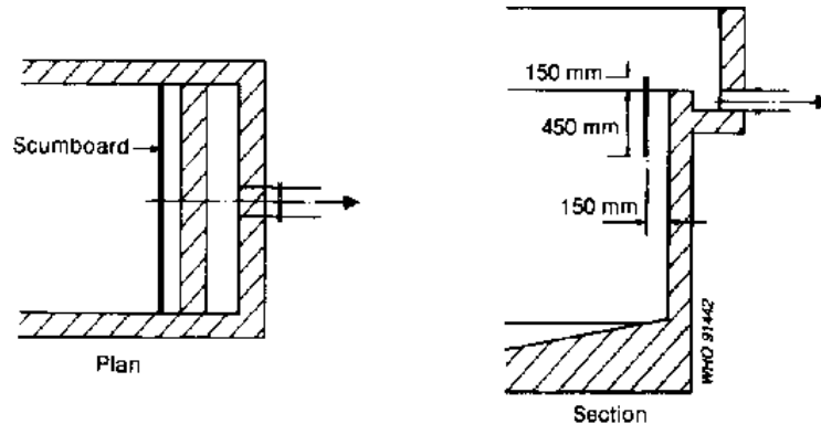
Fig. 6.23. Septic tank outlet using full width weir
