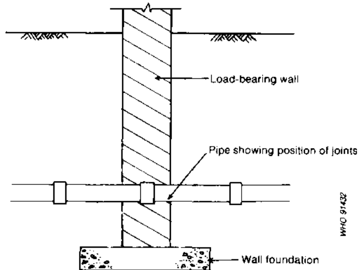
Fig. 6.12. Pipe laid through a hole in an external wall
