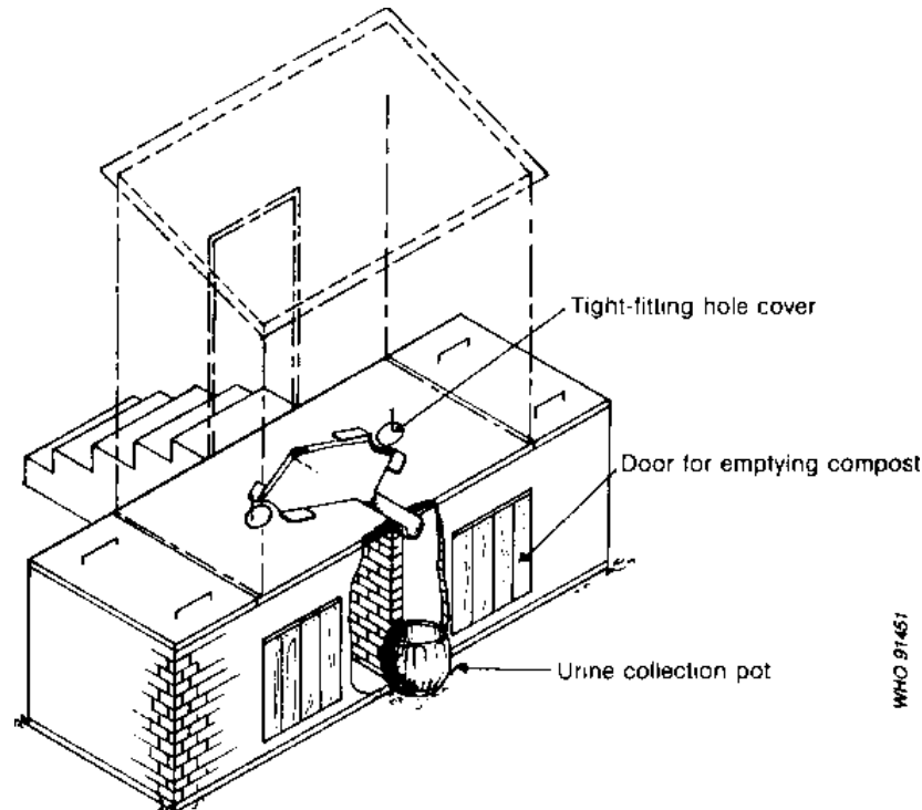
Fig. 6.32. Double-vault latrine
