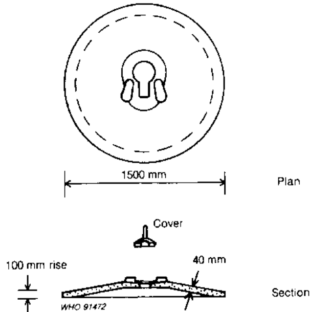
Fig. 7.12. Dimensions of domed slab without reinforcement
