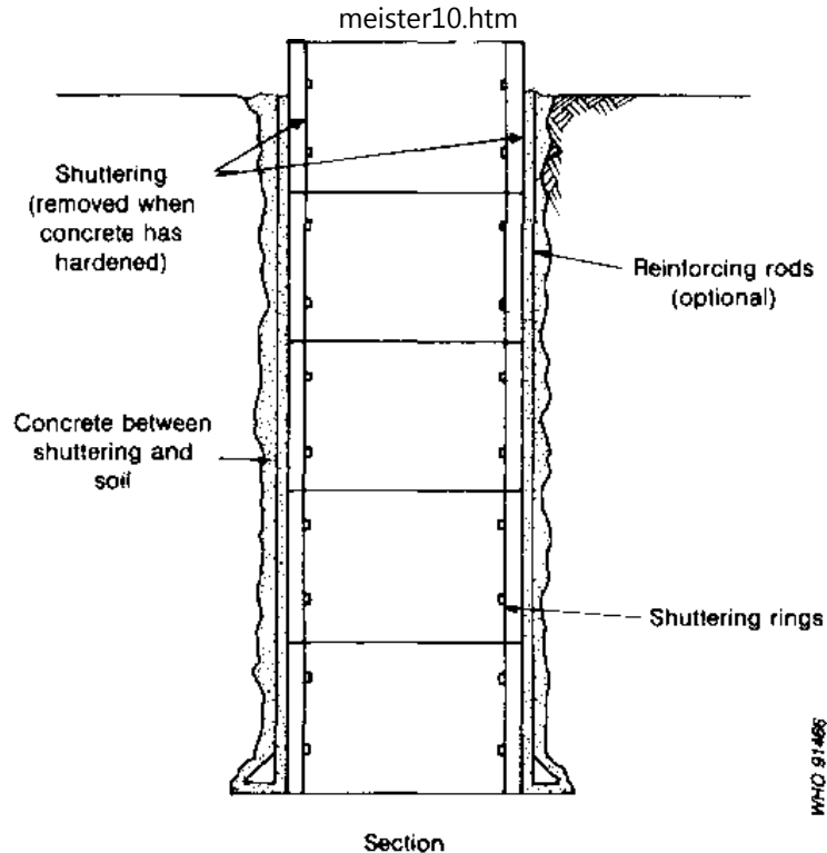
Fig. 7.6. Pit with concrete lining in situ
