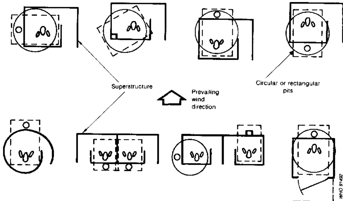
Fig. 7.32. Layouts for superstructures, vent pipes and pits
