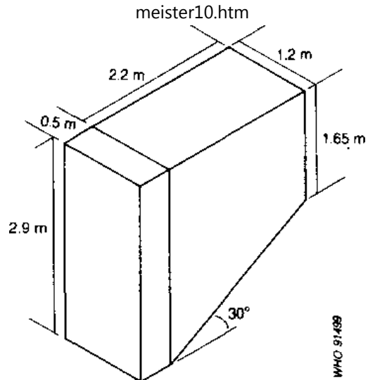
Fig. 8.2. Internal dimensions of the continuous composting toilet designed in example 8.9
