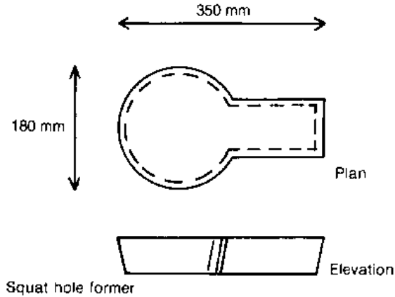
Fig. 7.25. Squat hole shapes and former
