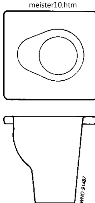
Fig. 7.27. Pedestal seat liner
