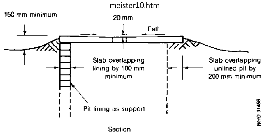
Fig. 7.8. Requirements of slabs
