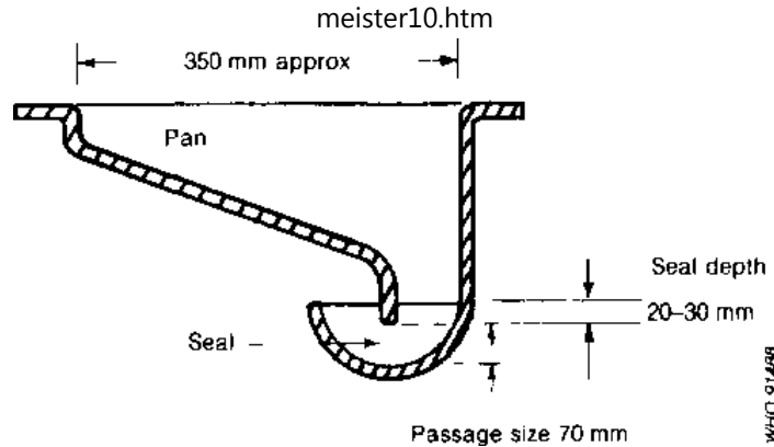
Fig. 7.28. Combined pan and water seal for direct pour-flush latrine depends on the design of the pan or pedestal, the depth and volume of the water seal, and the minimum passage size through the seal. For a water seal directly above the pit about 1 litre of water is normally sufficient for flushing. Two litres may be required for an offset pit and a minimum of 3 litres for an improved pedestal pan and offset pit.
