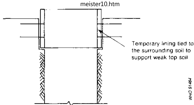
Fig. 7.4. Excavation for a pit to be lined with precast concrete rings
