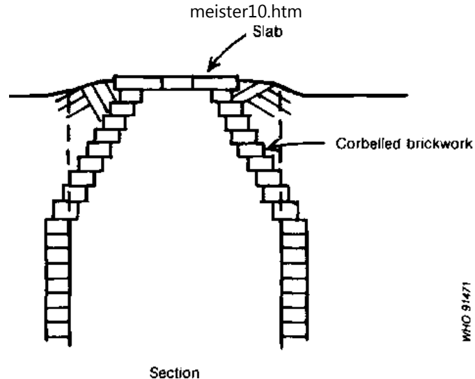
Fig. 7.11. Minimizing the span of the slab
