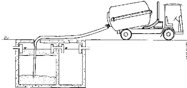
Fig. 6.1. Vacuum tanker desludging a septic tank
