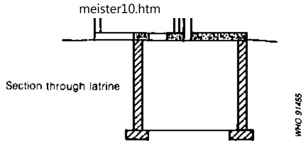
Fig. 6.36. Multiple double-pit VIP latrine
