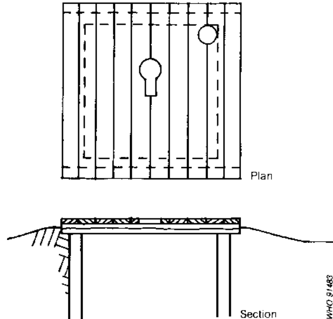
Fig. 7.23. Sawn timber slab
