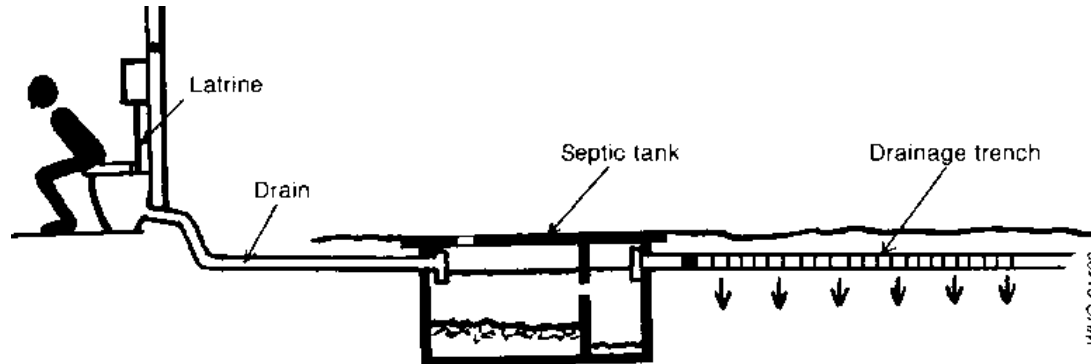
Fig. 6.19. Septic tank disposal system
