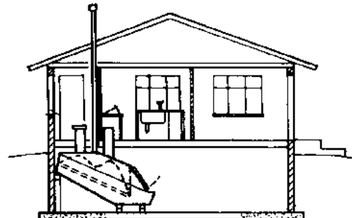
Fig. 6.34. Continuous composting toilet
