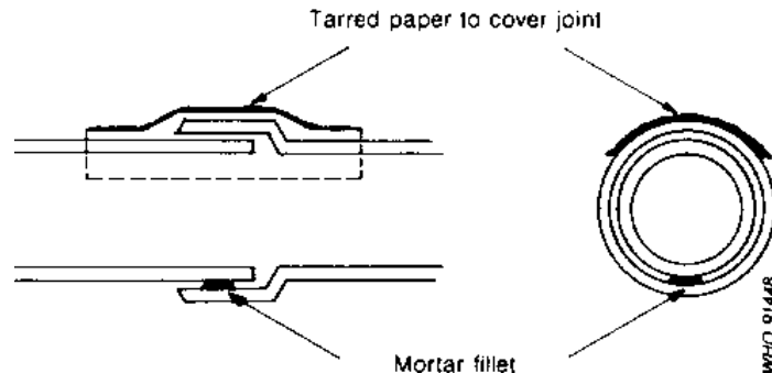
Fig. 6.29. Open pipe joint In a drainage trench
