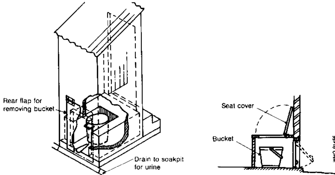
Fig. 6.37. Bucket latrine
