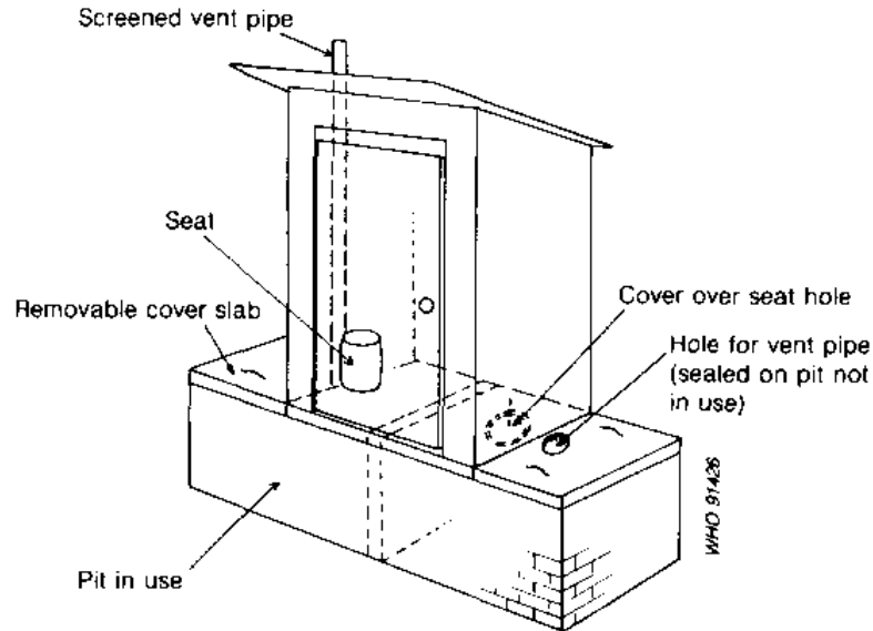
Fig. 6.7. Double-nit VIP latrine
