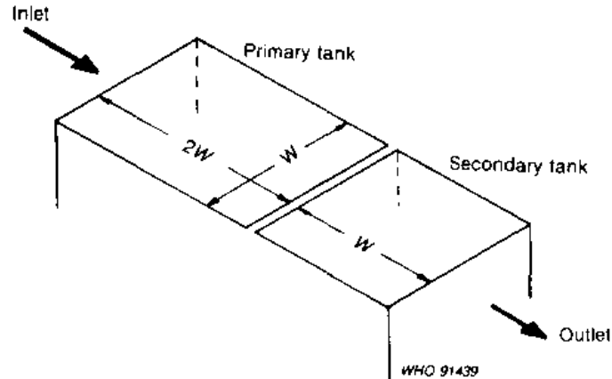
Fig. 6.20. Tank dimensions
