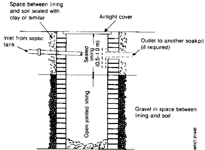
Fig. 6.27. Lined soakpit
