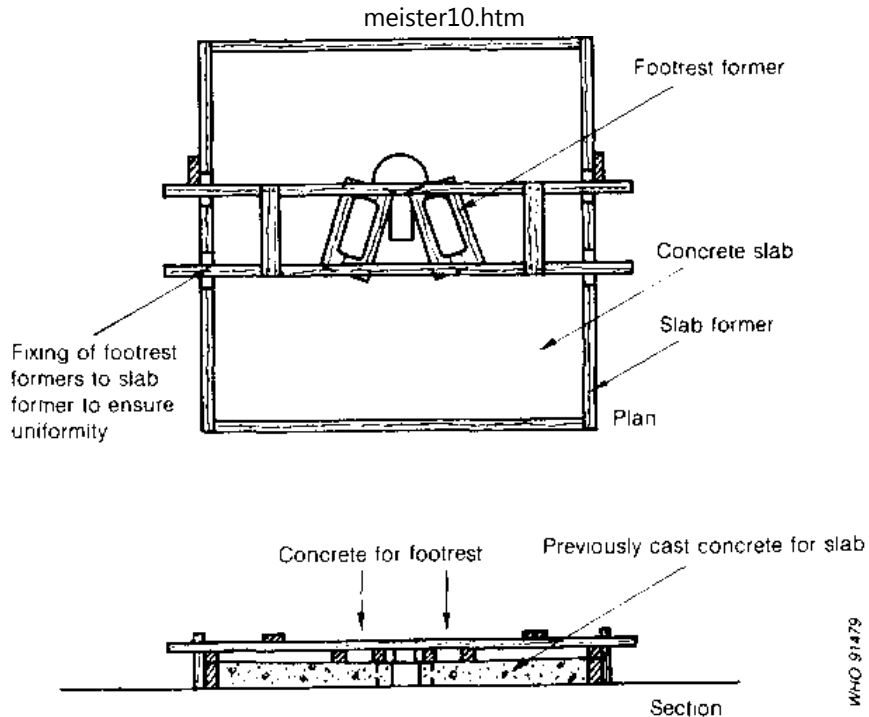
Fig. 7.19. Formwork for the casting of footrests
