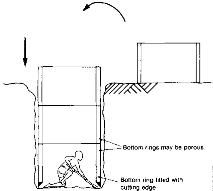
Section Fig. 7.7. "Caissoning" a pit
