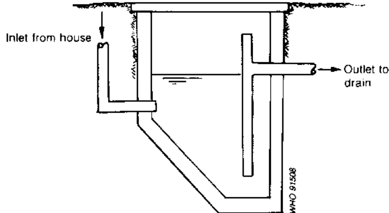
Fig. A2.2. Cross-section of a grease trap
