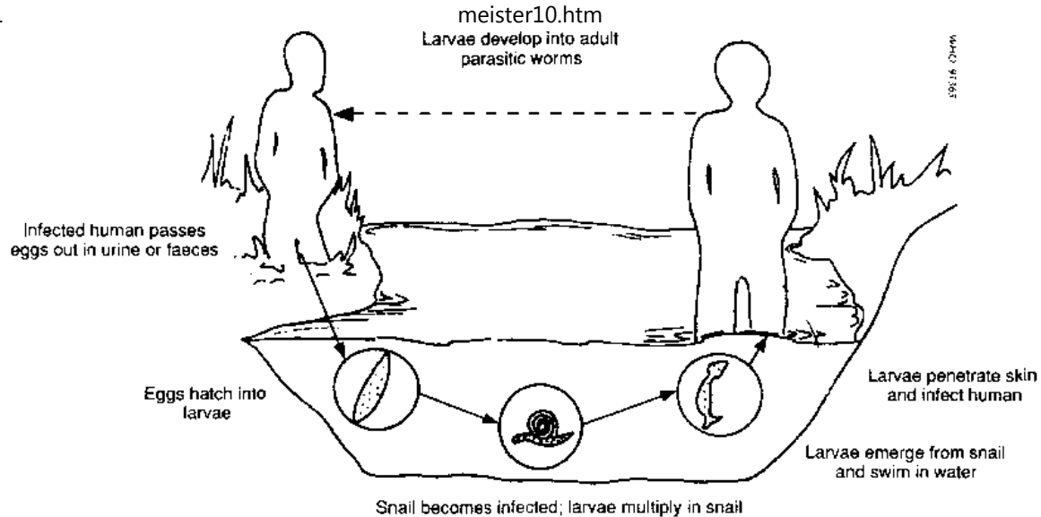
Fig. 2.2. The cycle of transmission of schistosomiasis
