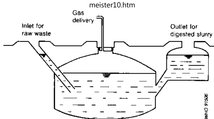
Fig. A1.6. Biogas plant with fixed dome
