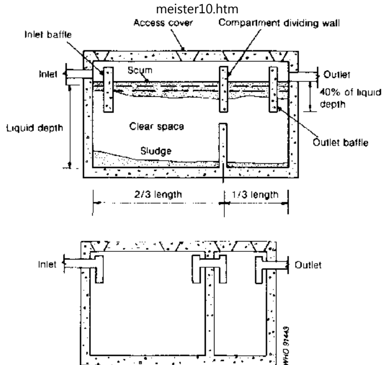
Fig. 6.24. Septic tanks showing options for connections between compartments
