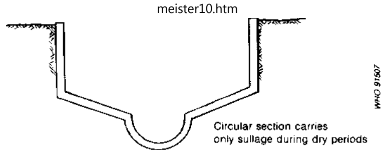
Fig. A2.1. Cross-section of a compound storm drain
