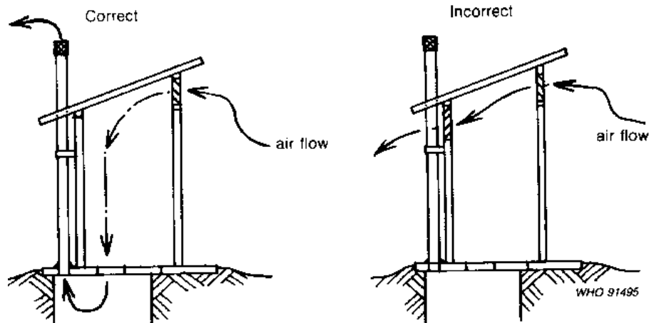
Fig. 7.35. Ventilation In a VIP latrine
