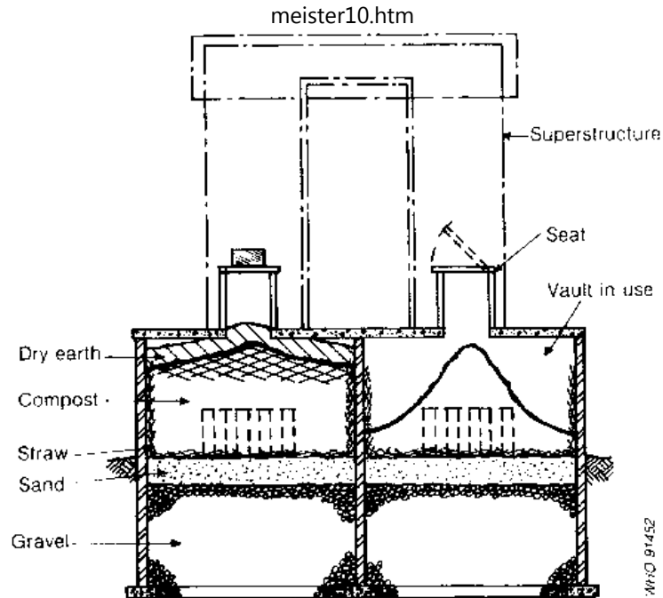
Fig. 6.33. Double-vault latrine with soakpits
