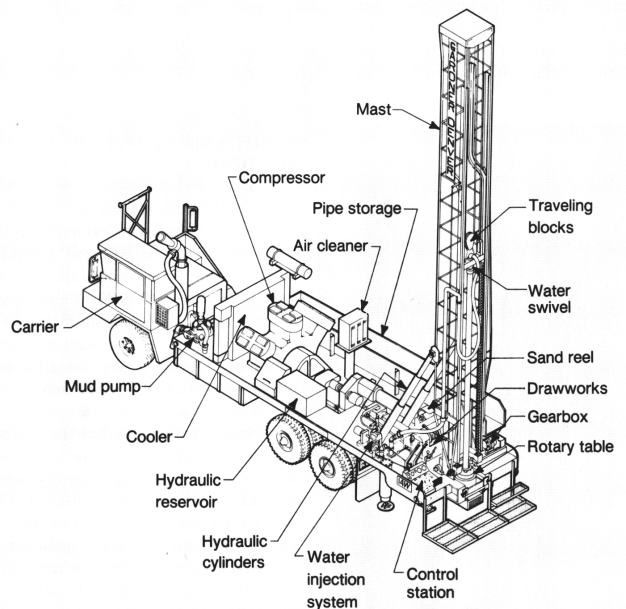
Figure 16. The 'monster' 'super rig'. In the seventies there were many such 'monsters' drilling for water in Africa, but not for long. A lack of spare parts and maintenance soon decimated these rigs - a rather inappropriate tool for a low yield borehole often far from an accessible road. Today, much smaller versions of this drill are available.
