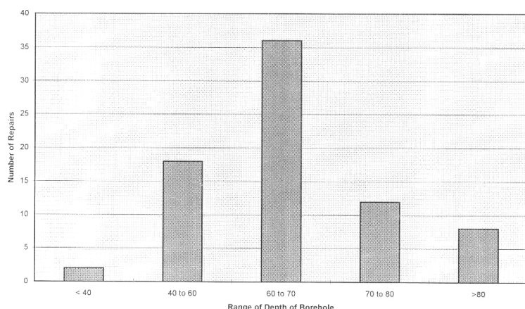
Figure 21. Depth of borehole versus number of repairs in Lesotho.
