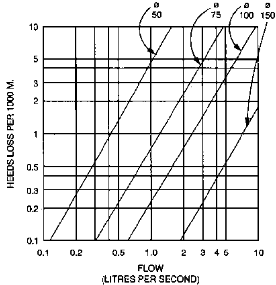
Fig. 35b Graphic Determination of Friction Head Losses in Pipes: PVC pipes*
