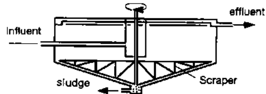
Fig. 30c Type of Sedimentation Tanks (radial flow)
