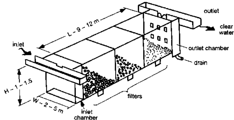
Fig. 29 Features of a Horizontal Flow Roughing Filter
