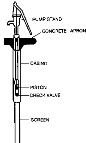
Fig. 14 "Deep Well" (Lift) Pump
