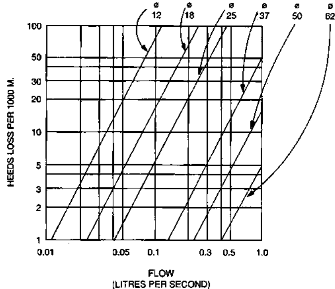
Fig. 35c Graphic Determination of Friction Head Losses in Pipes: galvanized steel pipes*
