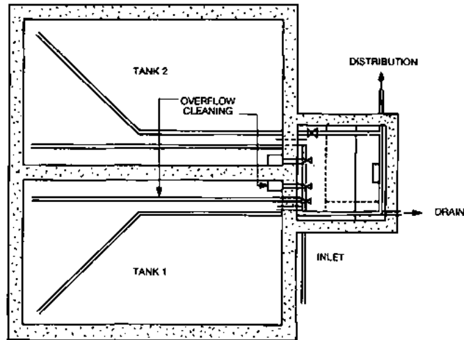
Fig. 32 Details of a Reservoir Tank
