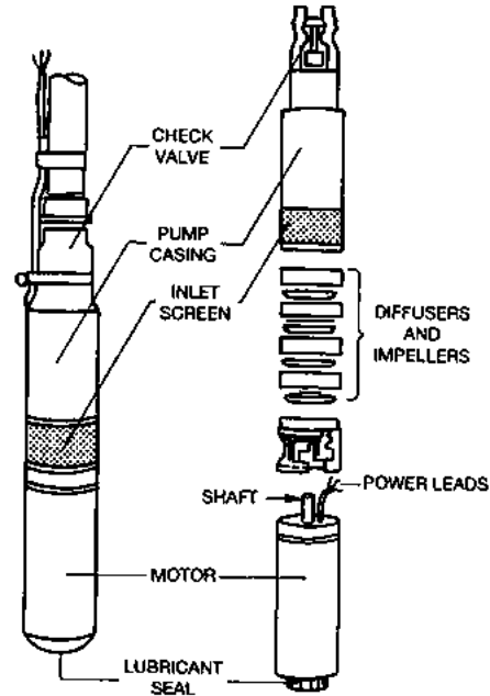
Fig. 21 Submersible Pump
