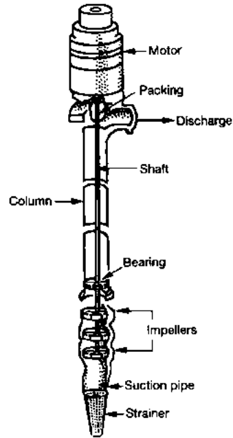
Fig. 20 Three-Stage, Shaft Driven Pump
