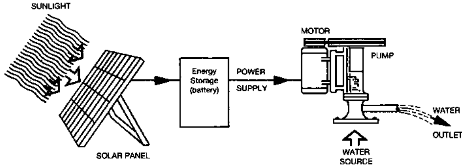
Fig. 25 Solar Powered Pumping System
