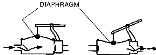
Fig. 16 Diaphragm Pumps
