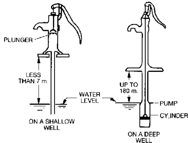
Fig. 15 Free Delivery (Force) Pumps
