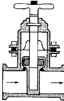
Fig. 34a Type of Valves: gate valve
