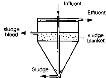
Fig. 30b Type of Sedimentation Tanks (vertical flow)
