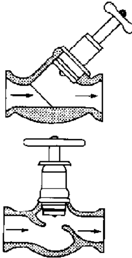
Fig. 34b Type of Valves: plug valves
