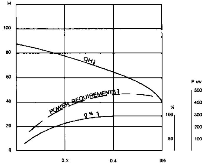
Fig. 27a Characteristic Curves (centrifugal pump)
