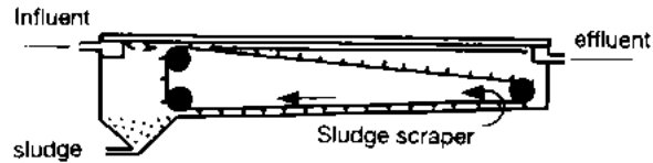
Fig. 30a Type of Sedimentation Tanks (horizontal flow)
