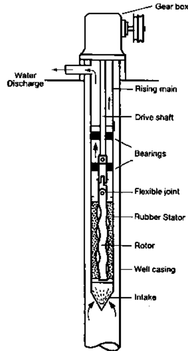
Fig. 17 Helical Rotor Pumps
