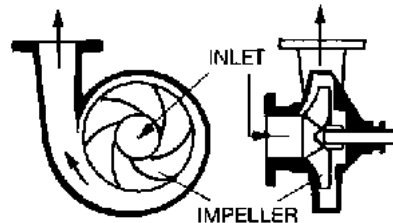
Fig. 19 Centrifugal Pump
