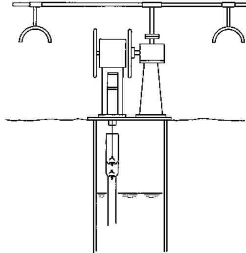
Fig. 23 Mechanism for Animal Traction Pumping
