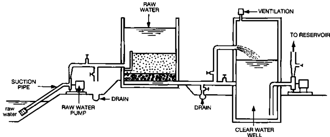
Fig. 31 Slow Sand Filtration Installations
