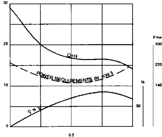
Fig. 27b Characteristic Curves (helicoidal pump)
