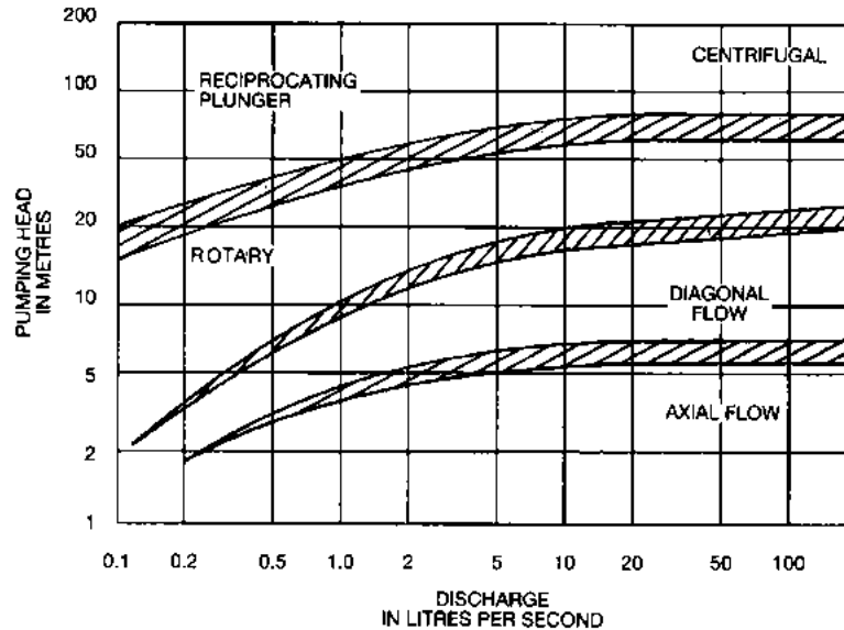
Fig. 28 Pump Type Selection Chart
