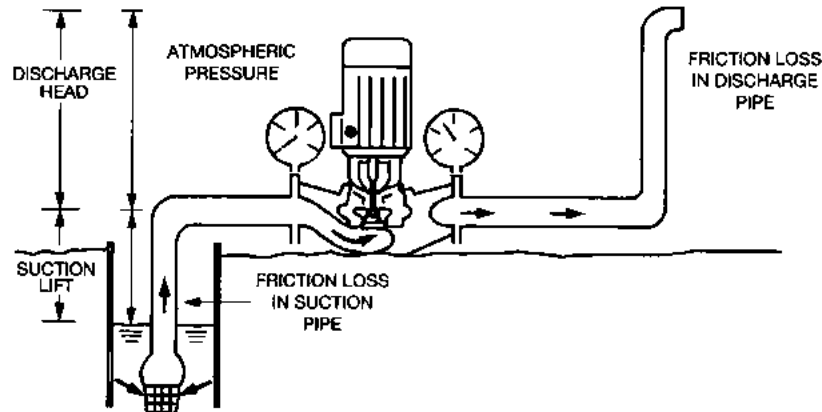
Fig. 26 Definition of Total Manometric Head
