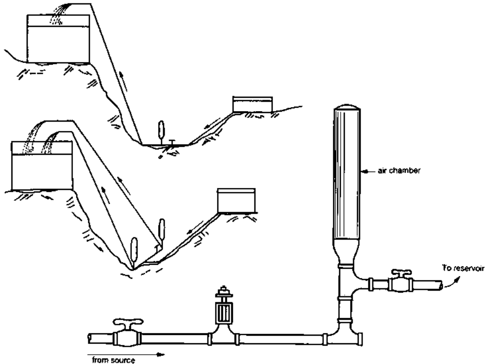
Fig. 22 Hydraulic Ram Installations
