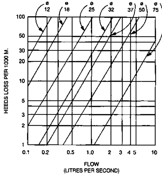
Fig. 35a Graphic Determination of Friction Head Losses in Pipes: HDPE pipes*
