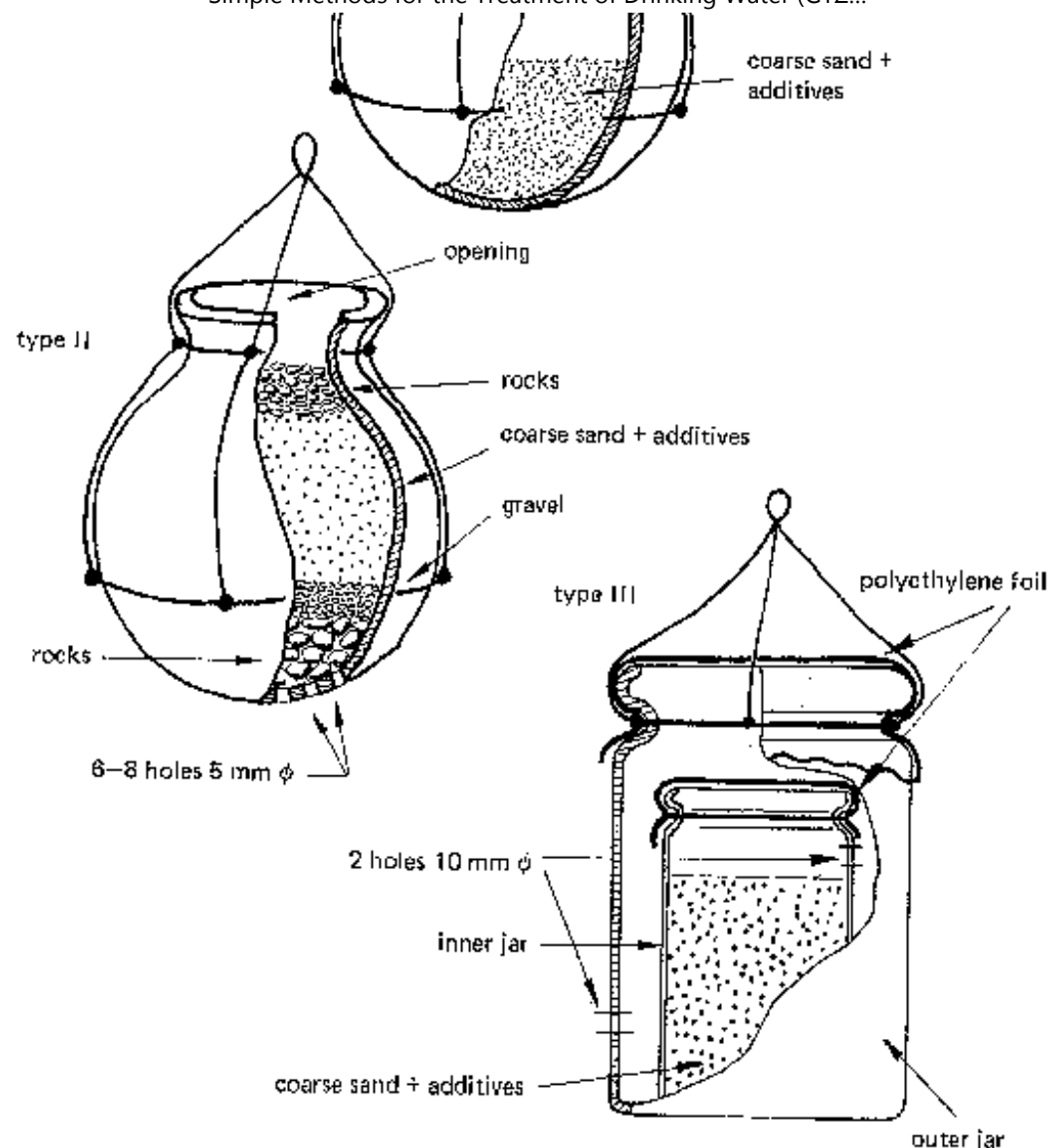
Fig. 32: Various devices for diffusion chlorination. Source: [84, 85, 51]
