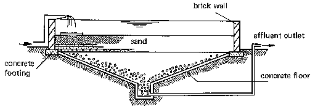
Fig. 26: Simple slow sand filter
