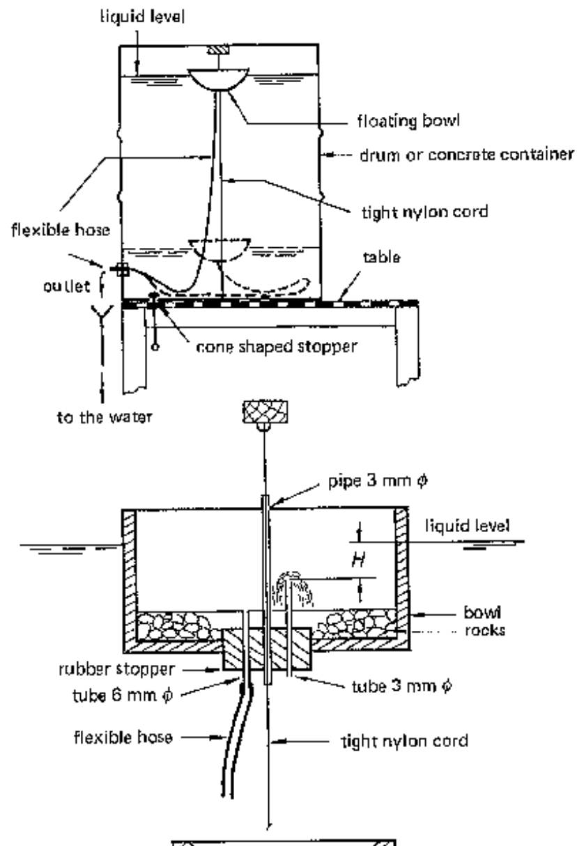
Fig. 34: Mariotte type bottles for dosing of chlorine solutions. Sources: [44, 46, 89, 91].
