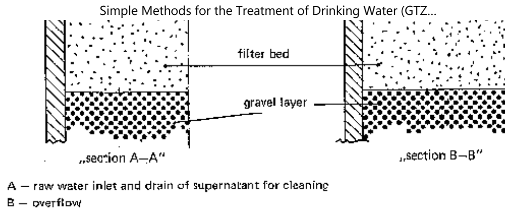
Fig. 24: Different design arrangements for their inlet zone of a slow sand filter
