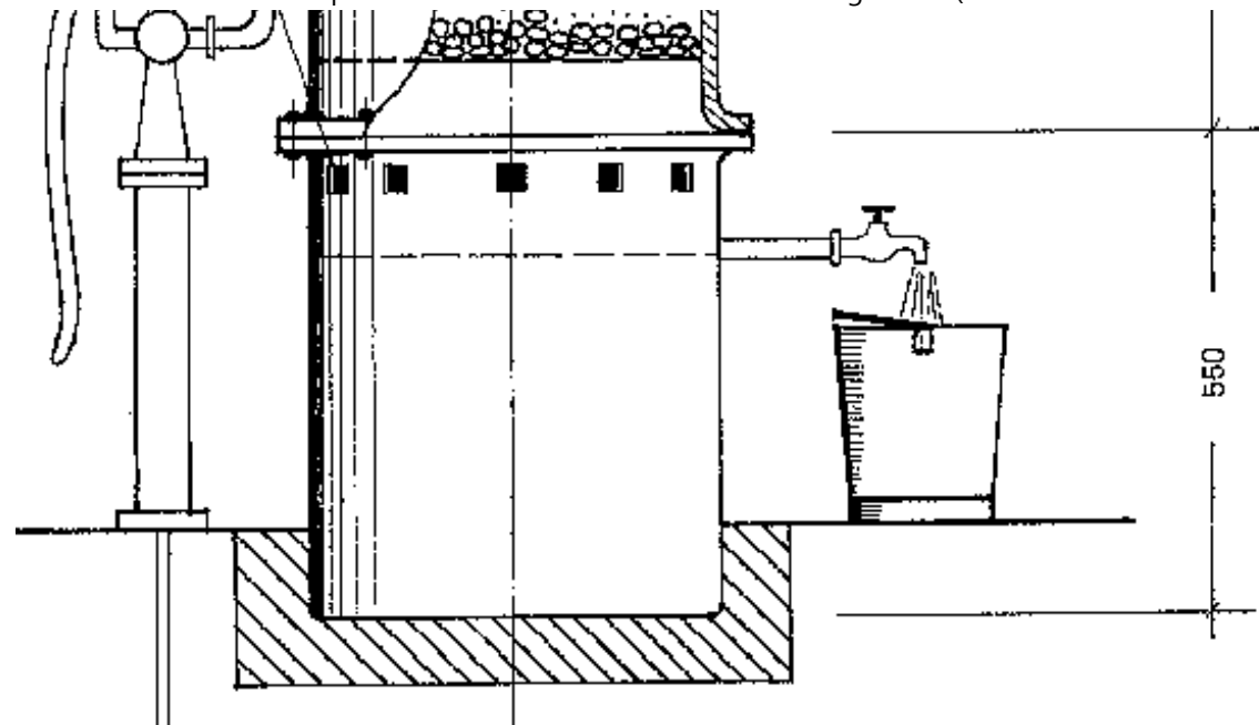
Fig 5: Manual device for removal of iron and manganese; capacity 200 a/h. Sources: [32, 46, 51, 57]
