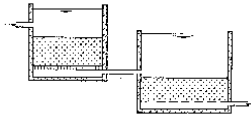
Fig. 14: Coarse filtration followed by slow sand filtration
