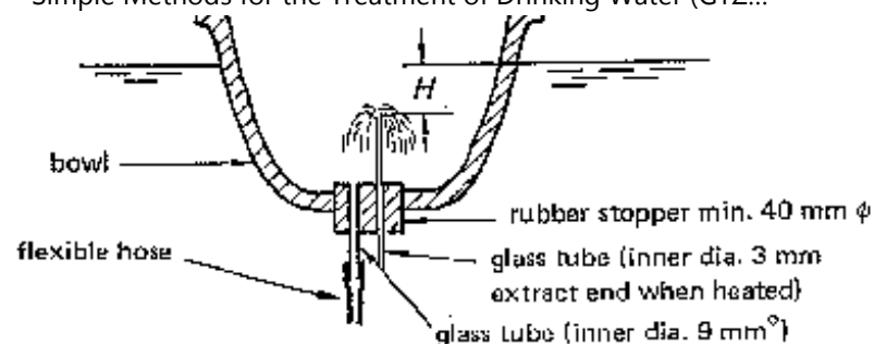
Fig. 35: Drip dosing devices with floating bowl. Source: [51, 56, 88].
