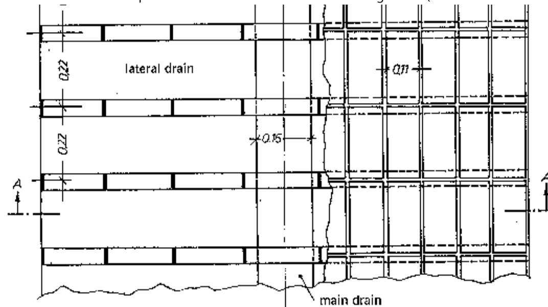
Fig. 22: Drainage system consisting of bricks [83]. The system can be arrayed such that the main drain runs along the side of the tank.
