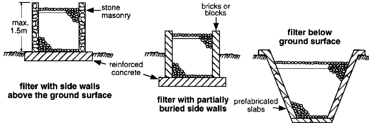
Fig. 45 Location and Materials of Roughing Filter Boxes
