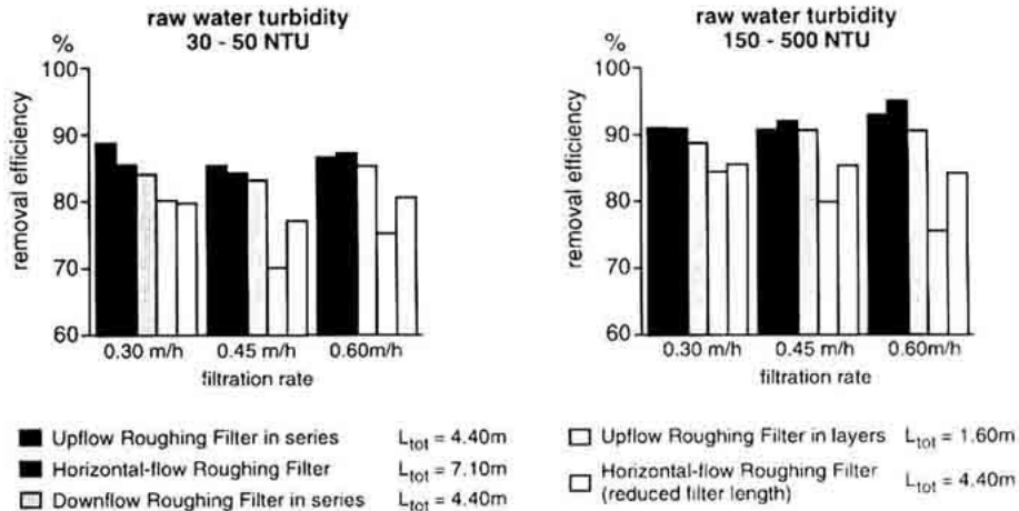
Fig. 40 Turbidity Removal by Different roughing filters
