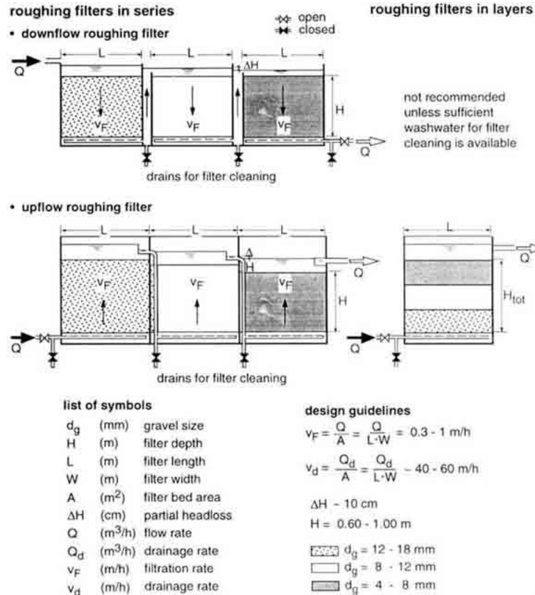
Fig. 38 Layout and Design of Vertical-flow Roughing Filters
