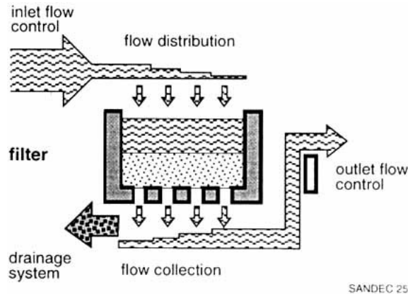
Fig. 25 Main Features of a Filter
