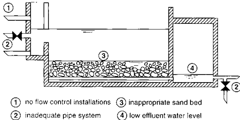
Fig. 13 Common Design Faults of Slow Sand Filters
