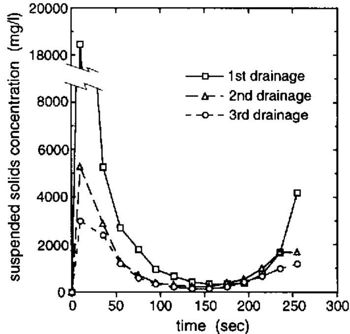
Fig. 52 Suspended Solids Concentration in Washwater of Three Subsequent Filter Drainage Cycles
