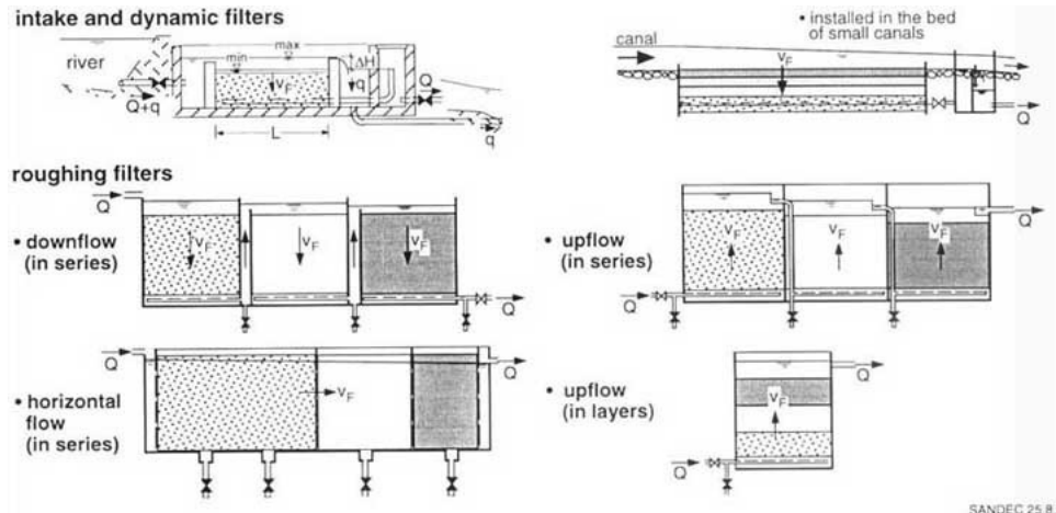
Fig. 9 Classification of Prefilters
