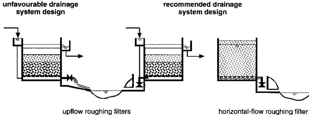
Fig. 48 Levelling of the Drainage System
