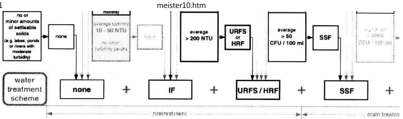
Fig. 55 Treatment Option for a Lowland Stream
