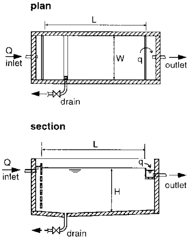
Fig. 7 Layout and Design of a Sedimentation Tank
