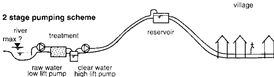
Fig. 16 General Layout of Pumped Water Supply Schemes
