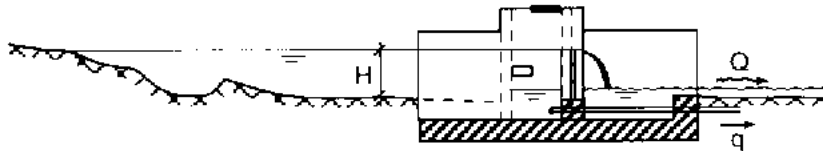
Fig. 6 Layout and Design of a Stilling Basin
