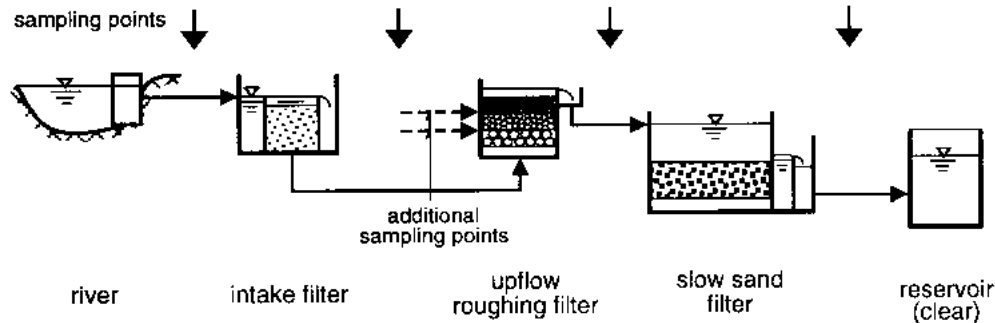
Fig. 51 Location of Water Sampling Points
