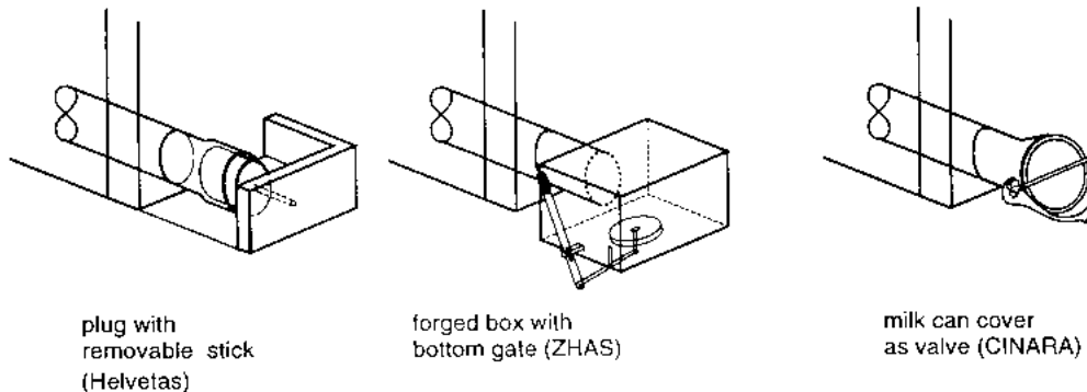
Fig. 34 Layout of Fast Opening Devices for Filter Drainage
