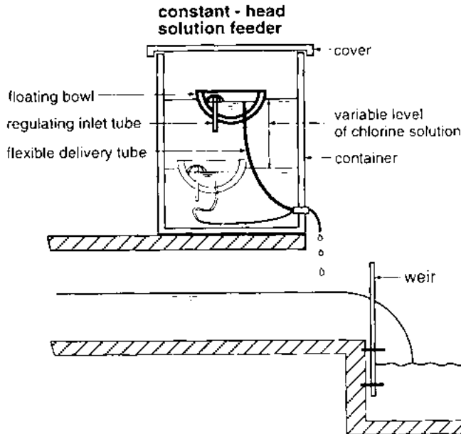
Fig. 14 Application of Chlorine
