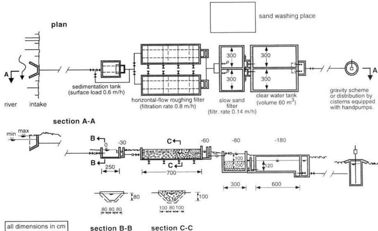
Fig. 20 Example of a Water Treatment Layout
