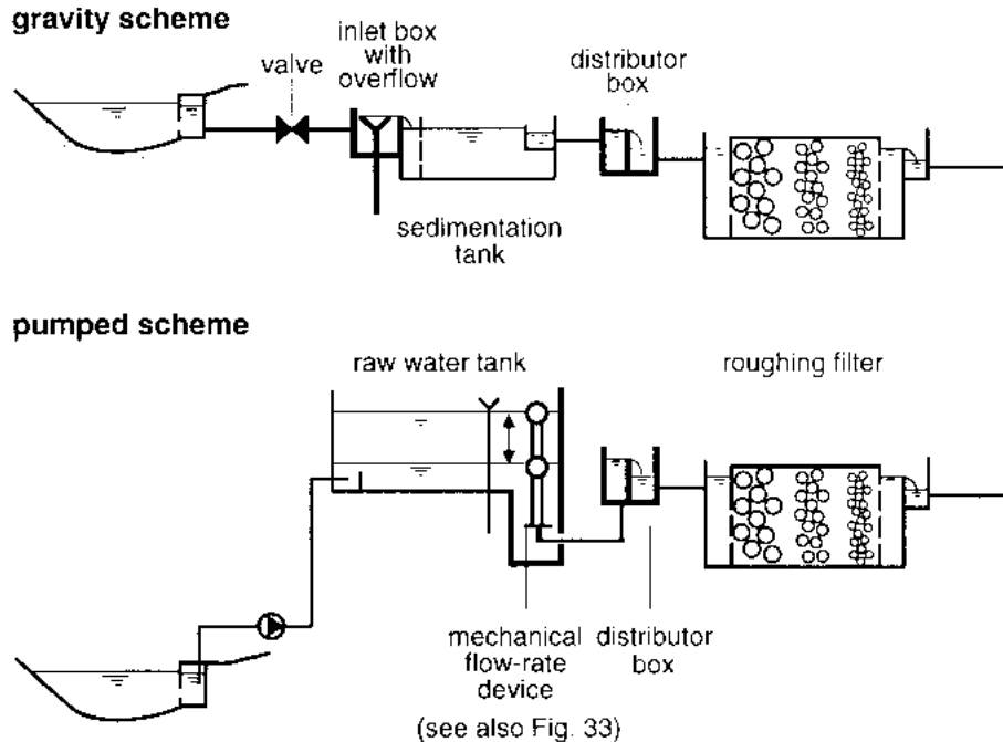
Fig. 21 Raw Water Supply and Flow Control
