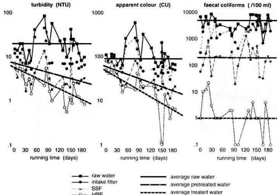
Fig. 42 Turbidity, Apparent Colour and Faecal Coliform Reduction at the Treatment Plant La Javeriana, Colombia
