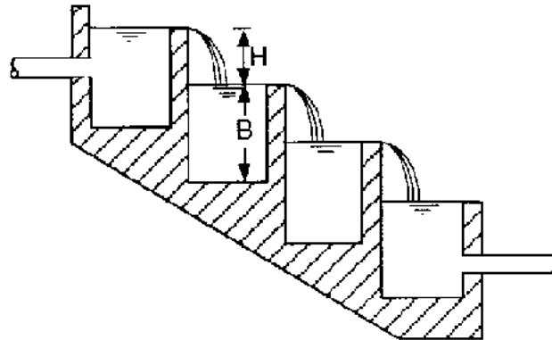
Fig. 19 Layout and Design of an Aeration Cascade
