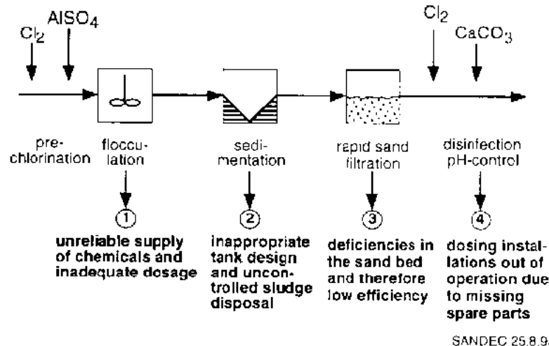
Fig. 1 Operational Problems in Conventional Water Treatment Plants
