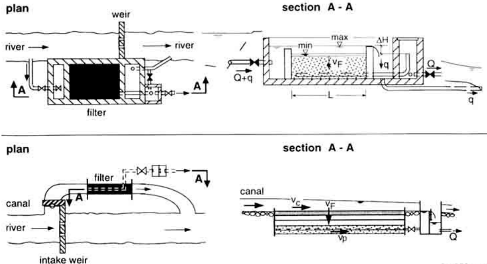
Fig. 36 Layout of Intake and Dynamic Filters
