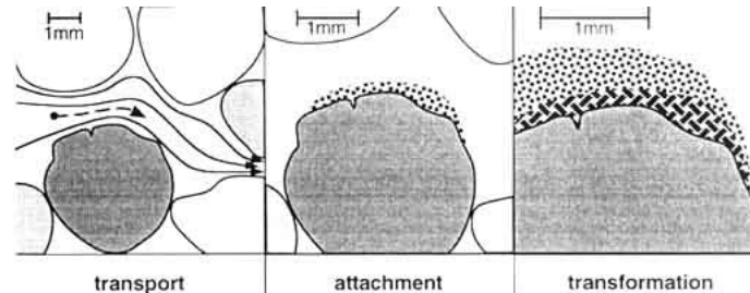
Fig. 26 Solid Separation Mechanisms in Roughing Filters
