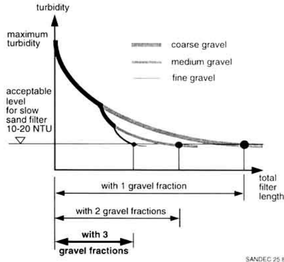
Fig. 31 Turbidity Reduction along a Roughing Filter
