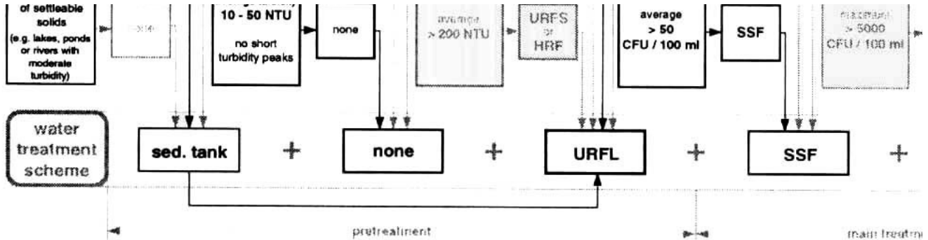
Fig. 57 Rehabilitation option for a Slow Sand Filter Plant
