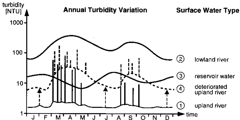
Fig. 53 Annual Turbidity Variation of Different Surface Water Sources
