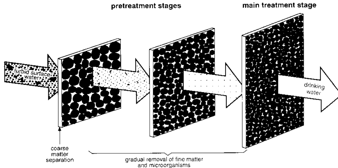
Fig. 3 Multiple Barrier Water Treatment Concept
