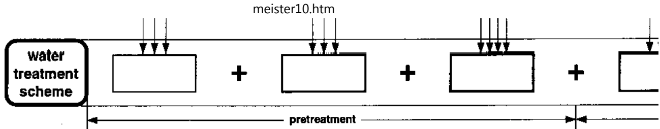
Fig. 43 Algorithm for the Design of Surface water Treatment Schemes Using Roughing and Slow Sand Filtration
