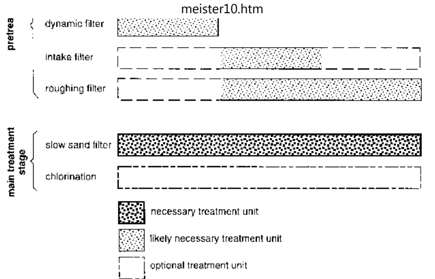
Fig. 17 Treatment of Surface Water
