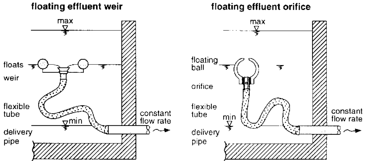
Fig. 33 Layout of Flow Rate Controlling Devices
