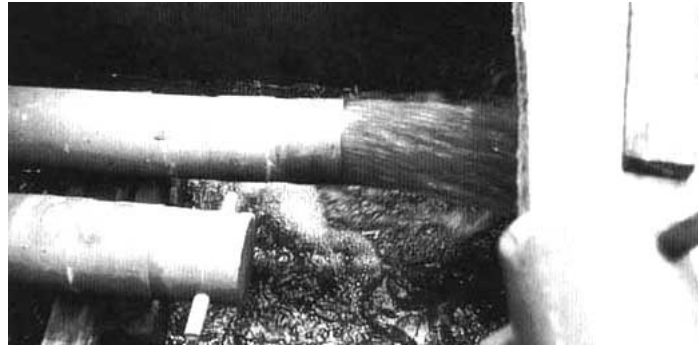
Photo 9 Hydraulic Cleaning of Roughing Filter (Note the Simple Design of the Fast Opening Device as also illustrated in Fig. 34, p. IX-9)
