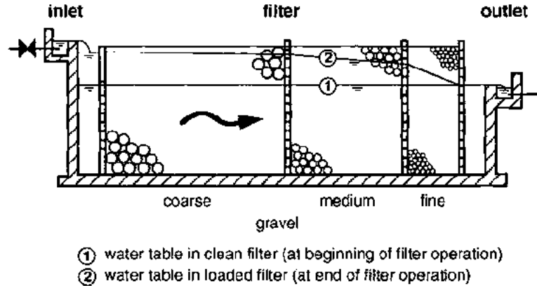
Fig. 32 Layout of an Inlet-Controlled Roughing Filter
