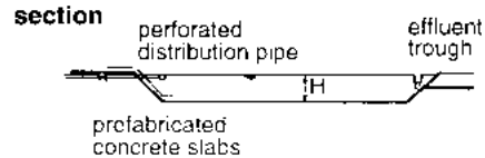
Fig. 18 Design of an Earth Basin as Sedimentation Tank
