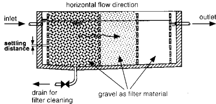
Fig. 8 Particle Removal in a Sedimentation Tank and a Roughing Filter
