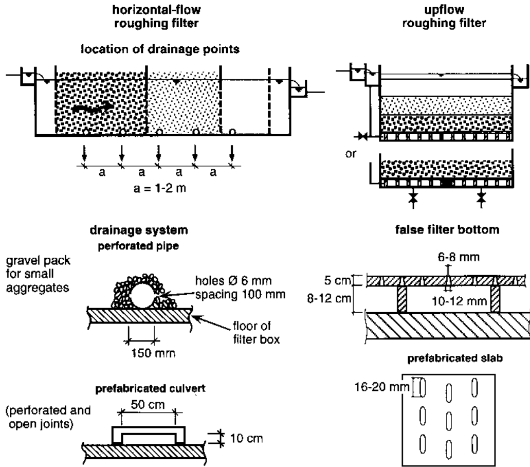
Fig. 47 Layout of Different Drainage Systems for Roughing Filters
