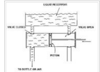
Figure 4: A piston filler
