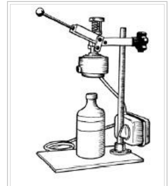
Figure 13: Capping Machine
