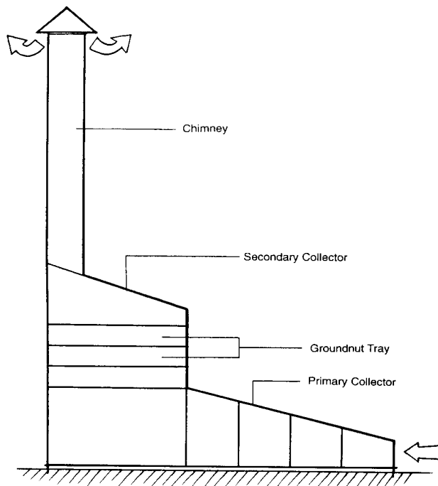
Figure 3: Indirect solar dryer
