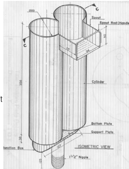
Figure 4: The piston design.
