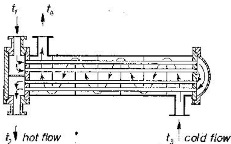
Fig. 8.2: Principal scheme of heat exchanger (mixed flow type)
