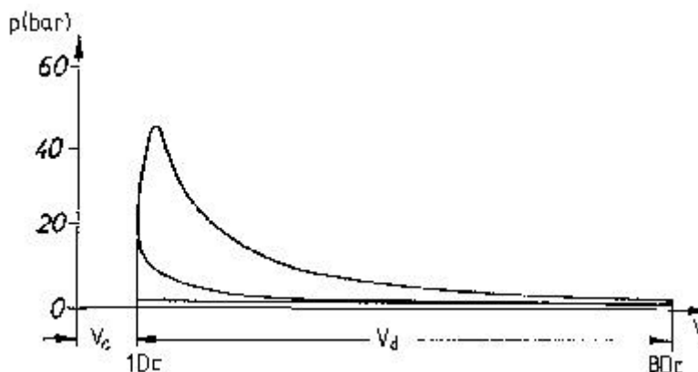
Fig. 3.14: Simplified p, v-digram of an Otto process
