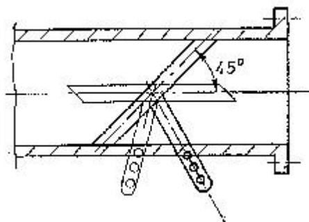
Fig.5.10: Butterfly gas control valve with elliptic butterfly for small angular movement (45°)
