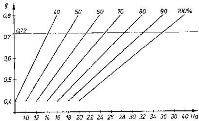
Fig. 4.2: Calorific value of biogas as a function of the density and volume %-age of its CH_4 content ( r = 0.72 is the density at a standard condition)
