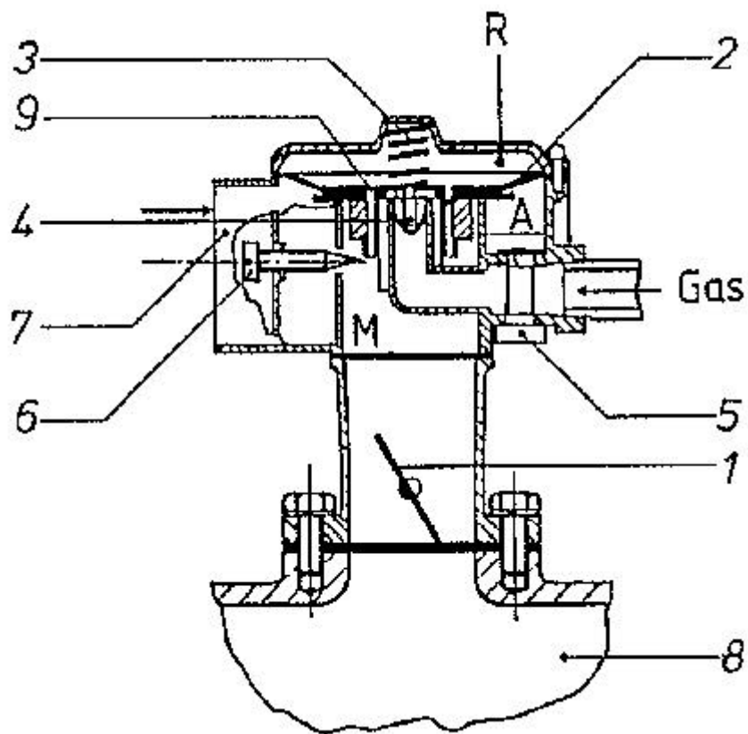
Fig. 6.6: Cross-sectional view of gas mixing valve.
