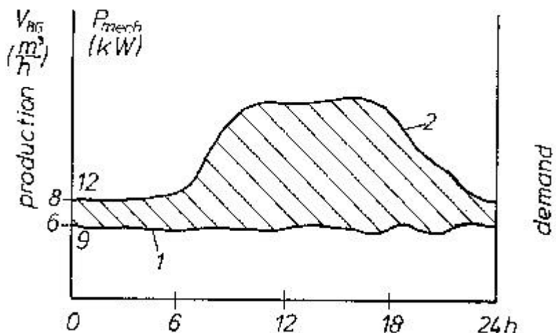
Fig 7.3: Daily profiles: 1 biogas and potential power production, 2 power demand, \\shortage in biogas/// power production. Power shortage to be compensated by other fuels/energies in isolated operation or by purchase of electric power from grid in parallel operation.
