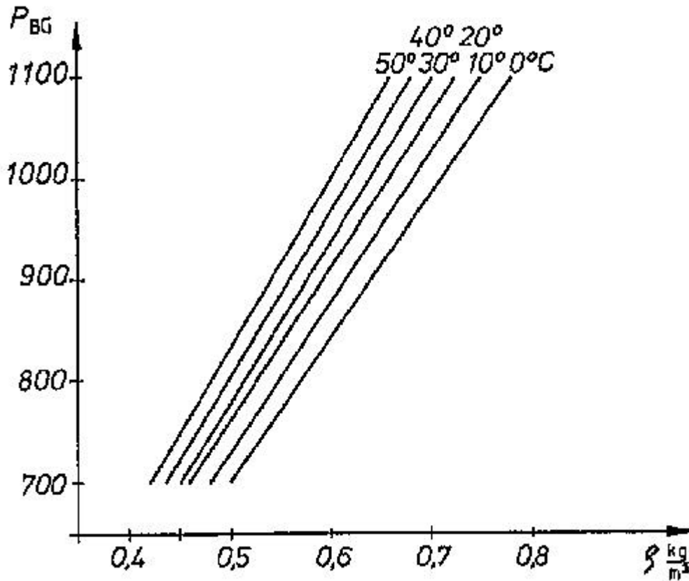
Fig. 4.1: Density r of CH_4 as a function of biogas pressure and temperature
