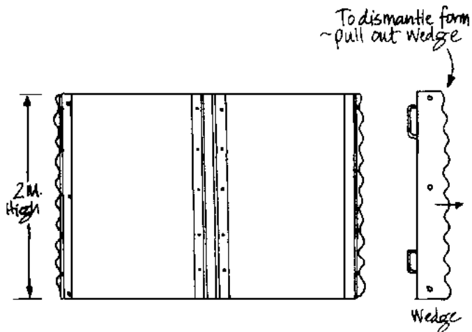
cross section of form Figure 18: Standard formwork for 10 cubic meter tank - cross section of form
