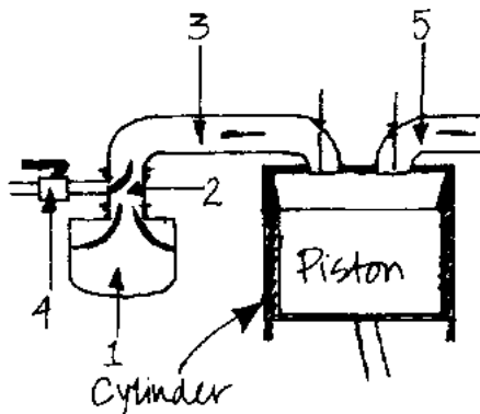
DIESEL ENGINE ADAPTED FOR BIOGAS
