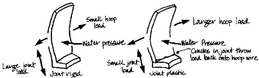
Figure 9: How the loads are taken
