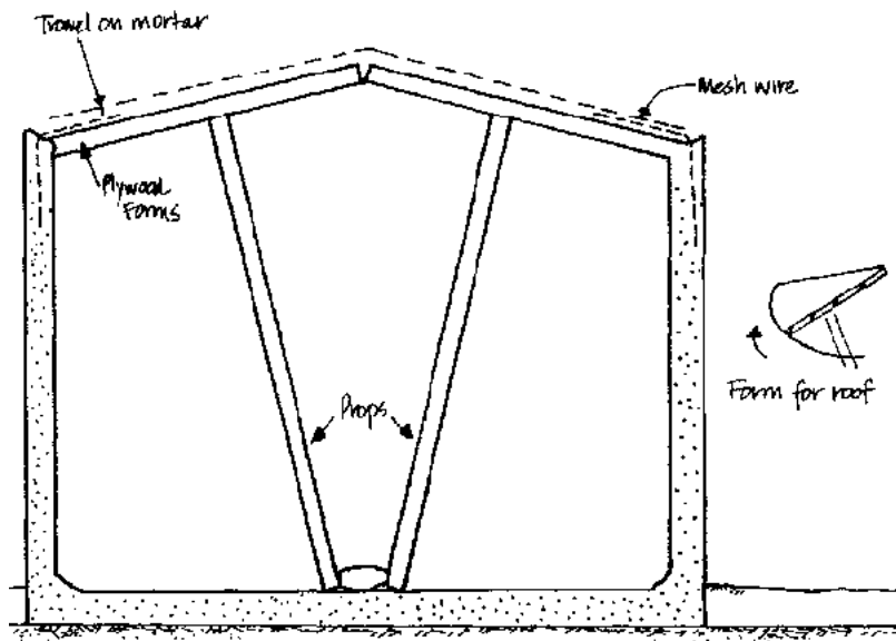
Figure 31: Constructing the roof
