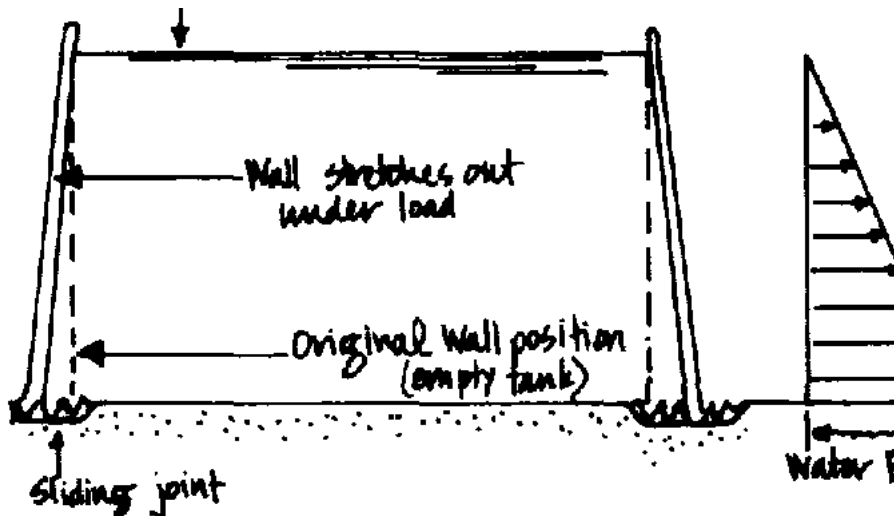
Figure 7: WALLS FREE TO MOVE
