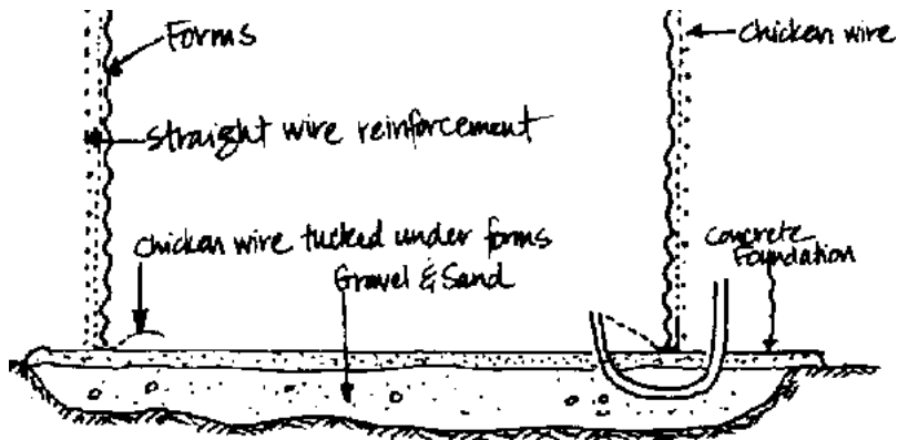
Figure 21: Erecting formwork and winding on reinforcing wire
