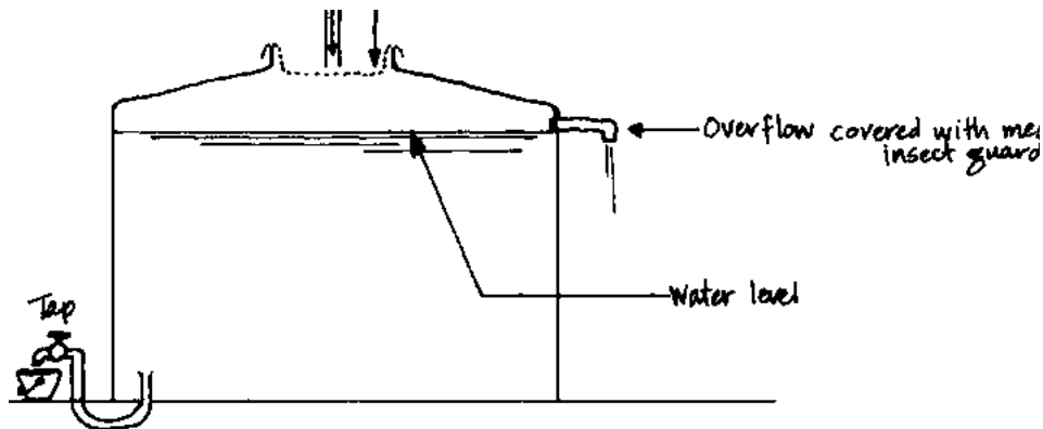
Figure 2: Protecting the tank from further contamination
