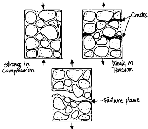
Figure 3: MORTAR UNDER LOAD
