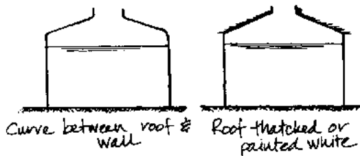
Figure 11: Roofs for tanks less than 5m diameter
