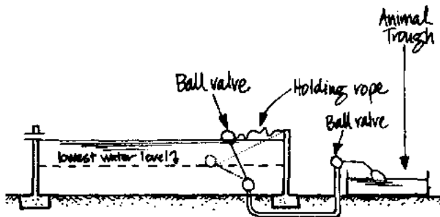
Figure 13: Ball valves for cattle watering
