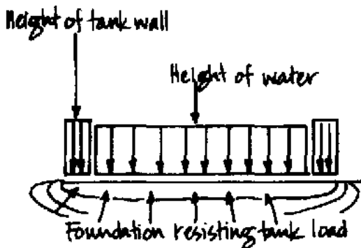
Figure 6B: Walls and floor separate
