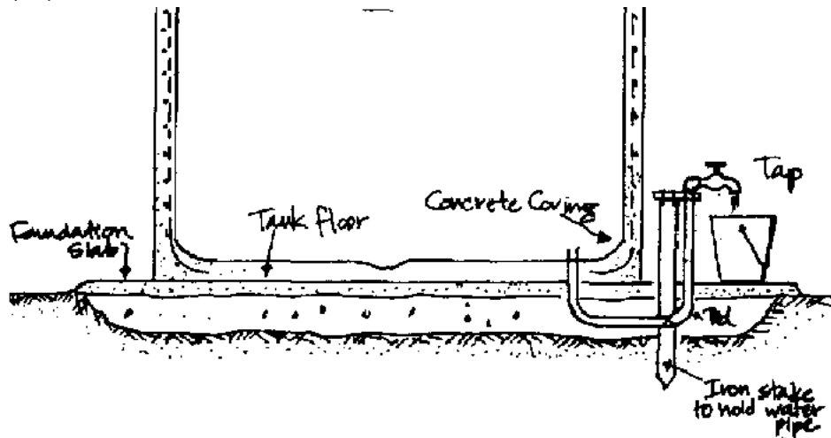
Figure 22: The completed tank
