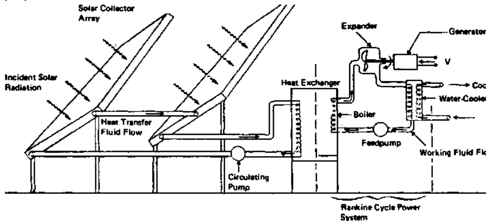
Solar-powered electric power plant. (Courtesy Arthur D. Little, Jr) SOLAR COLLECTOR AND RANKINE ENGINE
