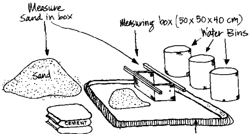
Figure 15: Mixing the concrete by hand
