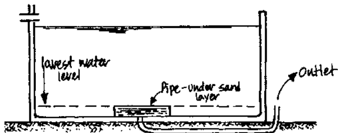
Figure 14: Slow sand filter in tank over outlet
