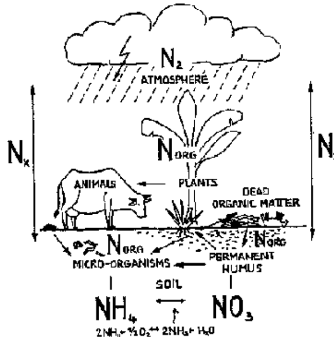
Fig. 33.: The nitrogen-cycle in nature
