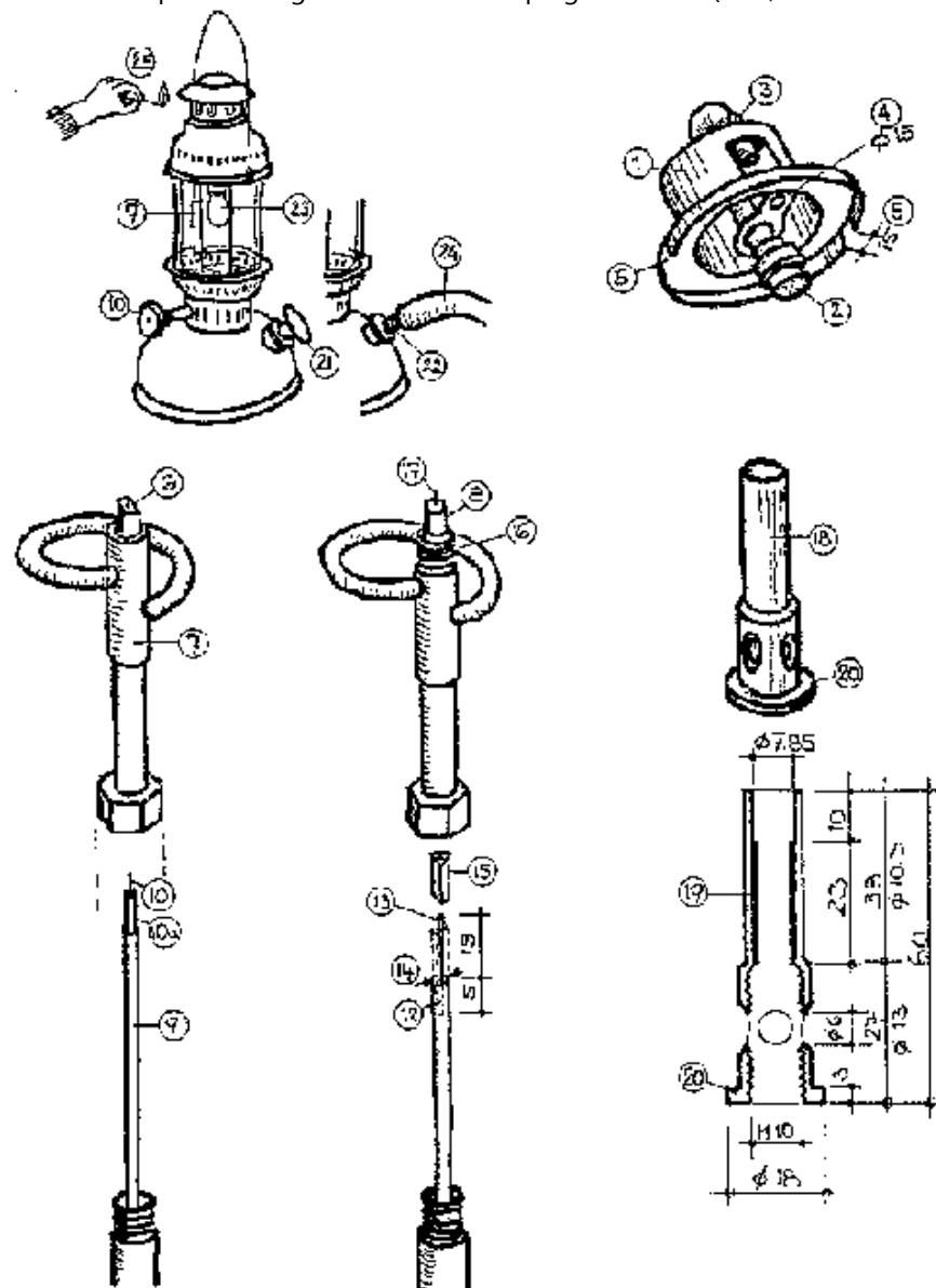
Fig. 39: Modification of pressure lamps
