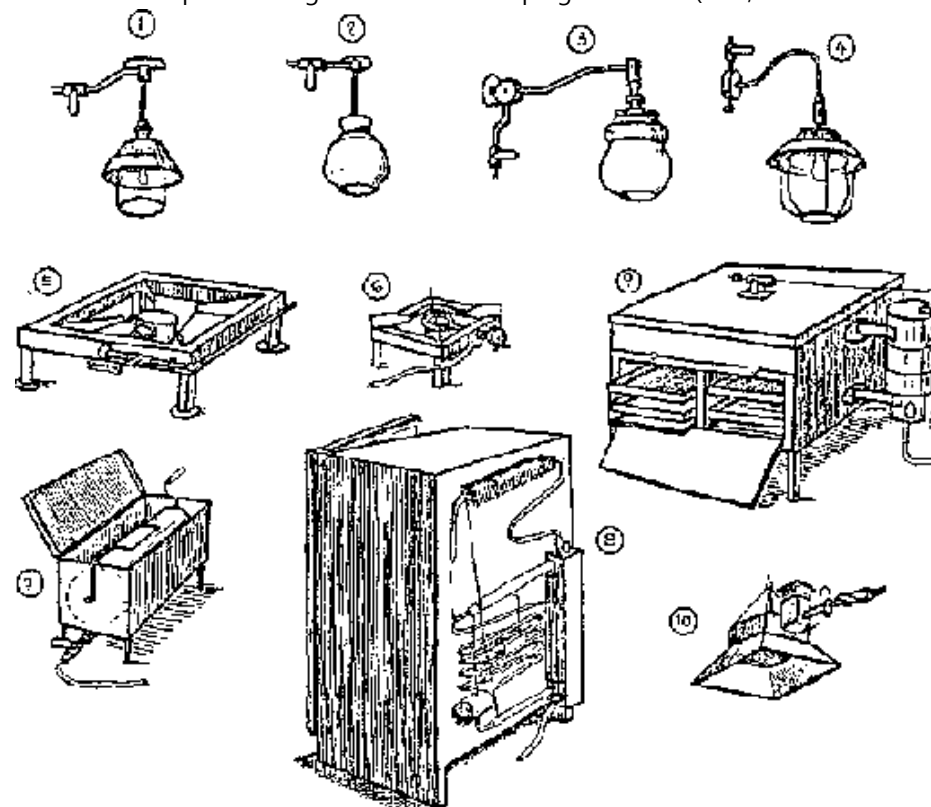
Fig. 38: Biogas appliances
