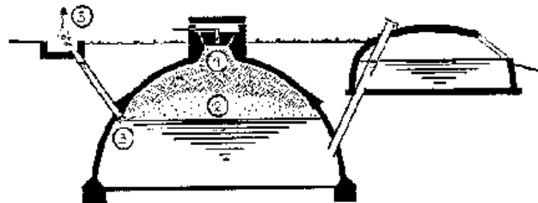
Fig. 41: Scum formation in a fixed dome plant
