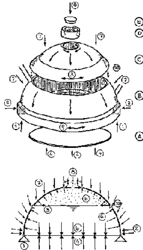
Fig. 14: Principle of statics of fixed dome plant
