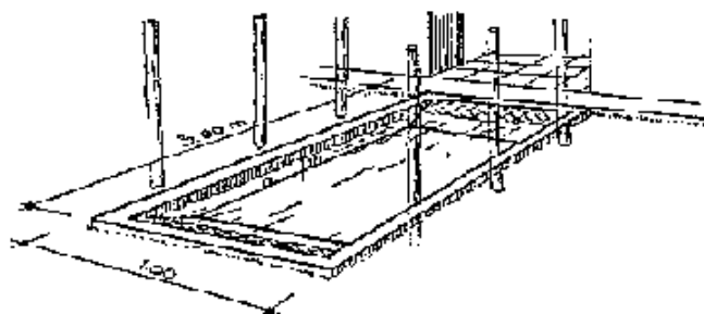
Fig. 30: Cattle foot bath. If cattle are regularly out grazing, they should pass a cleaning foot bath before entering the stable in order to prevent too much soil from entering the gasplant. A drainage pipe would allow easier cleaning.
