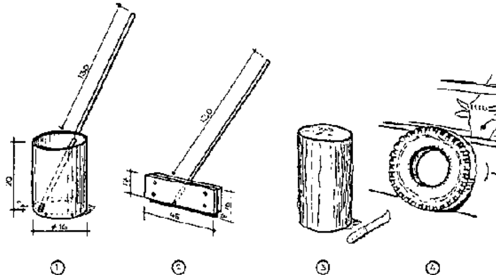
Fig. 12: Necessary equipment to operate a biogas unit
