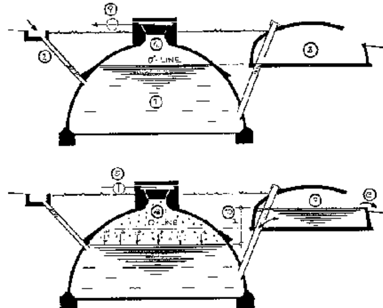
Fig. 6: System of the fixed dome plant
