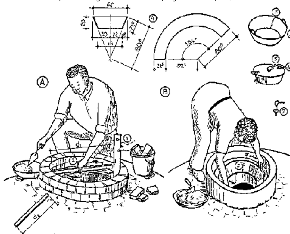
Fig. 22: Construction of neck and lid
