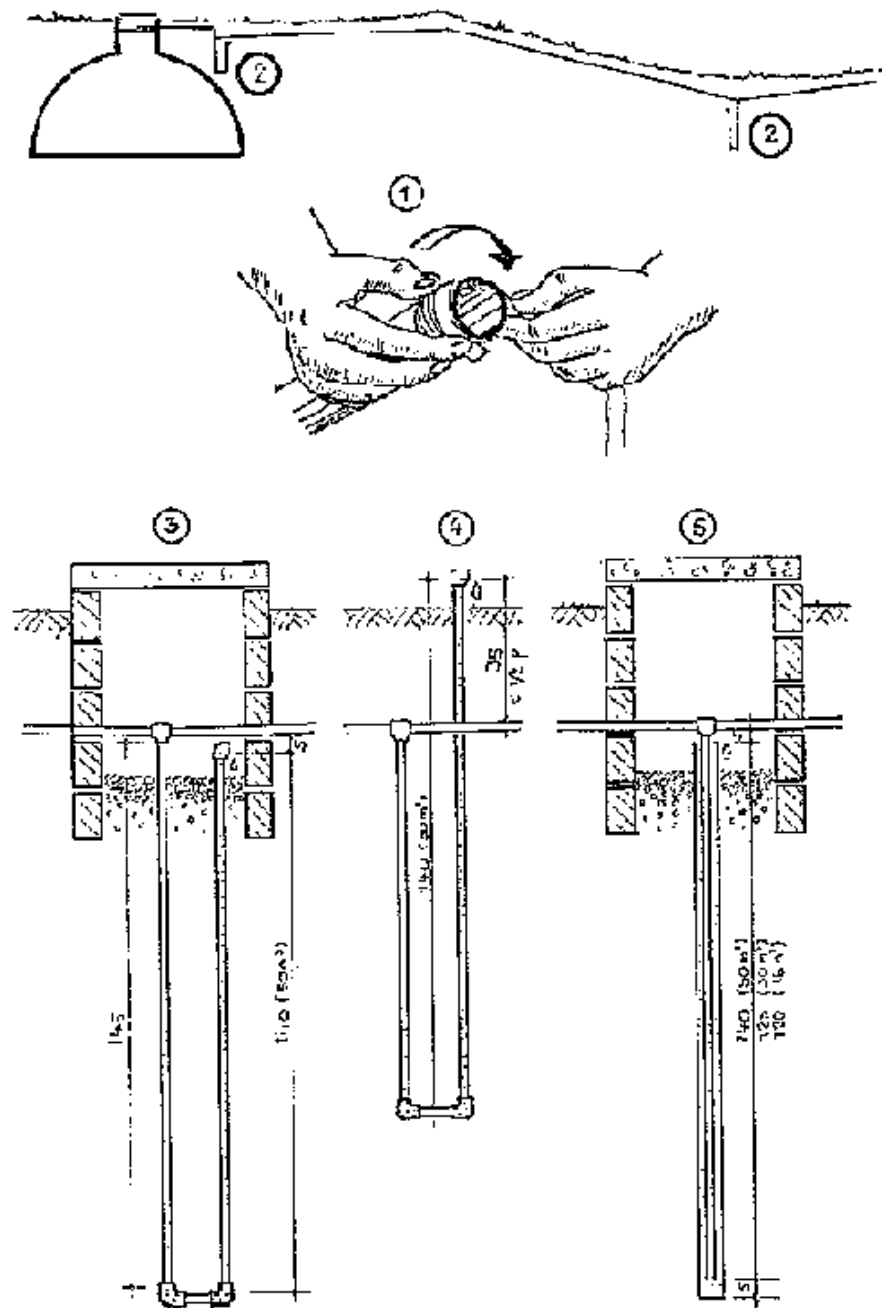
Fig. 26: Installation of gas pipe
