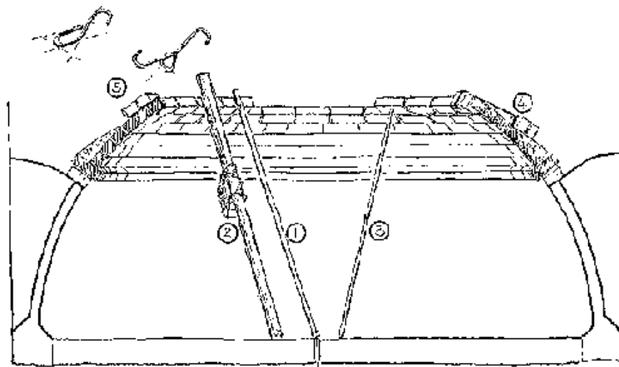
Fig. 19: Temporary support of brickwork
