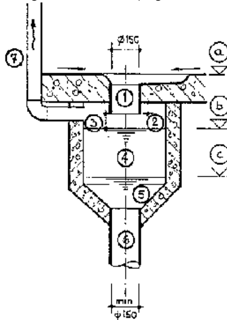
Fig. 32: Construction details of toilets
