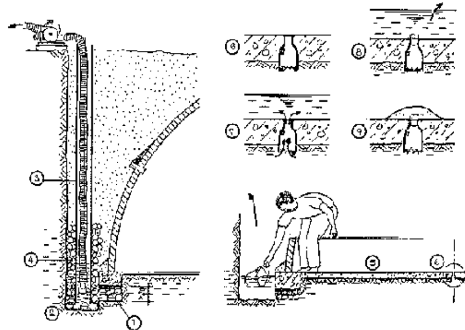
Fig. 24: Construction below the ground water table
