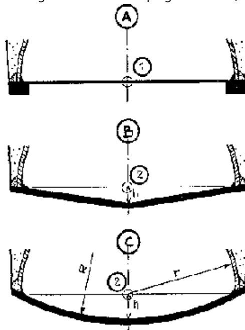
Fig. 25: Shape of the digester bottom slab
