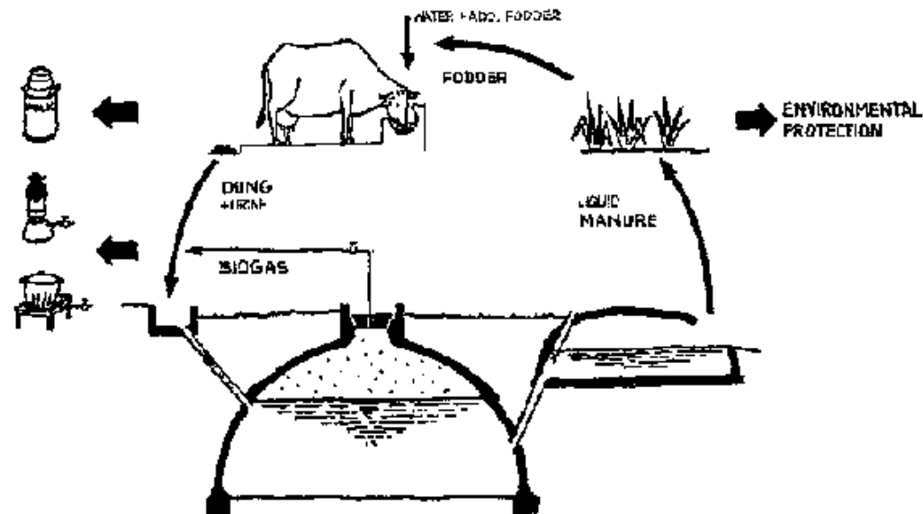
Fig. 1: The cycle of organic matter and the benefits of an agricultural biogas unit The animals provide dung to the biogas plant, the gasplant provides manure to the fodder plantation and the plantation provides feed to the animals. If enough water is given to the animals, no additional water is required for the biogas plant.
