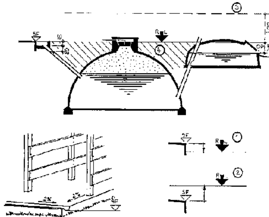
Fig. 15: The reference line
