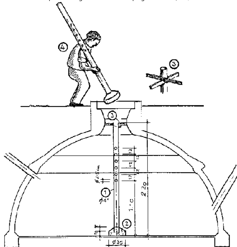
Fig. 42: Stand-pipe for gas release
