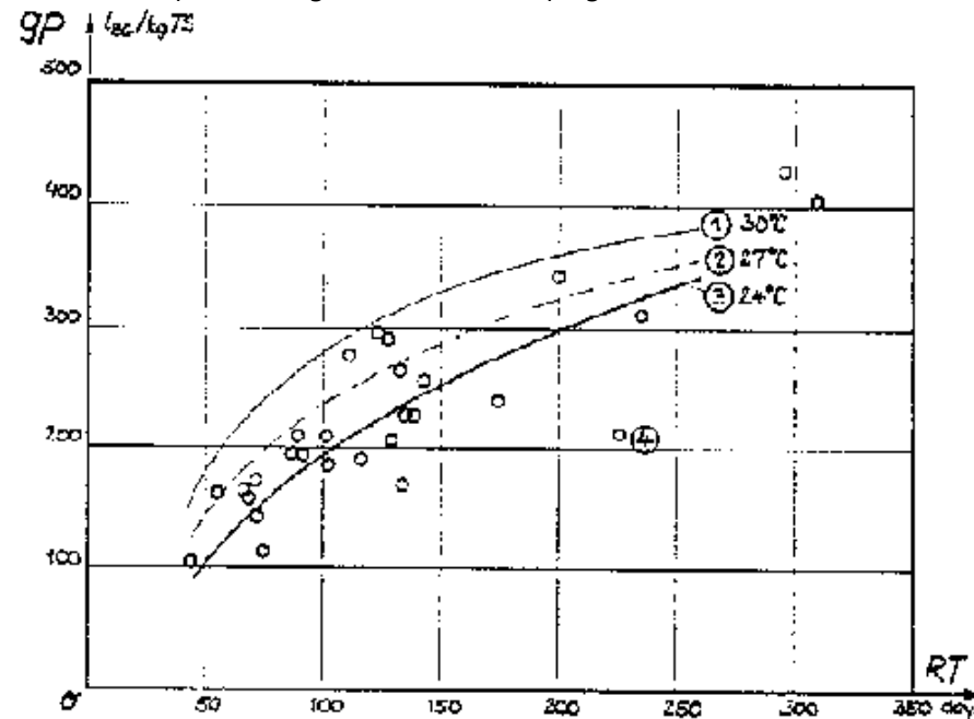
Fig. 4: Relation of gas production and retention time
