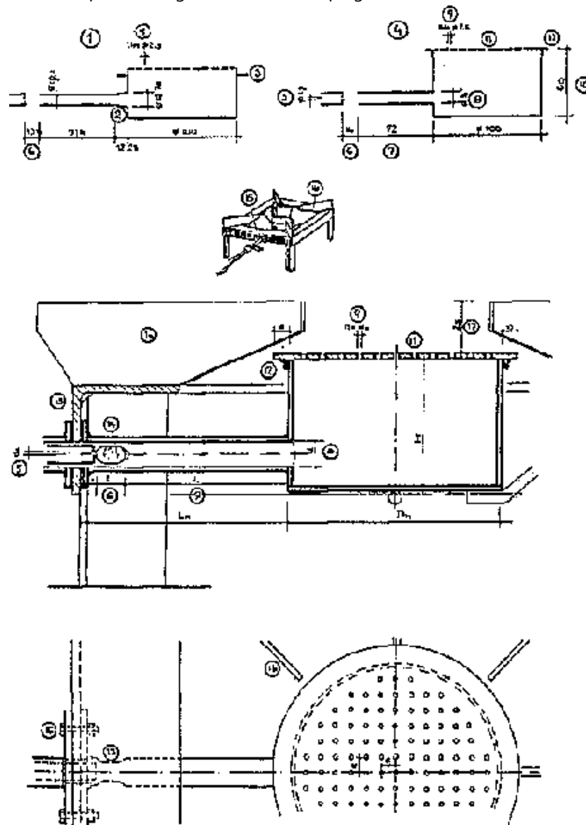
Fig. 37: Gas stoves
