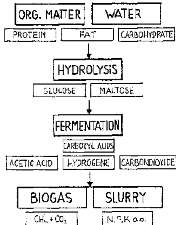
Fig. 2: The big-chemical process of anaerobic digestion The different groups of bacteria responsible for fermentation live in an interacting eco-system. Each type of bacteria depends on others. The fermentation time is shortest when populations of different bacteria are adequately balanced.
