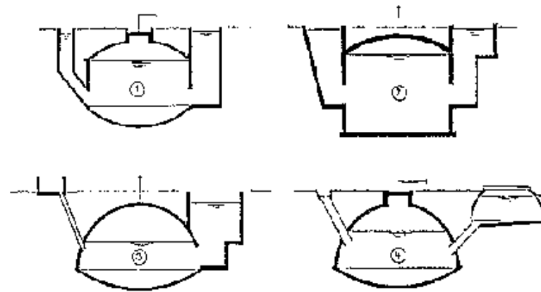
Fig. 7: Different models of fixed dome plants Fixed dome plants originate from China and were built already before 1960. Several variations with or without a removable cover at the top have been developed. (1) Biogas plant from Chengdu/China; (2) Janata Plant from India; (3) Dheenbandhu Plant of AFPRO from India; (4) Modified BORDA plant from Cankuso in Burundi..
