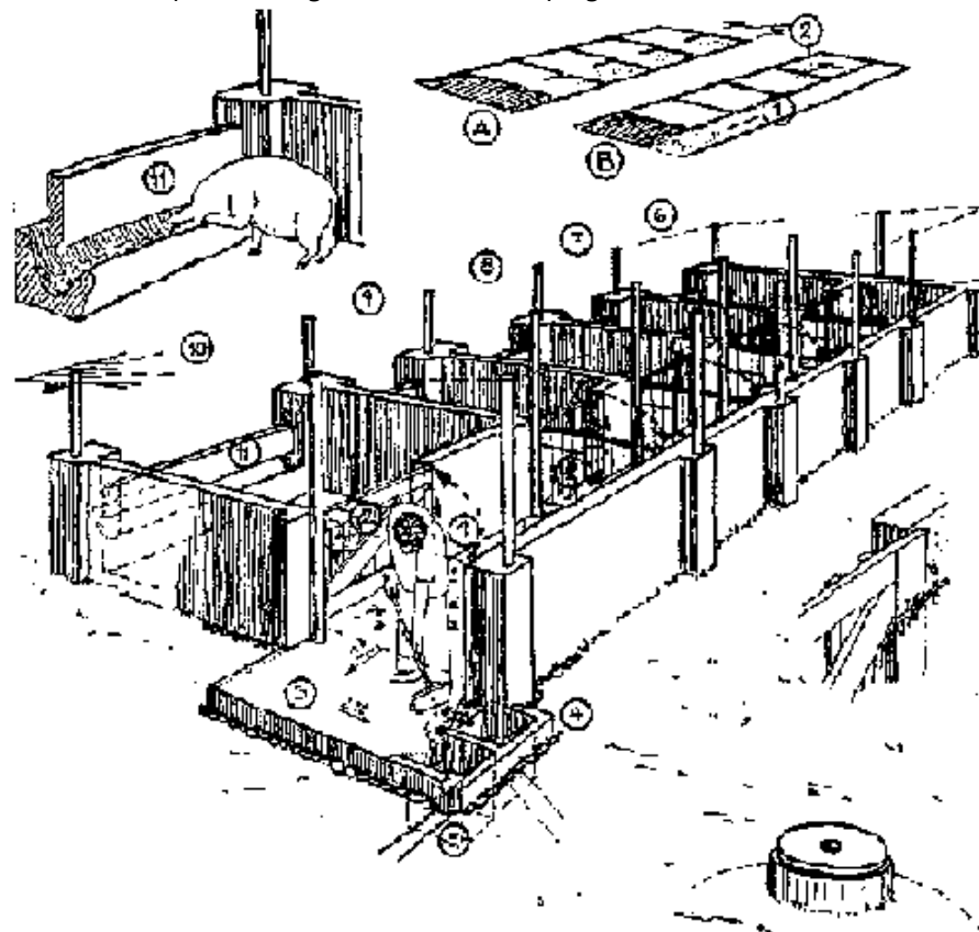
Fig. 31: Principle design of the pigsty
