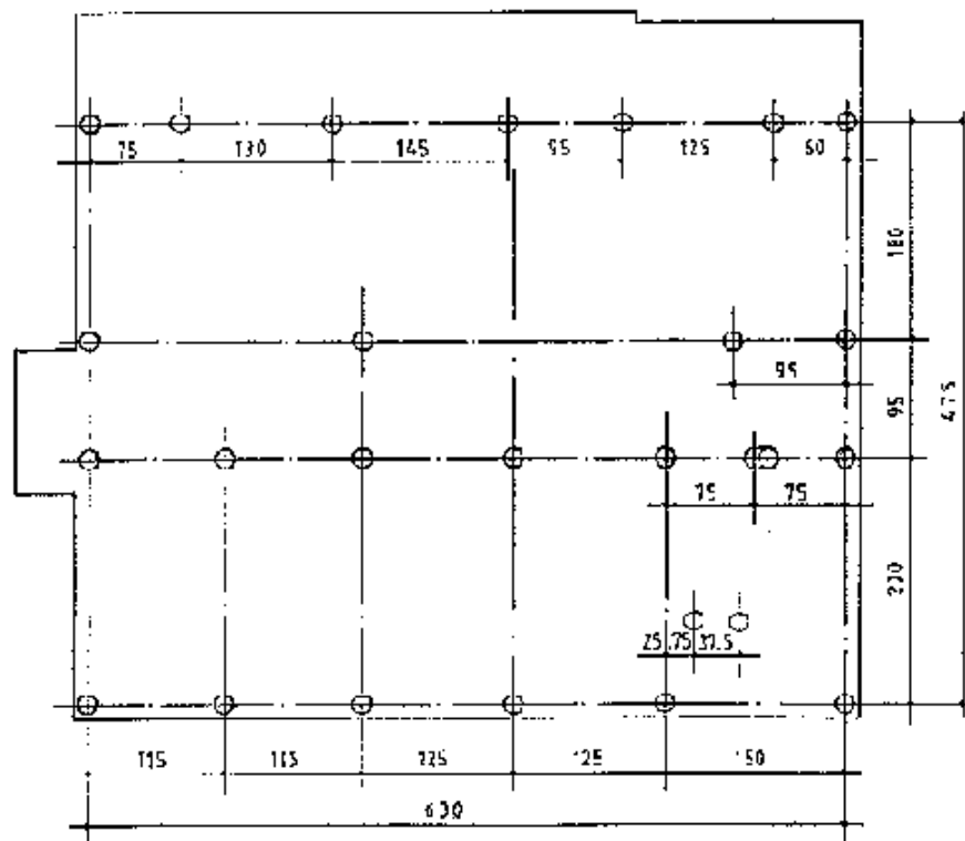
Foundation plan
