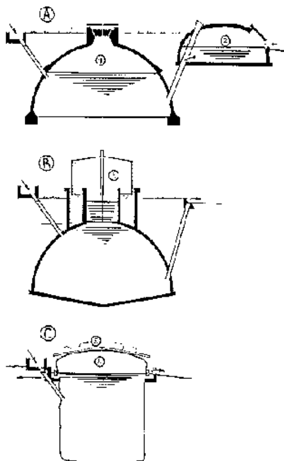
Fig. 5: Small-scale biogas plants for rural areas in tropical countries
