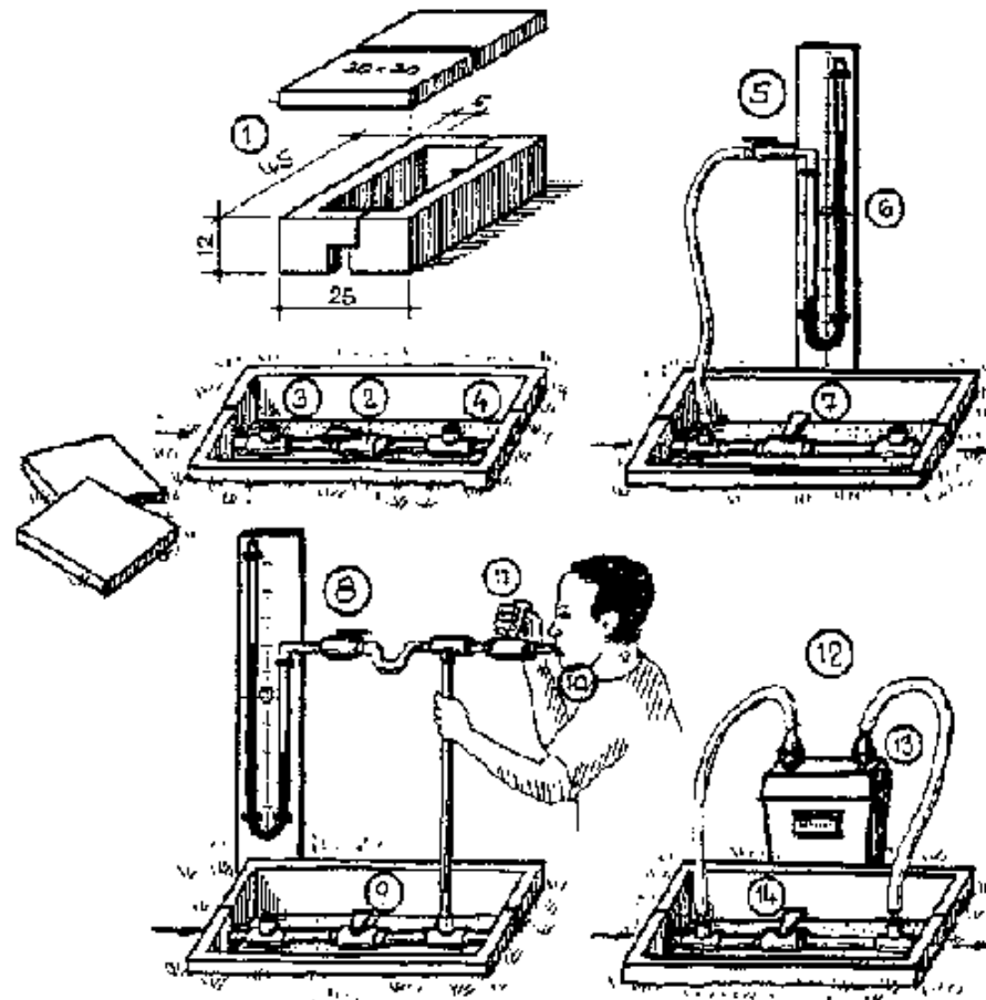
Fig. 27: The test-unit
