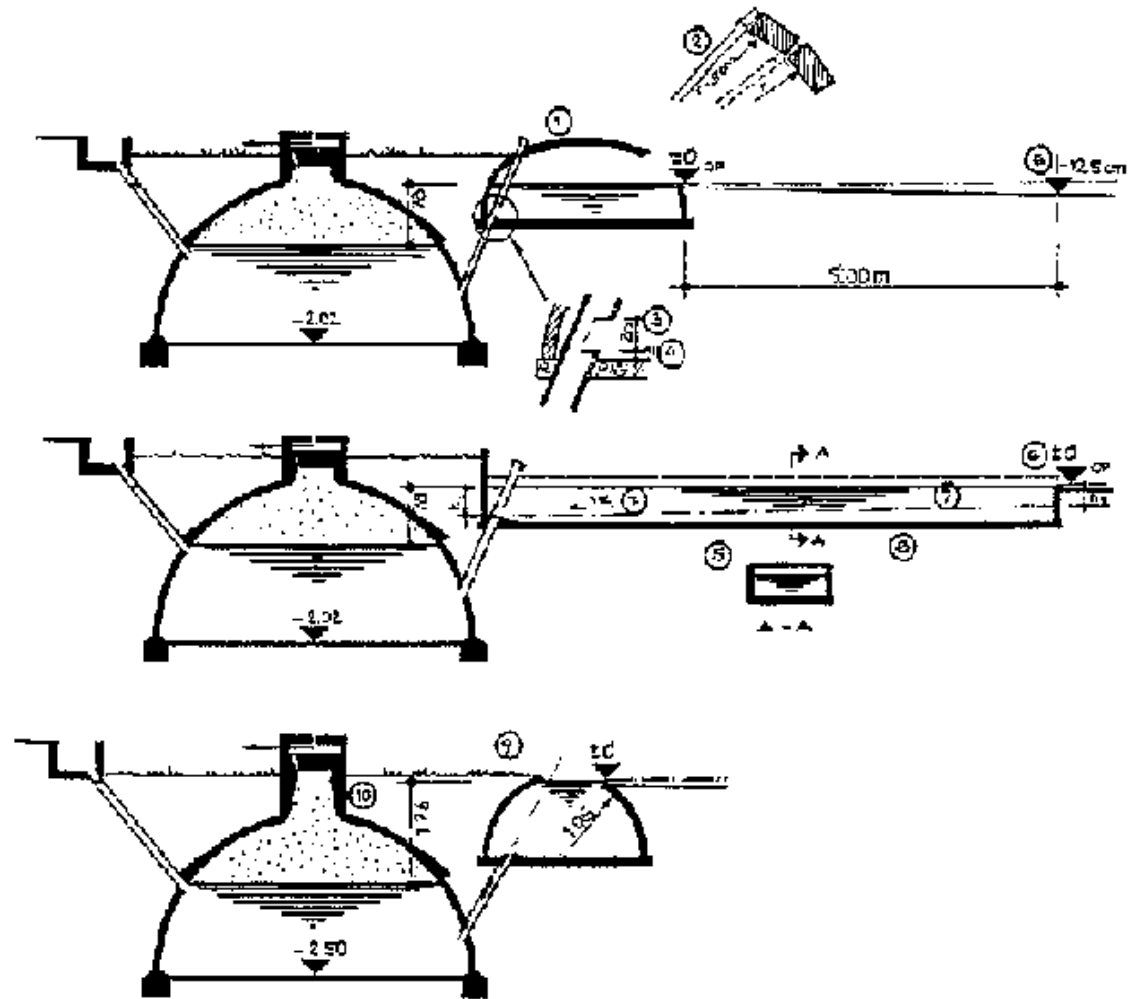
Fig. 21: The expansion chamber
