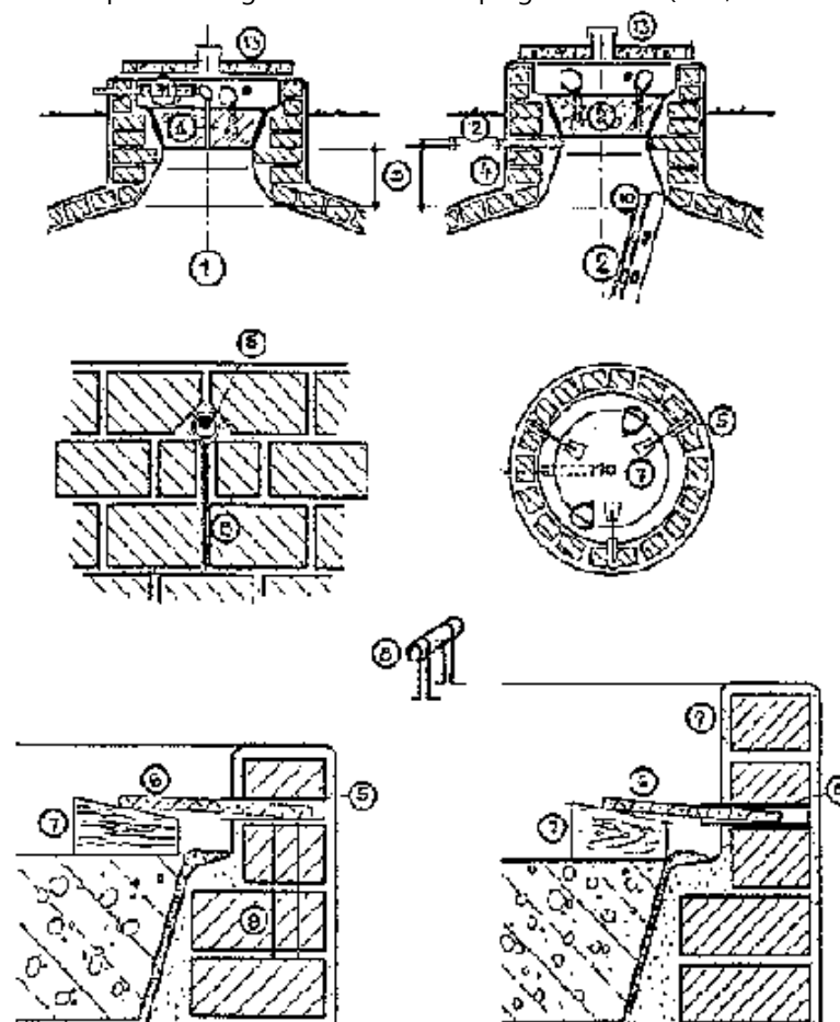
Fig. 23: Details of the neck and the lid
