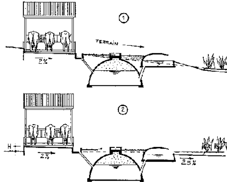
Fig. 13: Position of gasplant to stable floor The ideal situation is a sloping ground, falling from the stable via the gasplant to the crop plantation (1). On horizontal ground (2), it might be necessary to lift the floor of the stable (H).
