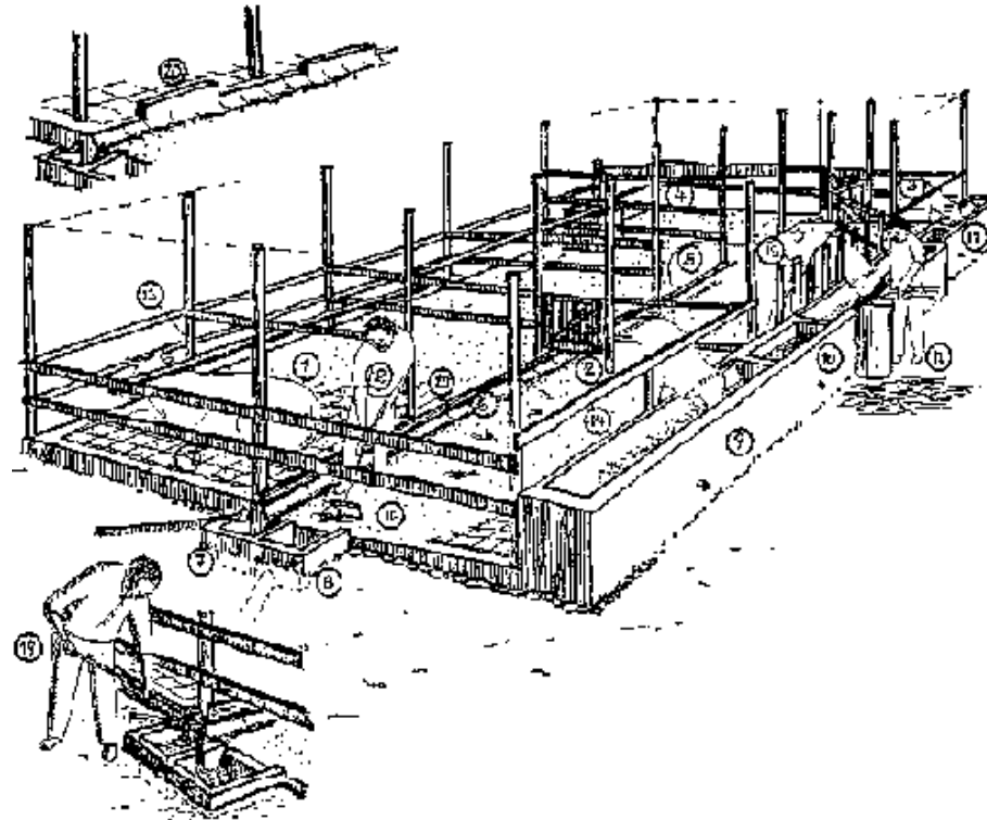
Fig. 29: Principle design of the cattle shed.
