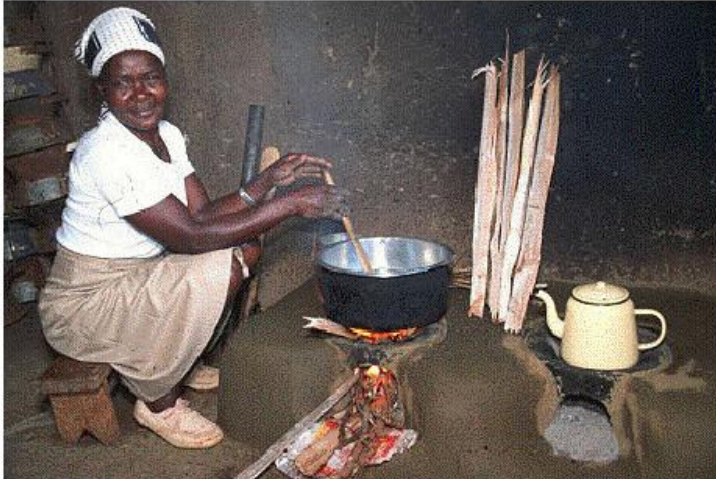
Figure 1: Improved Cookstove in Kenya Neil Cooper/ITDG
