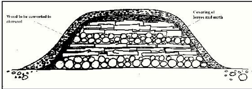
Figure 3: Traditional Earth Kiln for Charcoal Production
