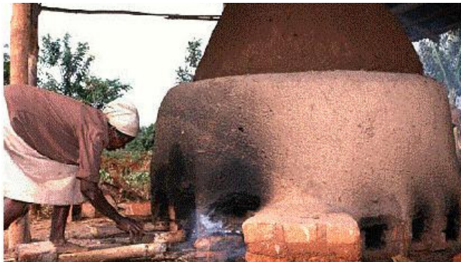
Figure 4: Charcoal Kiln, Kenya Heinz Muller/ITDG
