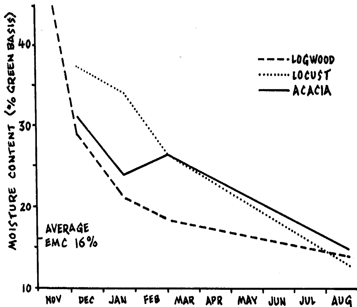
Figure 1. Drying Curves for Montserratian Fuelwood/Charcoal Species
