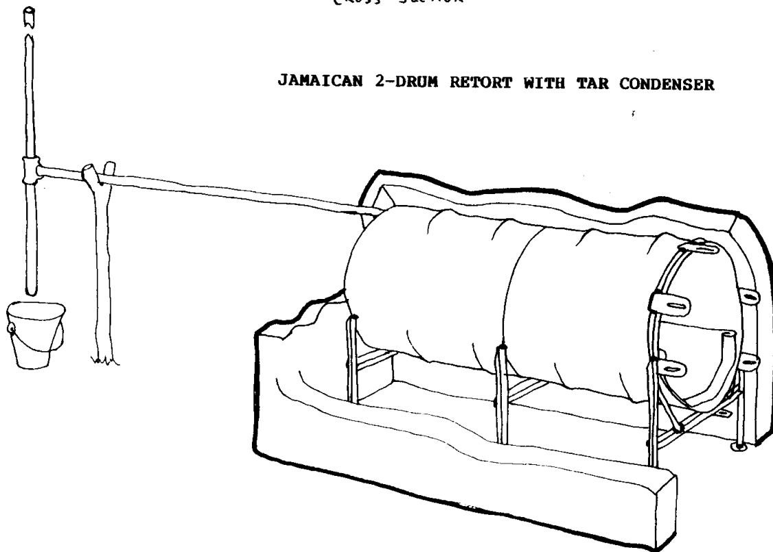
JAMAICAN 2-DRUM RETORT WITH GAS PORTS
