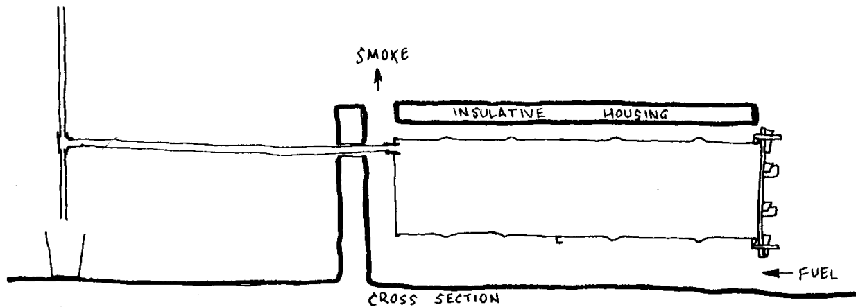
JAMAICAN 2-DRUM RETORT WITH TAR CONDENSER
