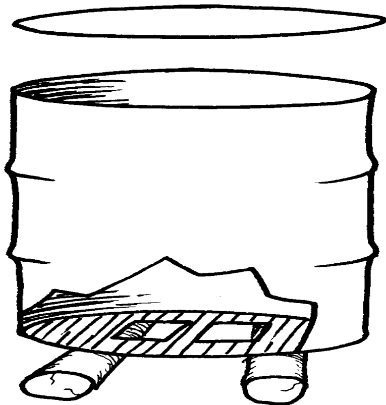
COSTA RICAN KILN
