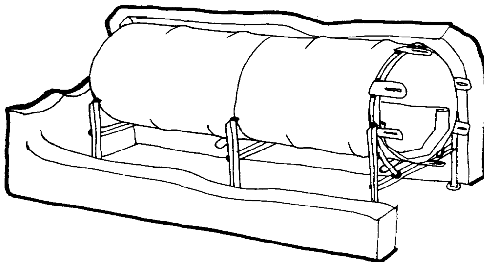
JAMAICAN 2-DRUM RETORT WITH GAS PORTS
