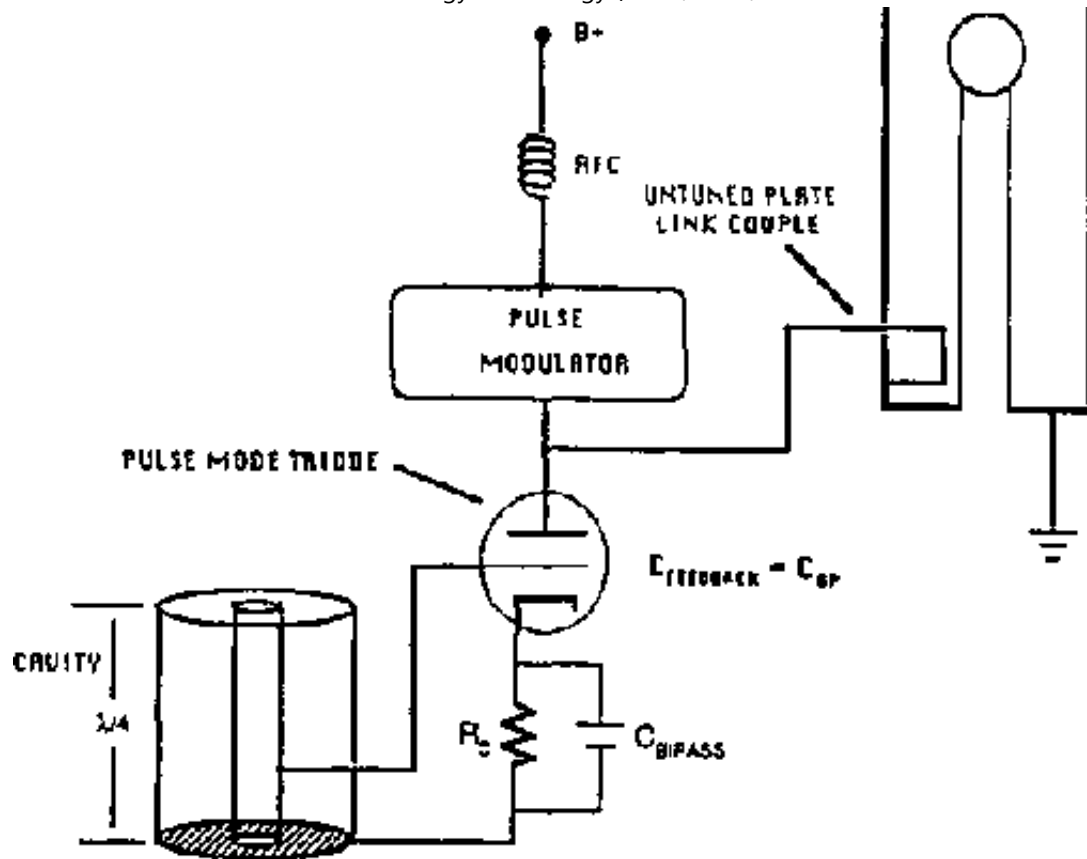
Figure 7: The optimal vacuum tube source configuration utilizing a tuned grid plate pulse modulated
