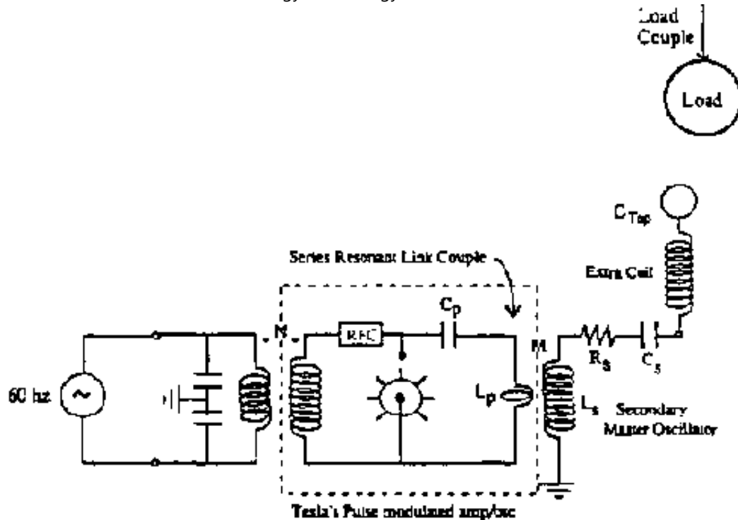
Figure 6: (a) Block diagram of typical RF power processing system (b) Tesla's 1899 Colorado Springs apparatus system equivalent. (3)
