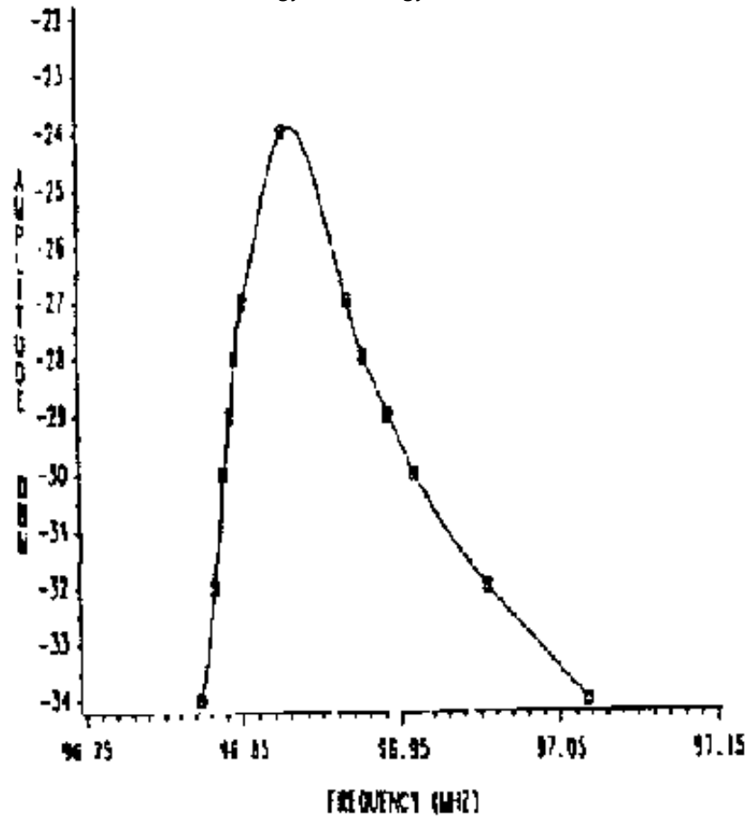
Figure 9. Response of cavity 1 ( b/a = 3.4 )
