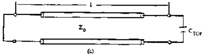
Figure 5. The quarter wavelength capacitively loaded
