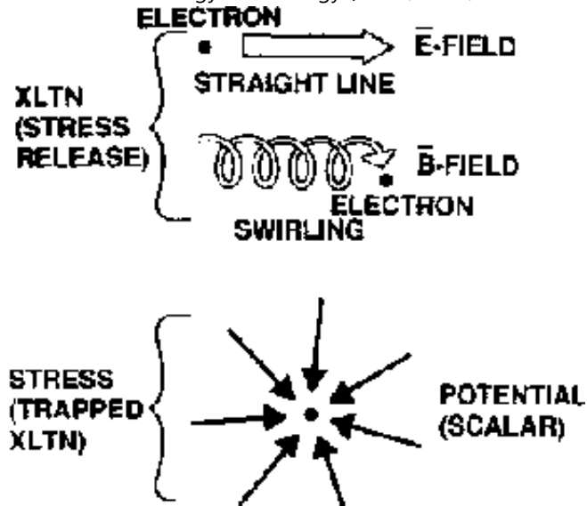
Figure 4. Electrogravitational fields E, B. and G
