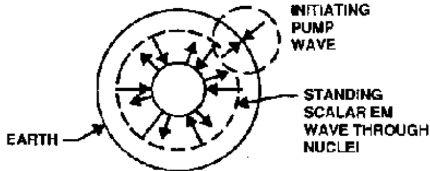
Figure 3. Spherical scalar wave in internal earth stresses
