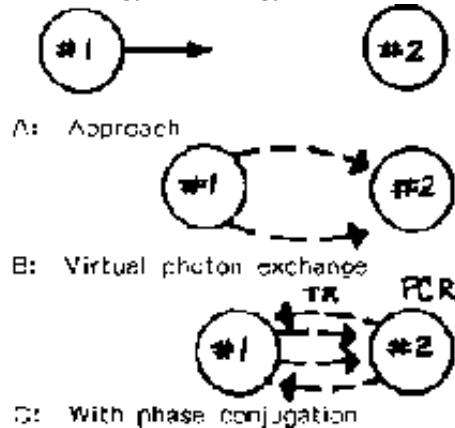
Figure 5. Newton's Third Law
