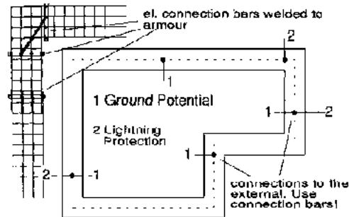
Fig 14 Using the reinforcement steel matt as earth contact.
