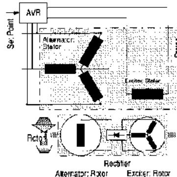
Fig 1 Principle diagram of a synchronous generator.
