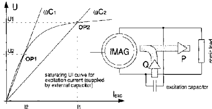
Fig 5 UI curve for the saturating excitation current and U_1 lines for two different capacitors at constant frequency. The resulting two stable operating points (OPT and OP2) are reached at very different output voltages U_1 and U_2 . The circuit besides shows the pow of power. The required magnetization power (reactive Q ) is supplied by the excitation capacitor.
