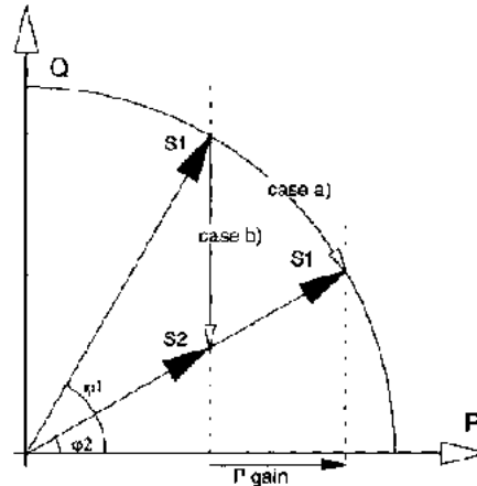
Fig 8 A geometrical interpretation of the influence of a power factor reduction ( j_1 , to j_2 ) on the power (P, Q & S) in a load. a) S constant: 'move on the circle'->in creases P, decreases Q b) P constant: 'move straight down' >decreases S and Q
