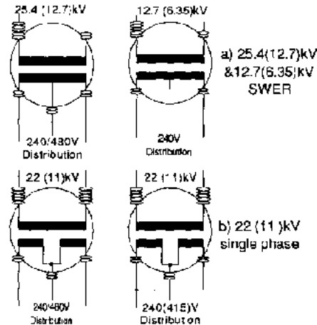
Fig 4 Dual Voltage Transformers.
