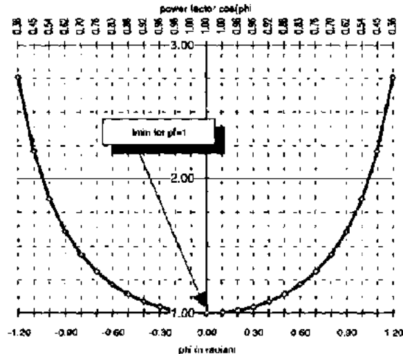
Fig 5 Ratio apparent to active current as a function of the power factor.
