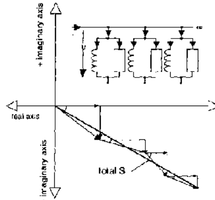
Fig 4 Phasor diagram to determine S in a parallel circuit of several inductances and resistors.
