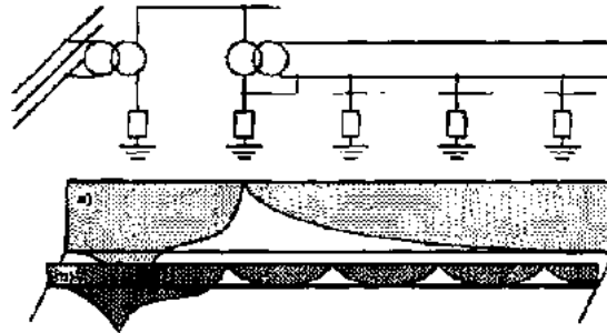
Fig 6 Improvement of the earth potential using several earthing systems. a) 'steep' and 'deep' potential funnel for a single earth at the transformers . b) the obvious betterment using
