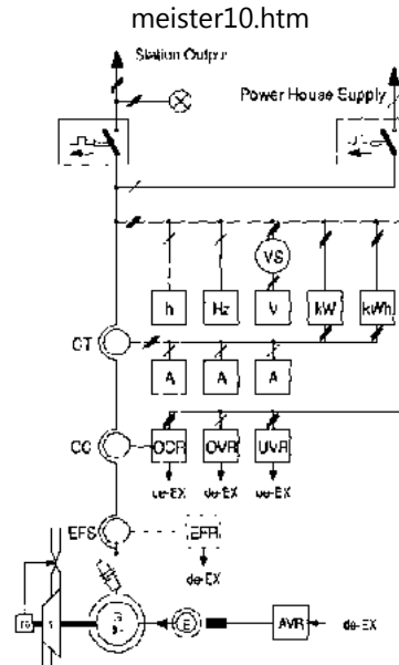
Fig 3 Single line diagram for the control circuit of category B. The earth fault relay is optional.
