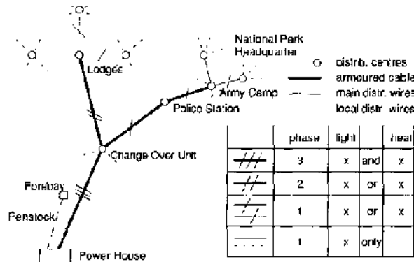
Figure 1 Schematic transmission and distribution system.
