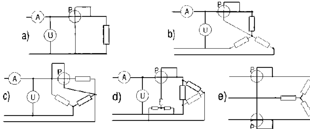
Fig 9 Measuring the power factor. a) single phase circuit b) circuit to measure a 'star' load c) circuit to measure a 'delta' load d) external star point circuit to measure a 'delta' load e) Aron circuit, which uses only two power meters to measure the total P in an unbalanced three phase system.
