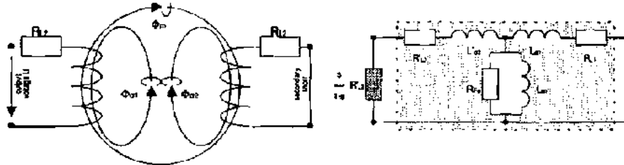
Fig 4 A simplified physical representation of a transformer. is the magnetic flux separated in a coupling component (index m) and two stray components (index a). This flux is modelled in a lumped circuit as inductance. Resistive losses are indicated as resistors (index L for coils, index Fe for iron)
