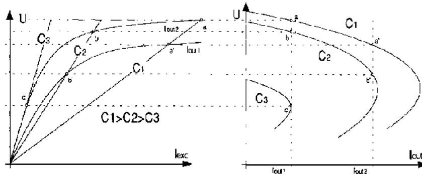
Fig 6 Relations of UI curves for varying excitation currents at constant I_{0,} and the corresponding UI curves for the output currents at constant C . For a constant capacitor value the voltage varies with the output current along the C -lines (a-a', b-b'). the point c indicates that for C_3 the maximum output current is reached. All curves at constant frequency.
