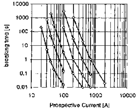
Fig 1 Time/current characteristic for fuses - a sample
