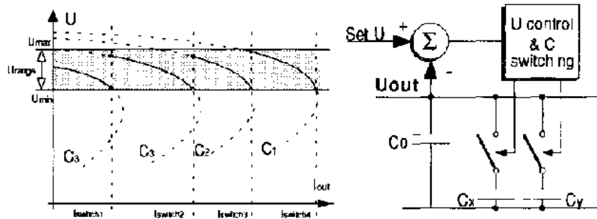
Fig 10 Switching between four combinations of excitation capacitor values to reduce the voltage swing.
