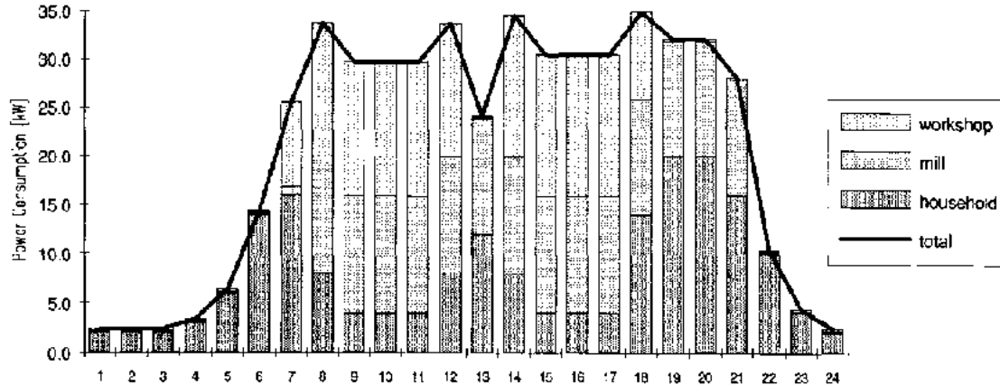
Fig 2 Example: hypothetical load curve during one day (24 hours)
