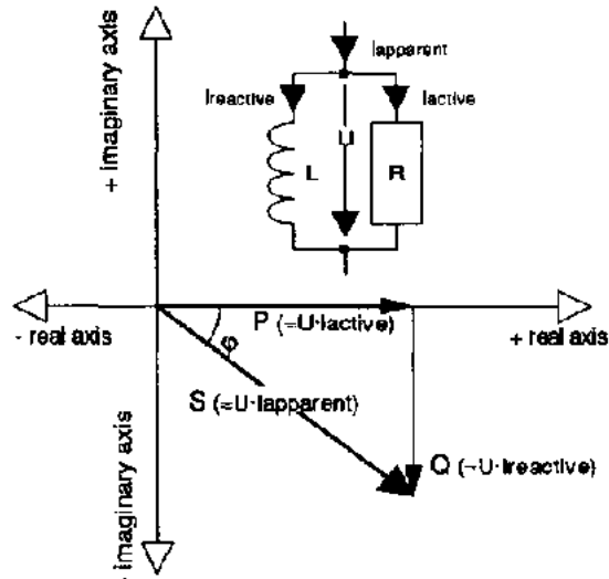
Fig 3 Phasor diagram for the electrical power in a parallel circuit (inductance II resistor).
