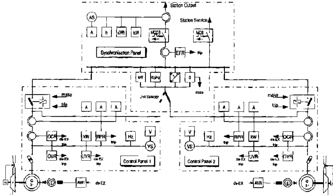
Fig 4 single line diagram for the control circuit of category C. Control panel I and 2 are identical.
