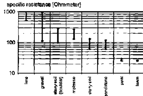
Fig 7 Specific resistance for different types of soil.
