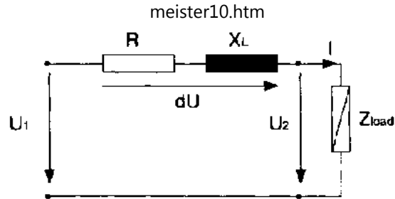
Fig. 4 Simplified equivalent circuit of overhead lines up to 60 kV
