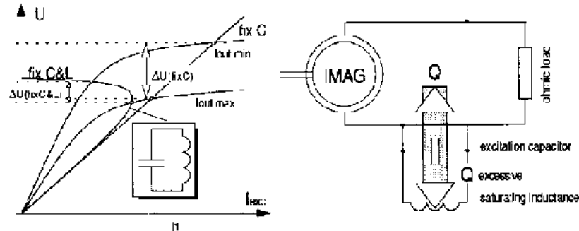
Fig 8 Reduce the output voltage swing by adding a saturating inductance.
