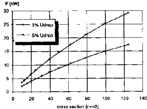
Fig 4 Cross section A as a function of P for 380V and 500m line length
