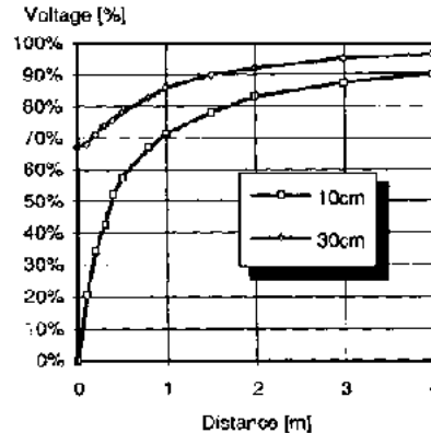
Fig 13 Resistance (voltage) distribution at the surface in case of a vertically dug-in plate t5(500/500mm) at two different depths.
