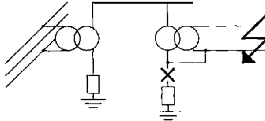
Fig 7 Risk of high tension on the LV distribution.
