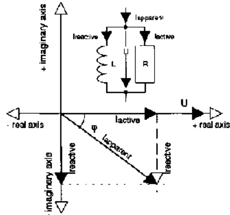
Fig 2 Phasor diagram for currents and voltage in a parallel circuit (inductance II resistor).
