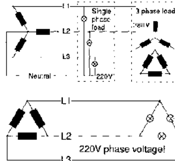
Fig 1 Three and four wire system
