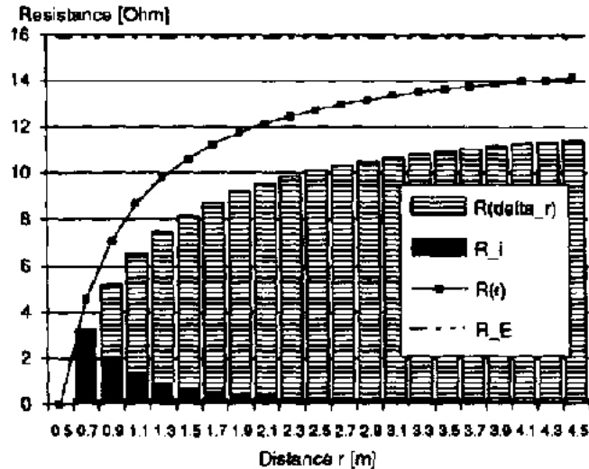
Fig 3 The development of the earth resistance R_E W with growing distance from the center of a metal sphere of 0.5m diameter. ( d = 100 Wm). It shows a) the decreasing resistance of 20cm thick 'soil shells' (see fig1 and 2), b) the stabilizing earth resistance, c) the exact calculation and d) the value at infinity.
