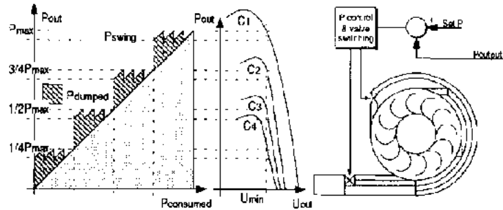
Fig 13 Reduce power loss by varying P_{mech} , and combine it with a load controller.
