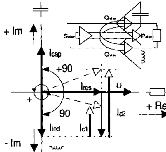
Fig 6 Compensating an inductive with a capacitive current.
