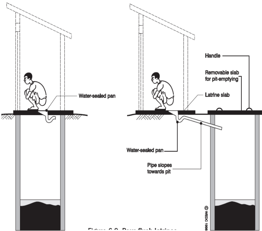
Figure 4: A pour-flush latrine set over a pit latrine (left) and discharging to an offset pit (right) (Source: Harvey et al, 2002)
