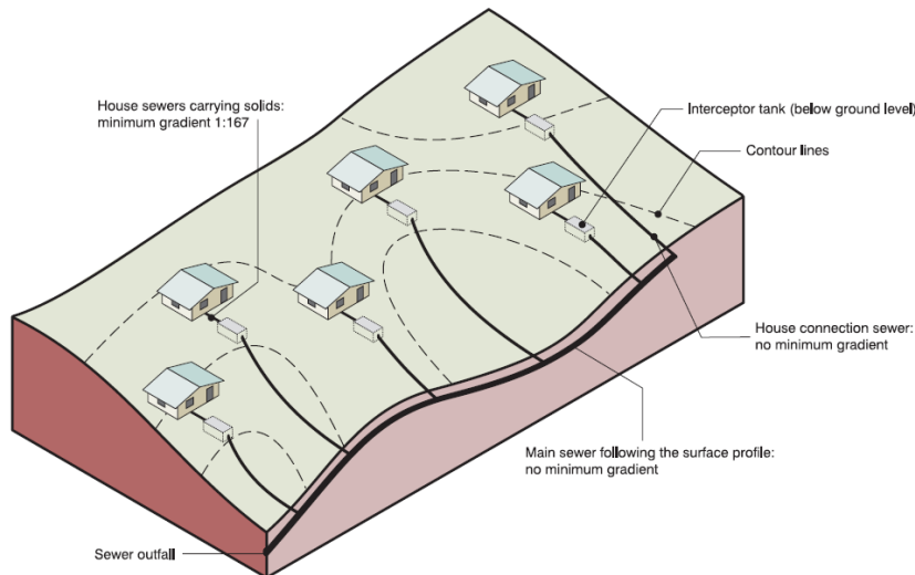
Figure 2: A schematic cut-away view of a sewerage system (Source WELL, 1998)
