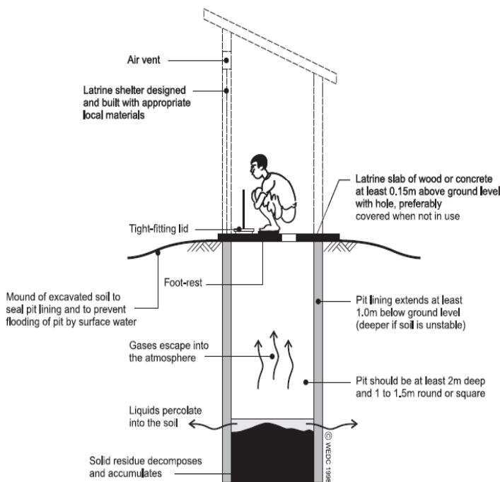
Figure 3: A simple pit latrine (Source: Harvey et al, 2002)
