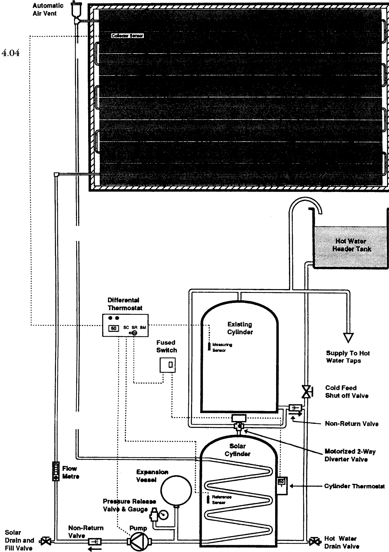
Fig 4.14 Active solar hot water heating system from AES (Appropriate Energy Systems Ltd.)
