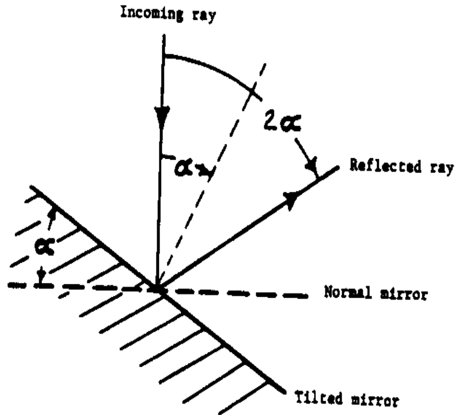
Figure 2. Tilted Mirror
