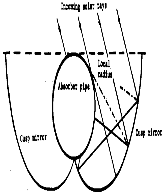
Figure 19. Diagram of the Trombe-Meinell Cusp Design for 180 Degree Acceptance Angle
