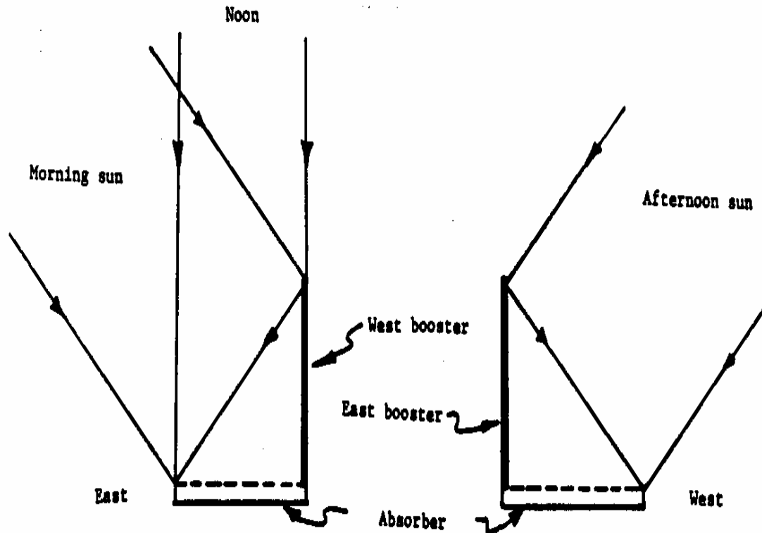
Figure 15. Flat Plate with Booster Mirrors
