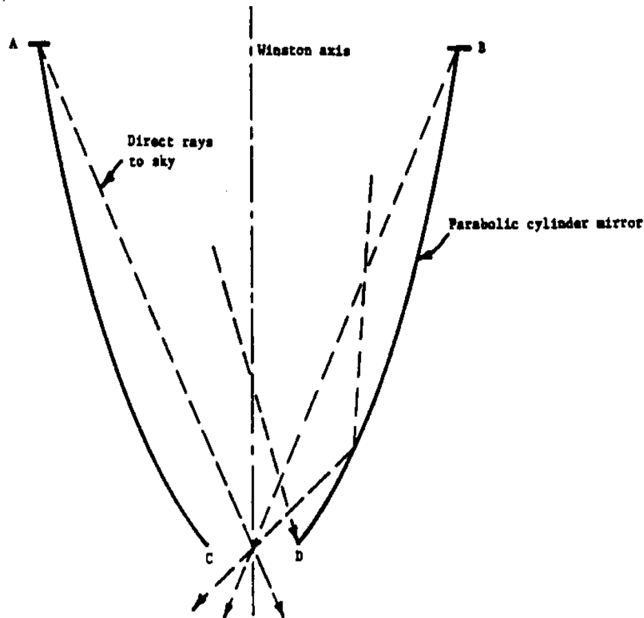
Figure 18. Winston Collector
