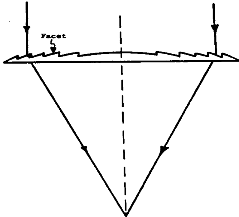
Figure 4. Fresnel Lens
