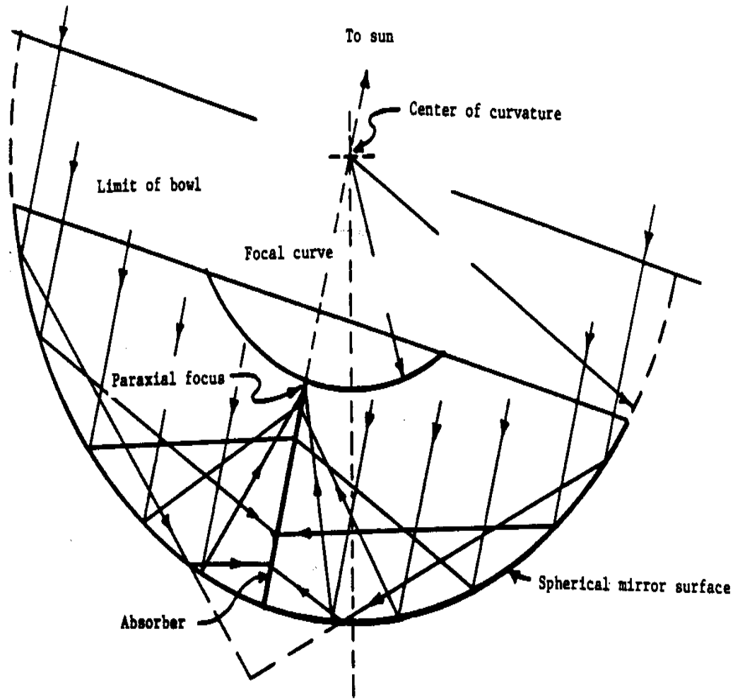
Figure 11. Basic Geometry of the Hemispherical Bowl Collector
