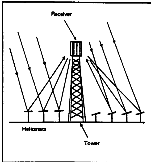
Figure 8. The Central Receiver Design Concept
