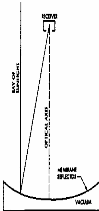
Figure 22. Diagram of a Pressure-Stabilized Membrane Reflector
