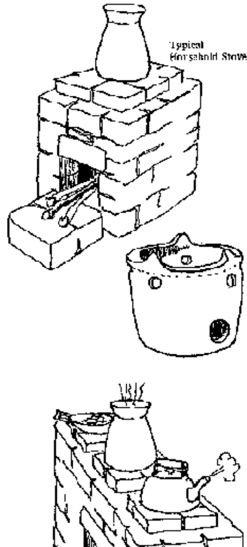
Fig. 7-89: Packed Stoves
