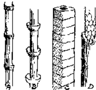
Fig. 7-25: Chimneys. A Bamboo chimney; B Terra cotta drainage pipes; C Sand/clay blocks; D Ferro-mud (wire netting and mud).
