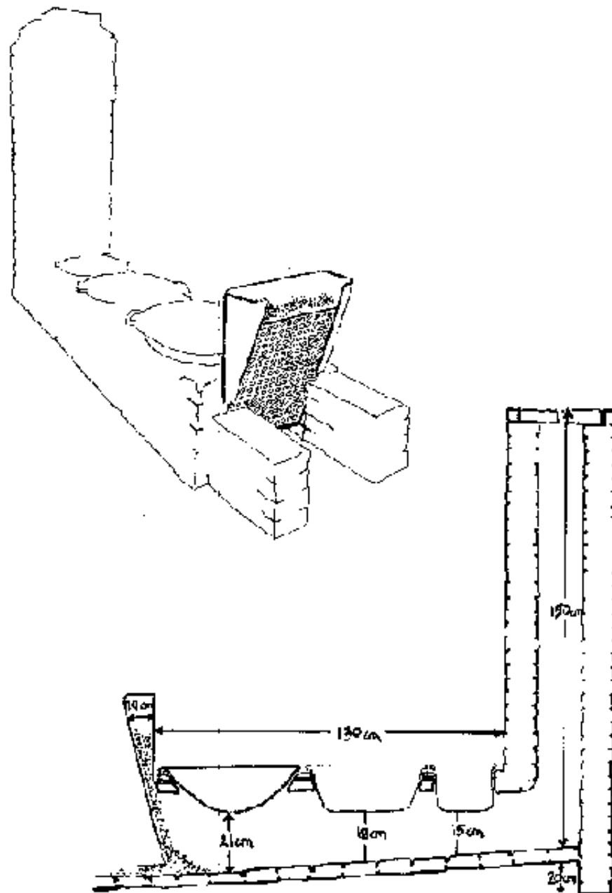
Fig. 7-94: "Gula Jawa" Stove
