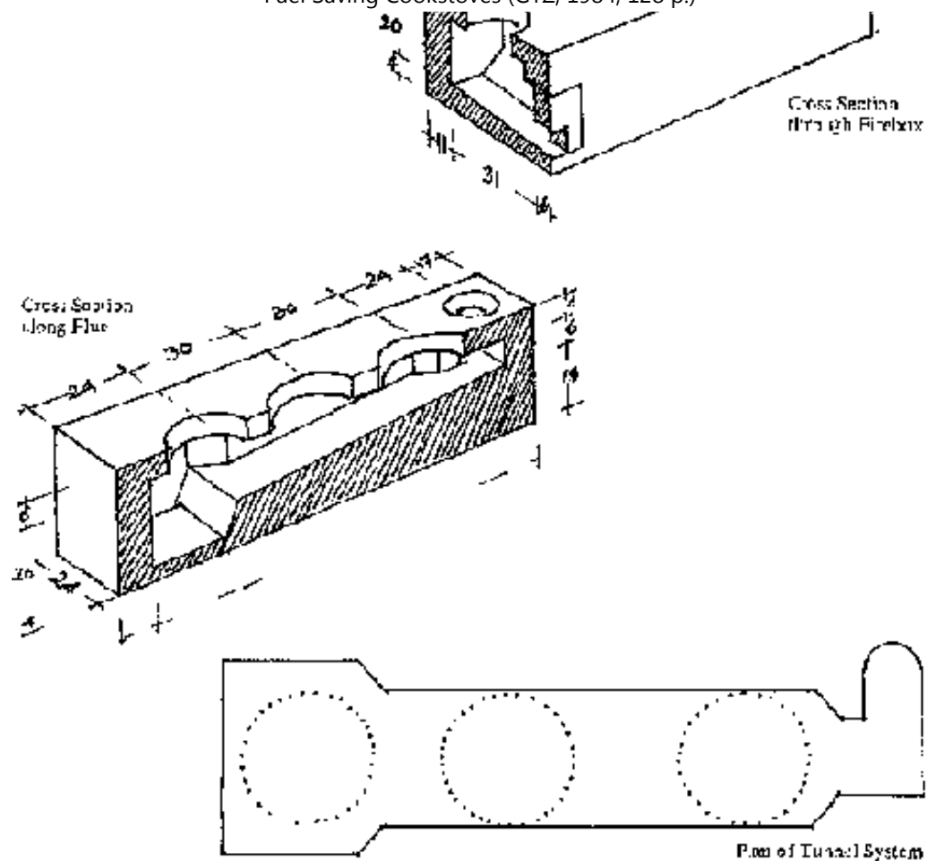
Fig. 7-77: Construction of the Singer Stove.
