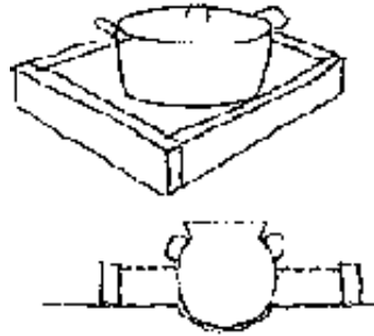
Fig. 7-73: Pots may be sunk through the plate by digging them into the ground before casting.
