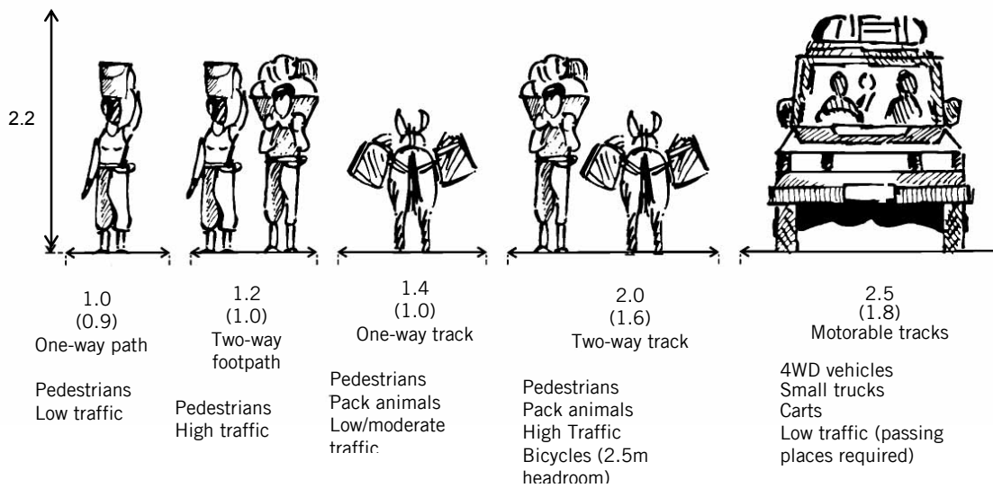
Figure 1: Width guidelines for paths and tracks
