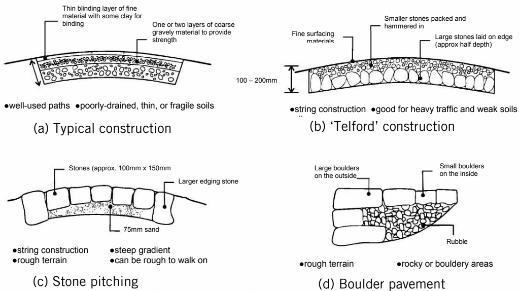
Figure 4: Surfacing methods for paths and tracks
