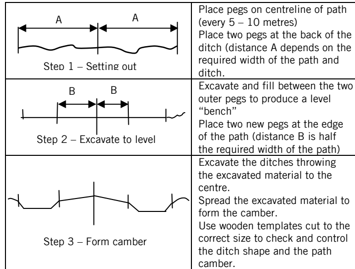
Figure 5: Construction sequence
