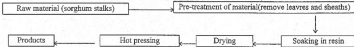
Figure 9: The processing method of sorghum plywood
