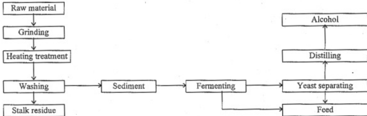
Figure 13: Flowing Diagram of Making Alcohol by Using Sweet Sorghum Stalks
