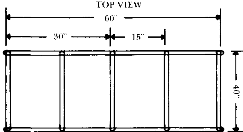
FIGURE 7: 2-CAGE, ALL WIRE QUONSET HUTCH
