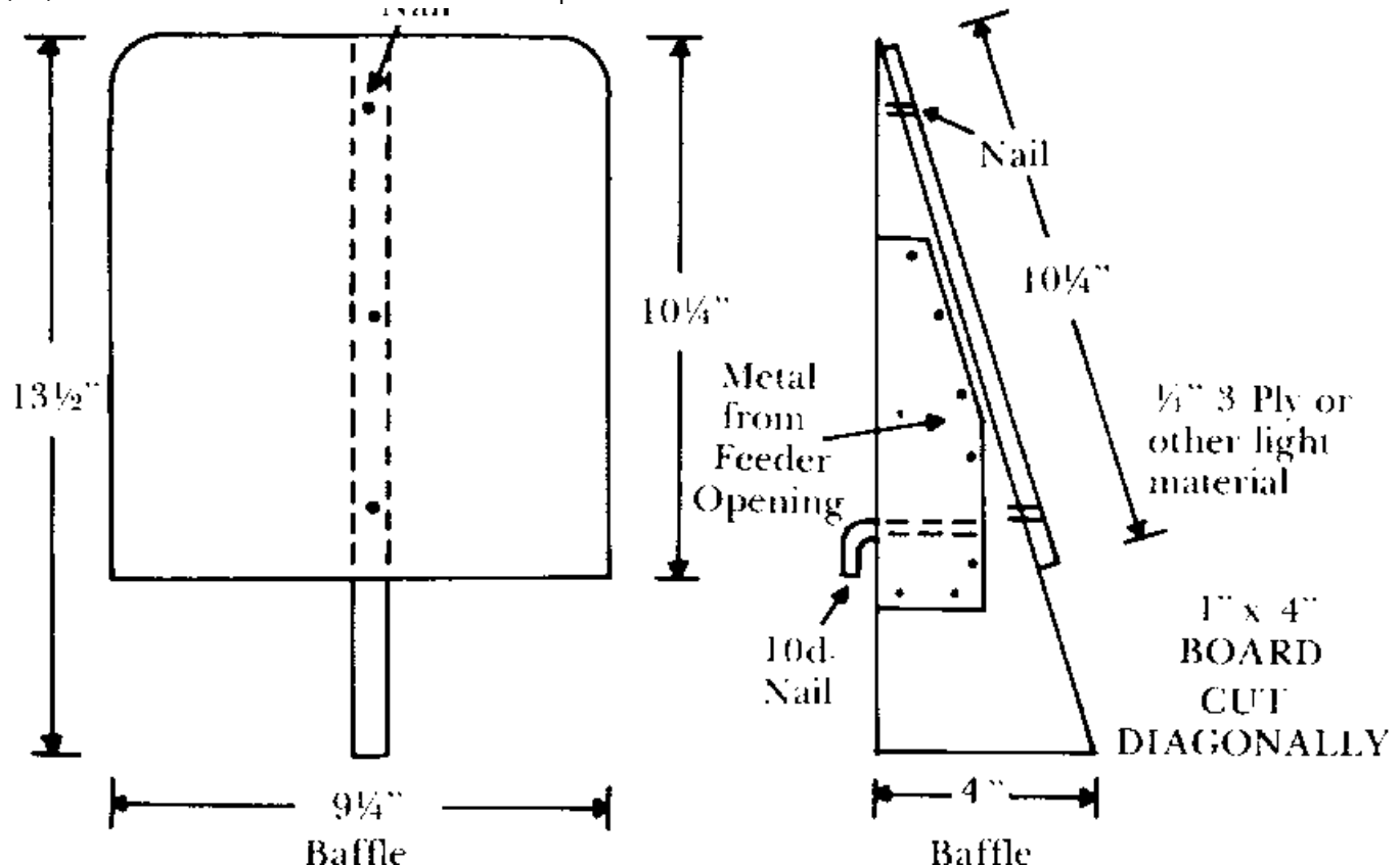
FIGURE 10 - DESIGNS FOR FEED HOPPER MADE FROM 5-GALLON CAN
