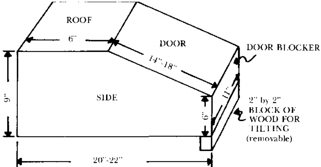
FIGURE 13 - STANDARD NEST BOX
