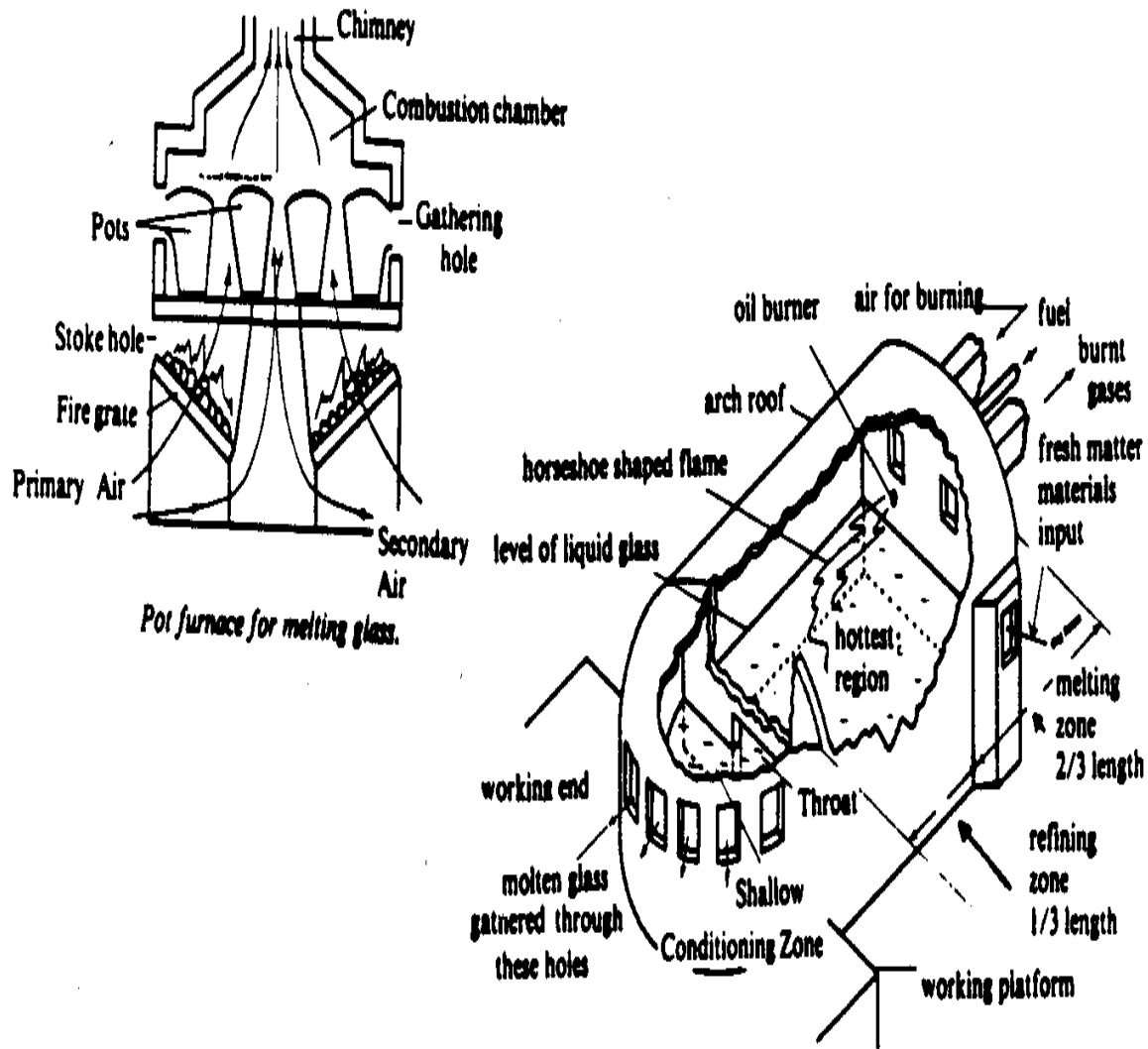
Diagram of a small, oil-fired glass tank furnace.
