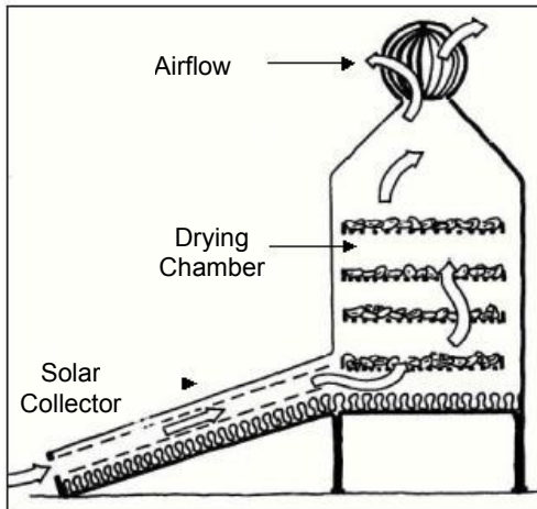
Figure 1: Solar drier components (Brace Research Inst.)
