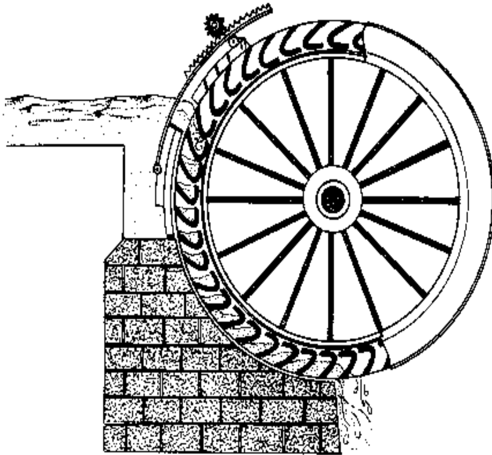
buckets on a breast wheel
