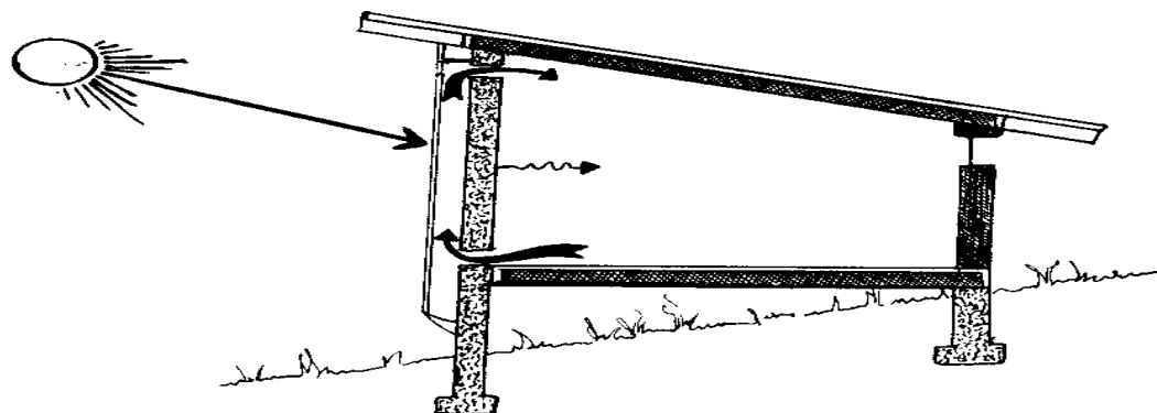
trombe wall - winter
