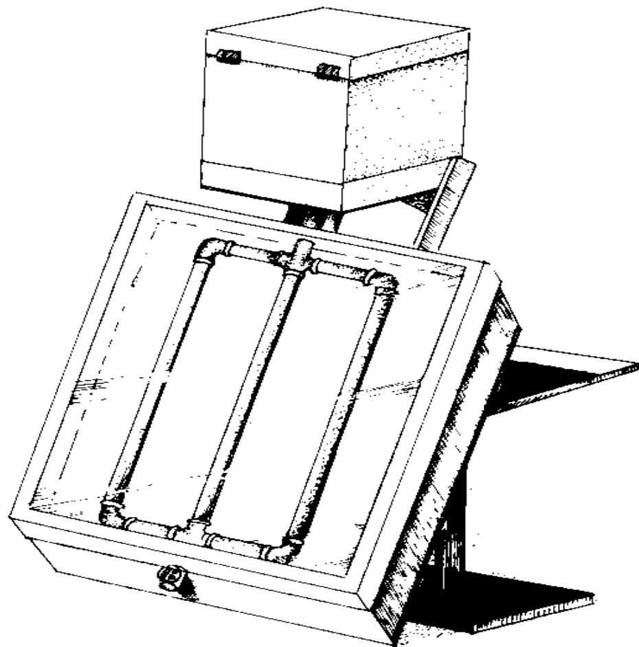
Brace solar steam cooker
