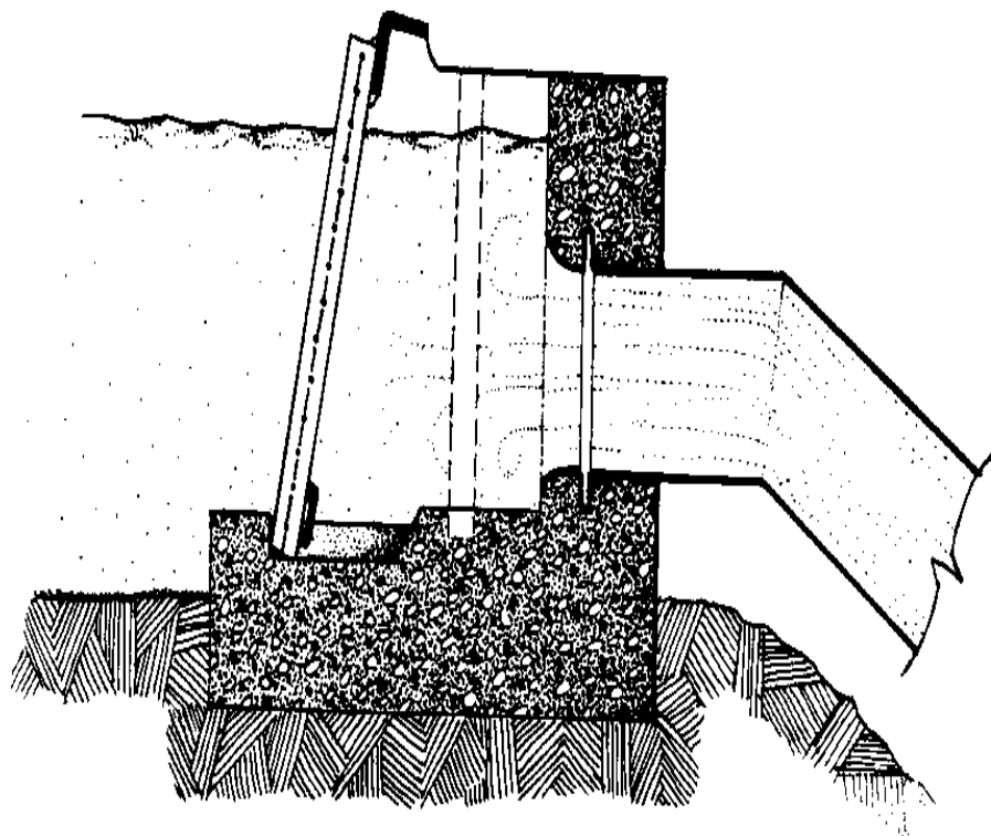
penstock intake (cutaway view)
