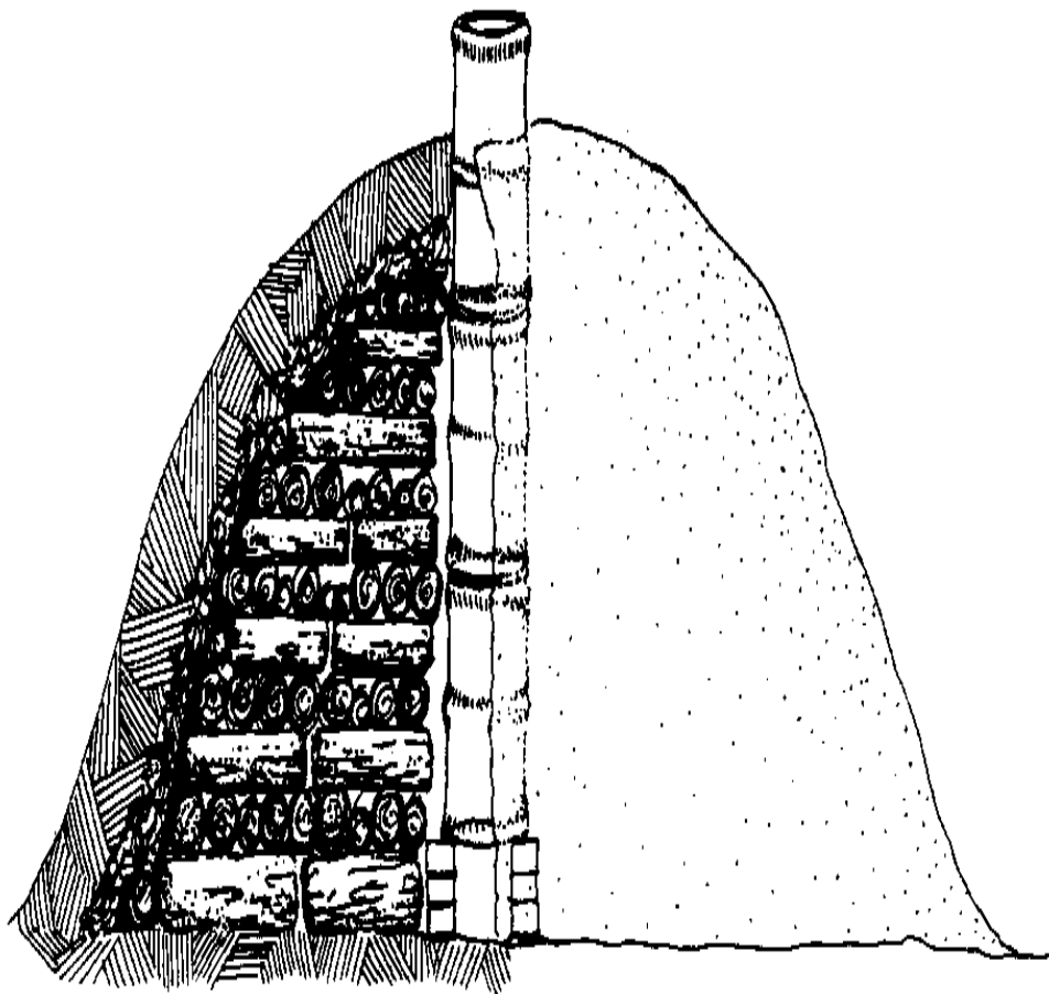
earth kiln (cutaway view)
