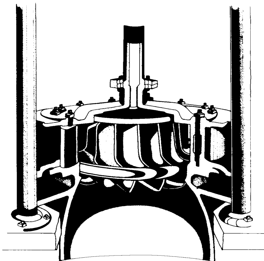
Francis turbine (cutaway view)
