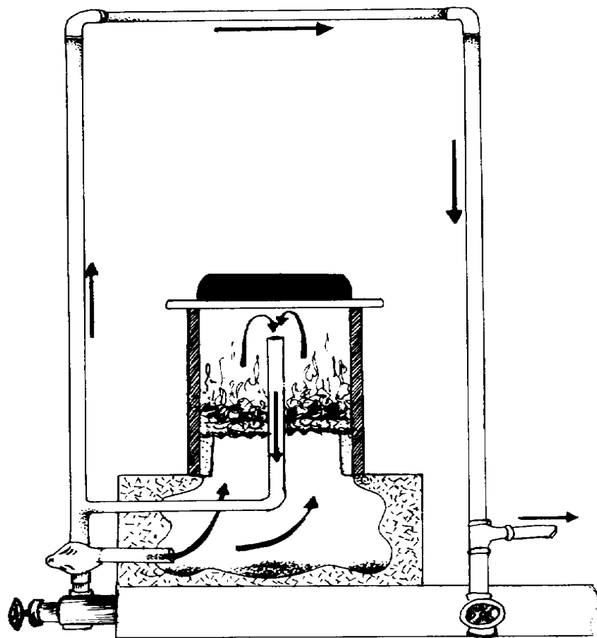
producer gas generator (cutaway view)
