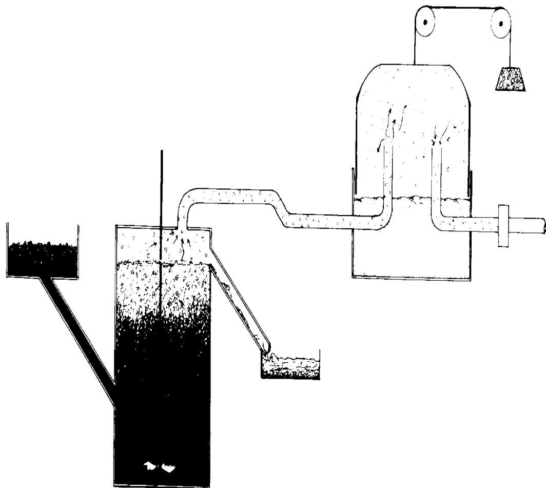
biogas digester
