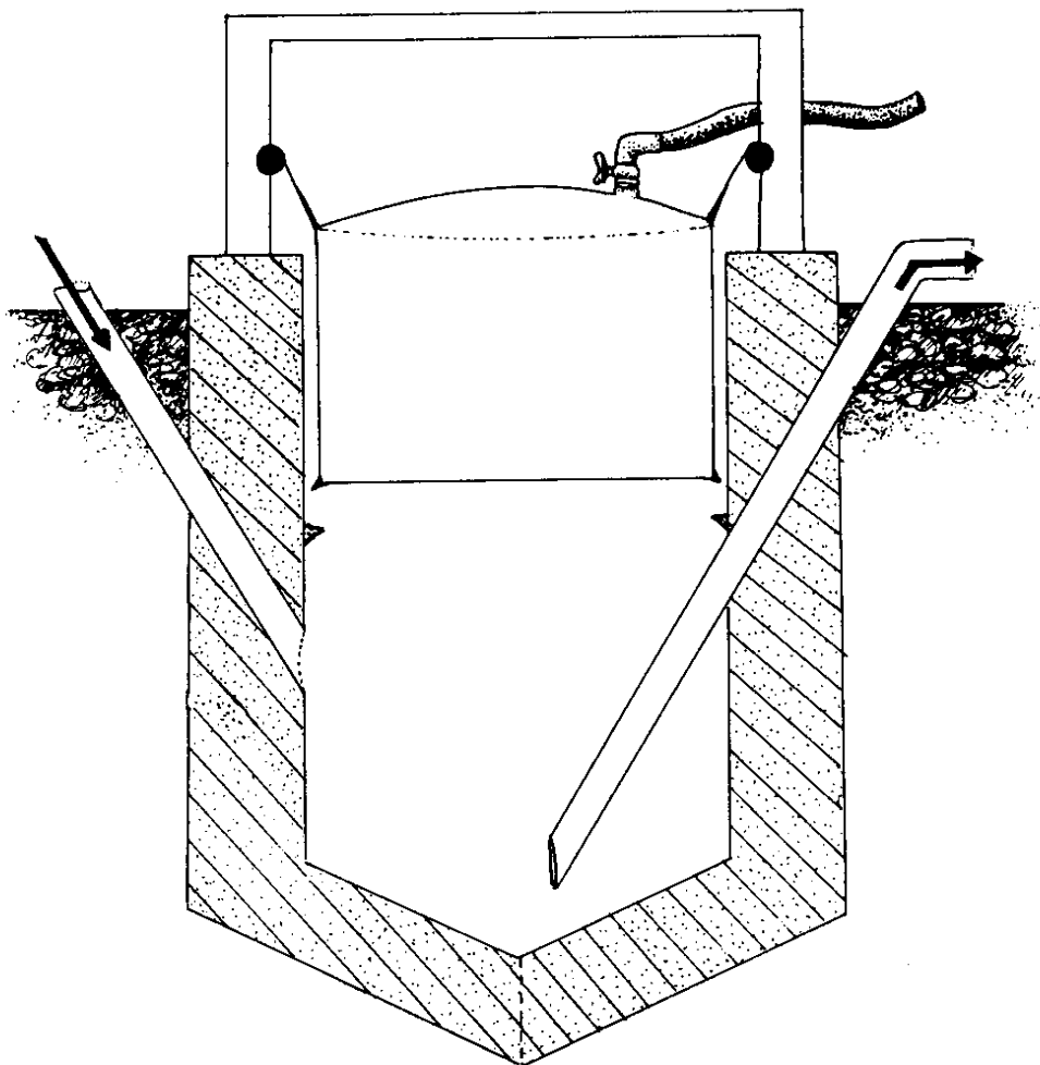
Indian-type digester
