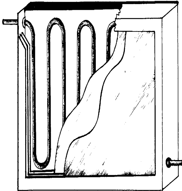
flat-plate solar water heater (cutaway view)
