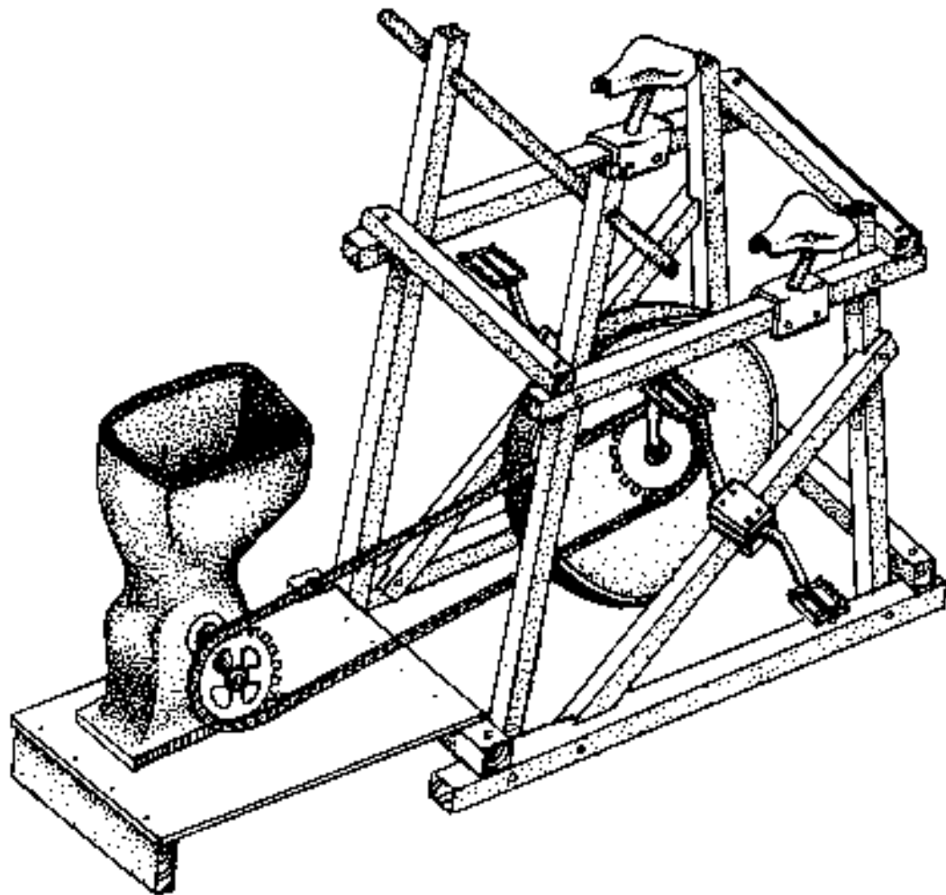
dynapod with chain drive and grinder
