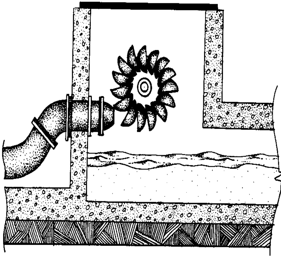
impulse turbine (cutaway view)
