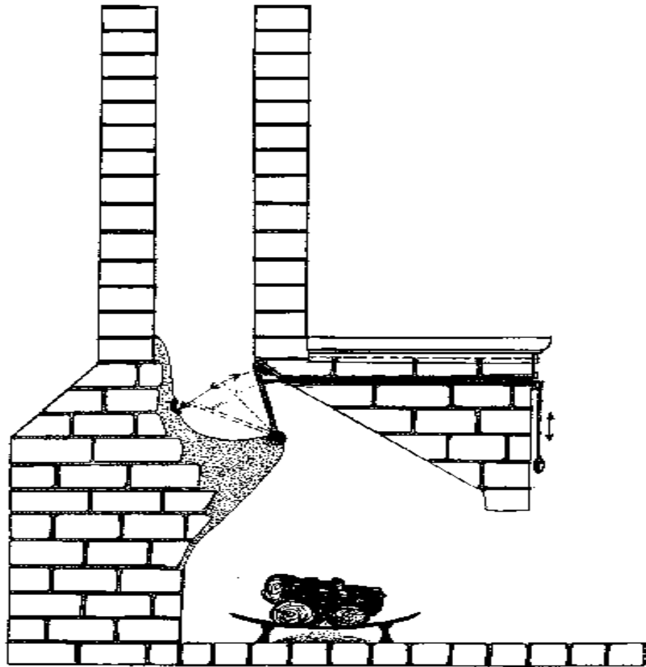
damper in a fireplace
