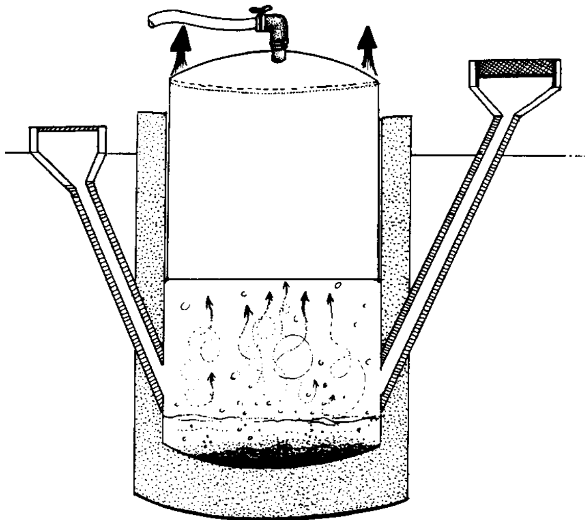
floating gas cap
