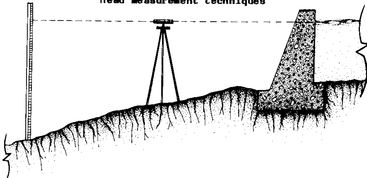
head measurement techniques
