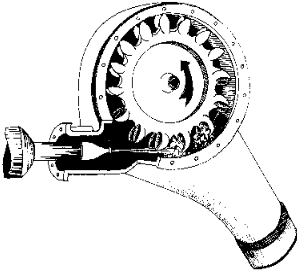
Pelton wheel
