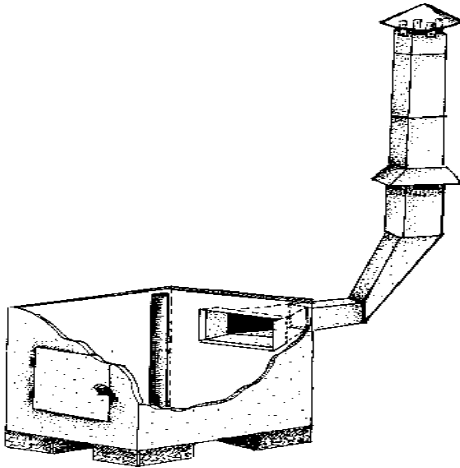
sandust burning stove (cutaway view)
