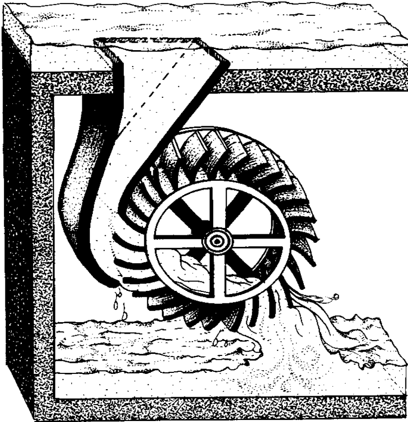
Banki turbine
