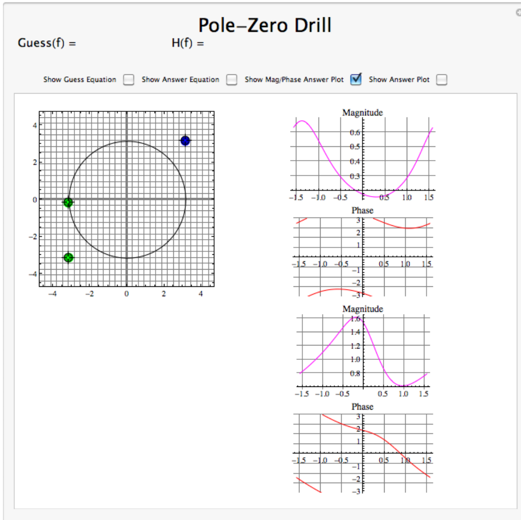
Figure 3.9: Interact (when online) with a Mathematica CDF demonstrating Pole/Zero Plots. To Download, right-click and save target as .cdf.
