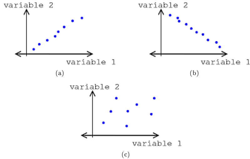
Figure 4.5: Types of Correlation (a) Positive Correlation (b) Negative Correlation (c) Uncorrelated (No Correlation)
