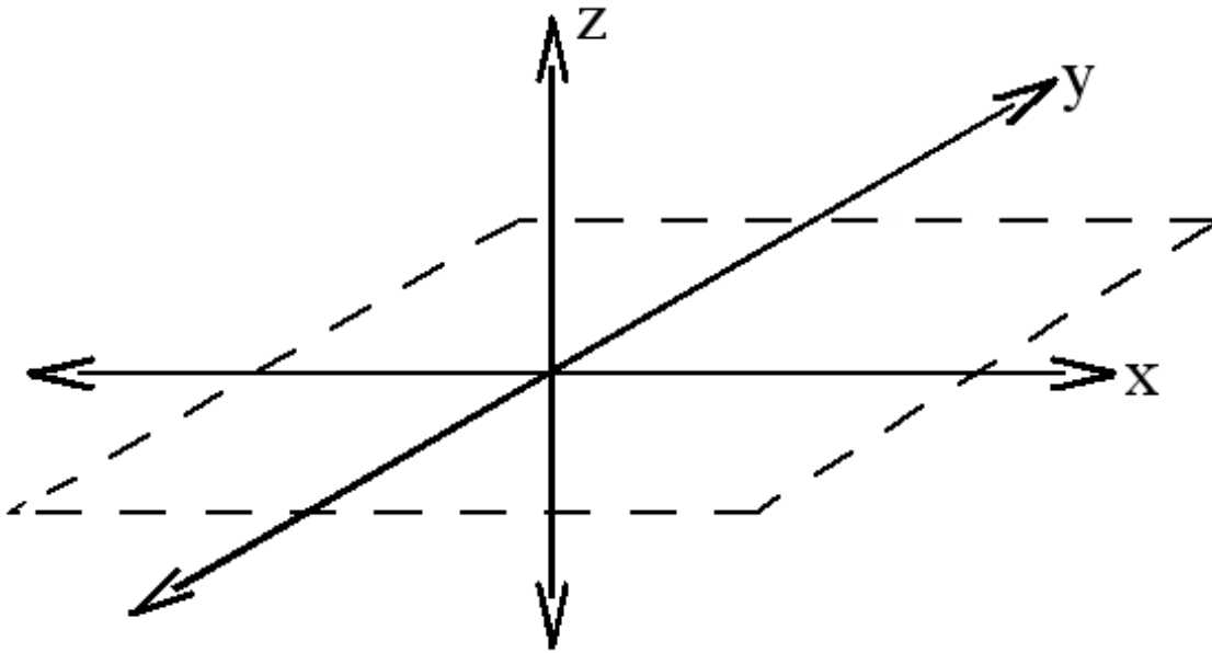
Figure 1.11: \langle S \rangle is the xy-plane.
