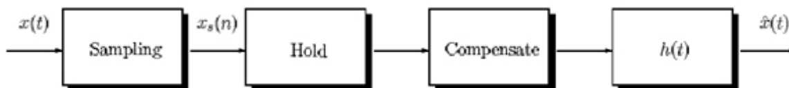
Figure 2.9: More practical reconstruction system with a hold component 34
