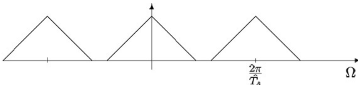
Figure 2.4: The spectrum X_s . Sampling frequency is OK.
