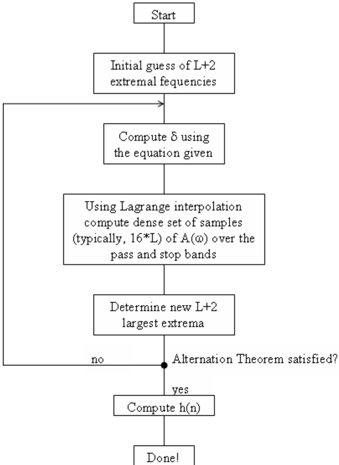
Figure 3.18: The initial guess of extremal frequencies is usually equally spaced in the band. Computing \delta costs O(L^2) . Using Lagrange interpolation costs O(16LL) \simeq O(16L^2) . Computing h(n) costs O(L^3) , but it is only done once!
