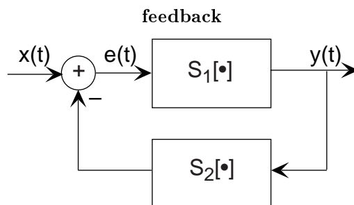
Figure 1.6: The feedback configuration.
