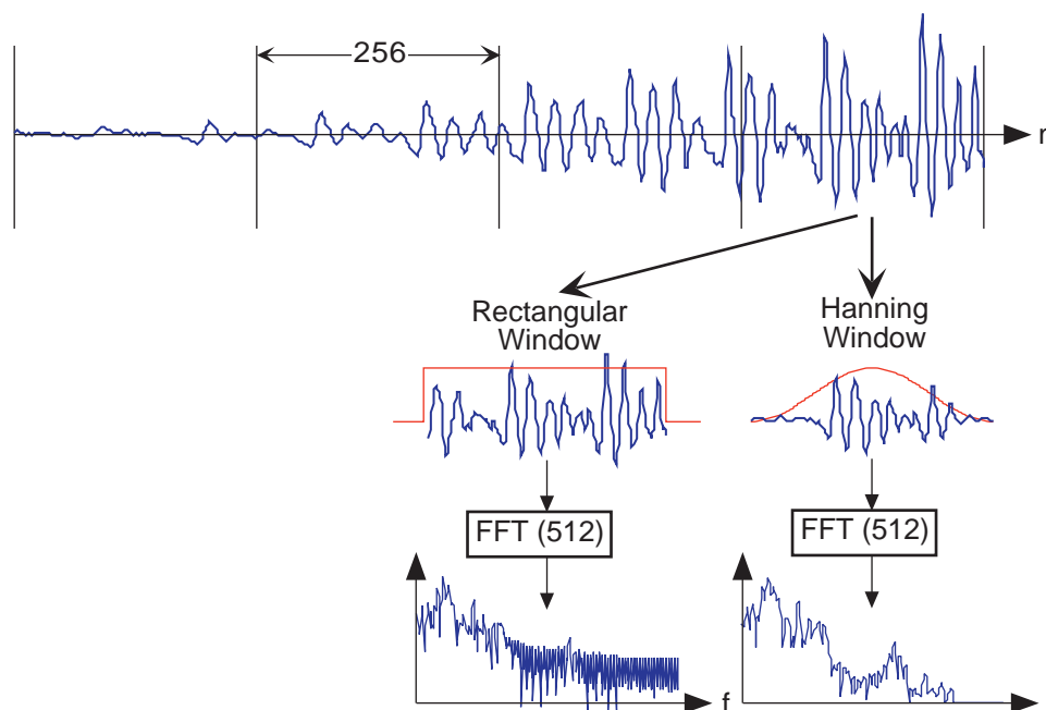
Figure 2.47: The top waveform is a segment 1024 samples long taken from the beginning of the "Rice University" phrase. Computing Figure 2.46 (Speech Spectrogram) involved creating frames, here demarked by the vertical lines, that were 256 samples long and finding the spectrum of each. If a rectangular window is applied (corresponding to extracting a frame from the signal), oscillations appear in the spectrum (middle of bottom row). Applying a Hanning window gracefully tapers the signal toward frame edges, thereby yielding a more accurate computation of the signal's spectrum at that moment of time.
