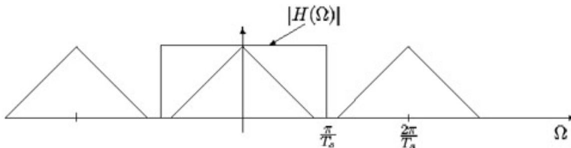
Figure 2.6: H(i\Omega) The ideal reconstruction filter.
