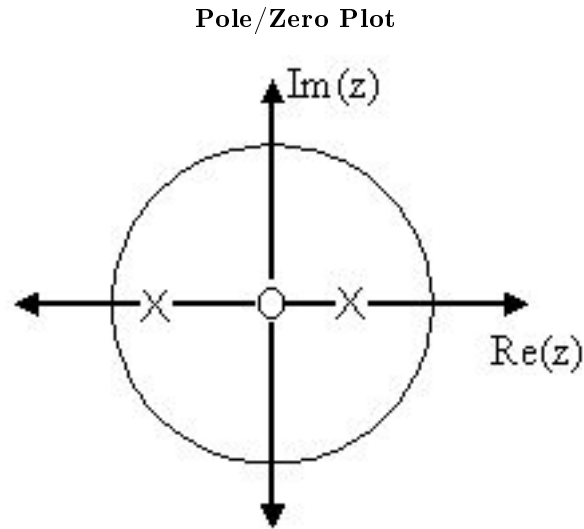
Figure 3.7: Using the zeros and poles found from the transfer function, the one zero is mapped to zero and the two poles are placed at \frac{1}{2} and -\frac{3}{4}
