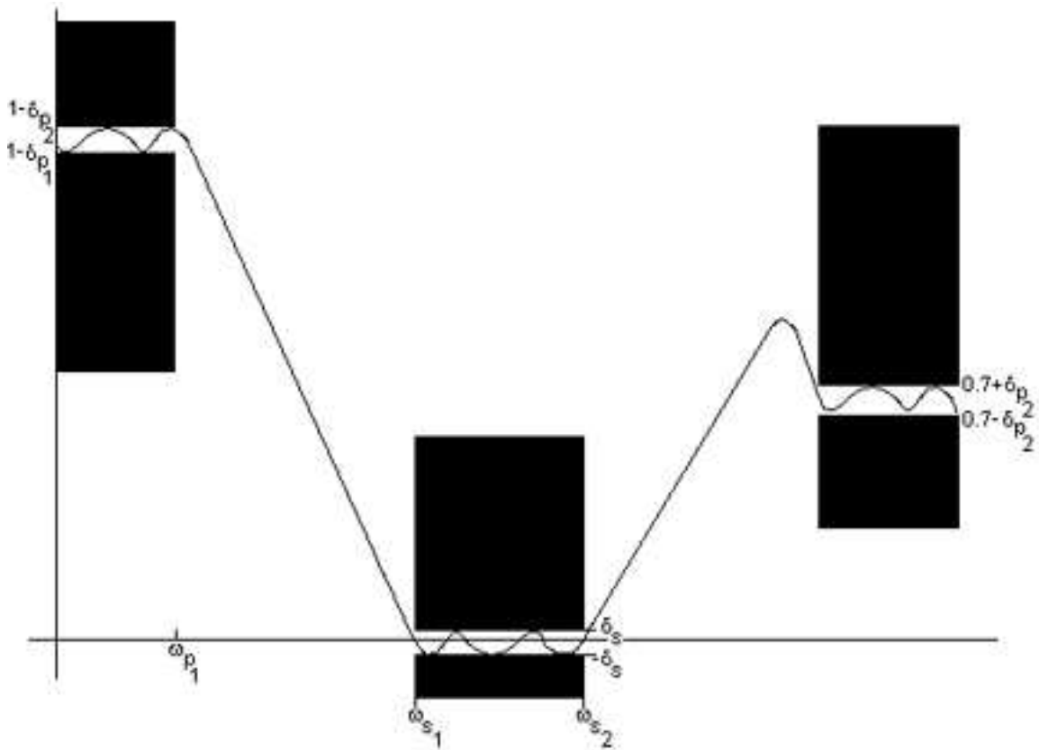
Figure 3.16: The black boxes on the left and right are the passbands, the black boxes in the middle represent the stop band, and the space between the boxes are the transition bands. Note that overshoots may be allowed in the transition bands.
