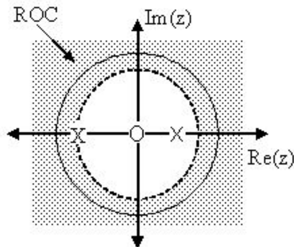
Figure 3.10: The shaded area represents the chosen ROC for the transfer function.
