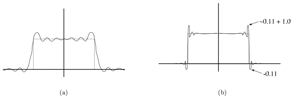
Figure 3.19: (a) A(\omega) , small M (b) A(\omega) , large M
