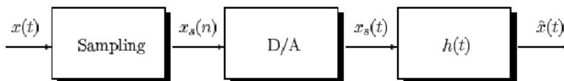
Figure 2.7: Ideal reconstruction system
