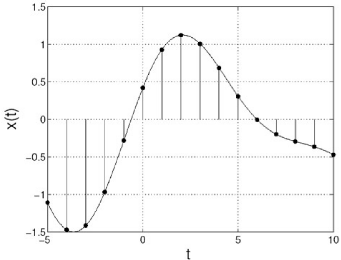
Figure 2.2: Analog signal, samples are marked with dots.
