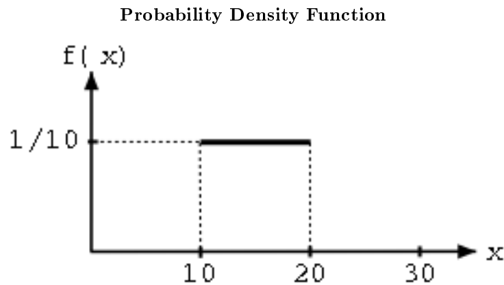
Figure 4.4: A uniform probability density function.
