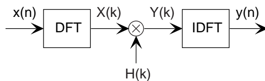
Figure 3.11: To filter a signal in the frequency domain, first compute the DFT of the input, multiply the result by the sampled frequency response, and finally compute the inverse DFT of the product. The DFT's length must be at least the sum of the input's and unit-sample response's duration minus one. We calculate these discrete Fourier transforms using the fast Fourier transform algorithm, of course.
