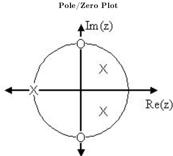
Figure 3.8: Using the zeros and poles found from the transfer function, the zeros are mapped to \pm(i) , and the poles are placed at -1 , \frac{1}{2} + \frac{1}{2}i and \frac{1}{2} - \frac{1}{2}i
