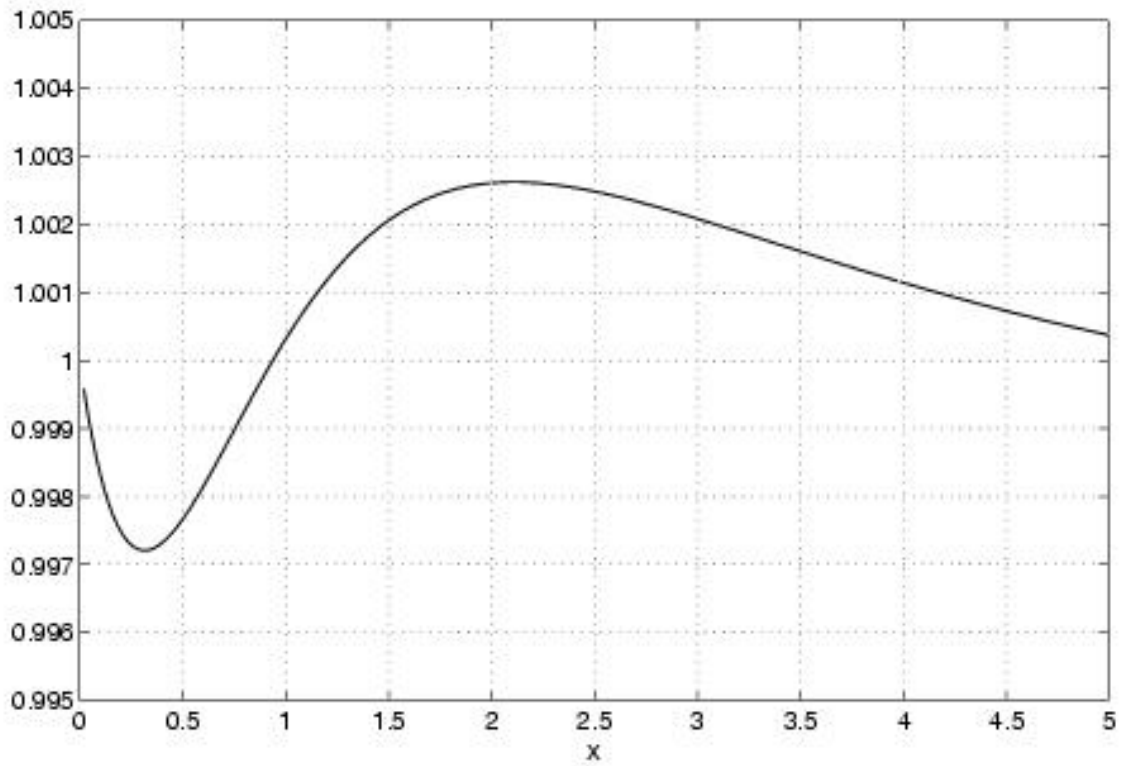
Figure 2.5: The ration of the improved approximation of Q(x) in (2.22) to the true value, obtained by numerical integration.
