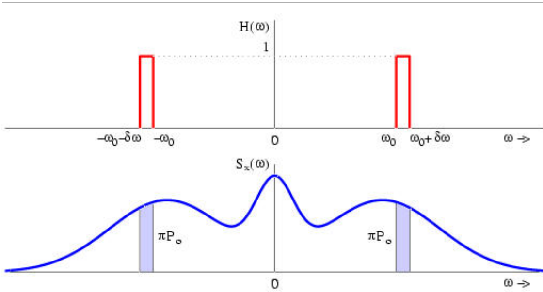
Figure 4.4: Narrowband filter frequency response and PSD of filter input and output.
