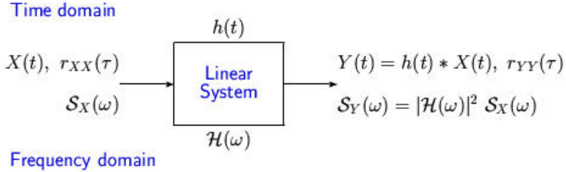
Figure 4.3: Block diagram of a linear system with a random input signal, X(t) .
