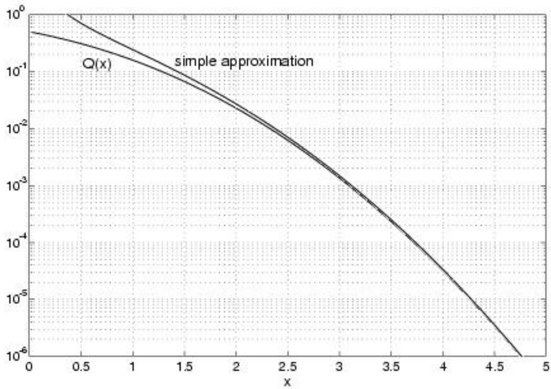
Figure 2.4: Q(x) and the simple approximation of (2.21).
