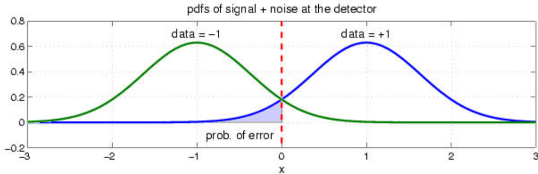
Figure 2.3: The pdfs of the signal plus noise at the detector for the two \pm(1) . The vertical dashed line is the detector threshold and the shaded area to the left of the origin represents the probability of error when data = 1.
