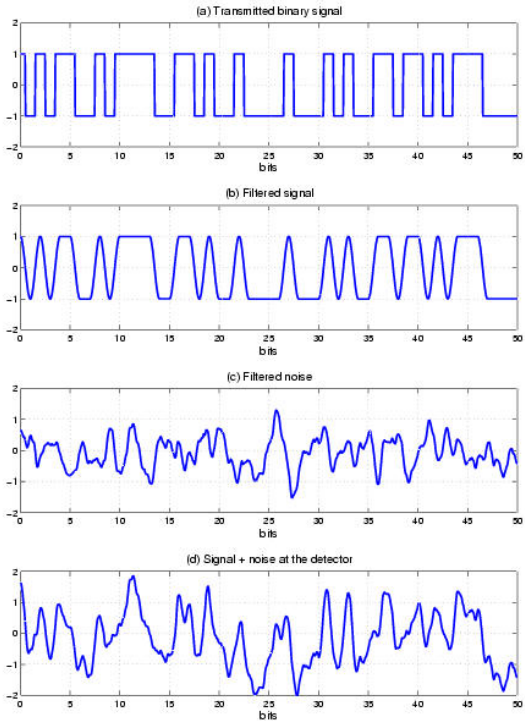
Figure 2.2: Detection of signals in noise: (a) the transmitted binary signal; (b) the binary signal after filtering with a half-sine receiver filter; (c) the channel noise after filtering with the same filter; (d) the filtered signal plus noise at the detector in the receiver.
