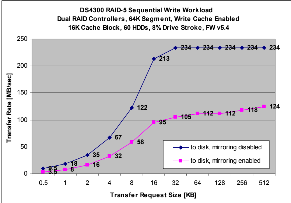
Chart 4. RAID-5 Dual DS4300s Streaming Writes Transfer Rate
