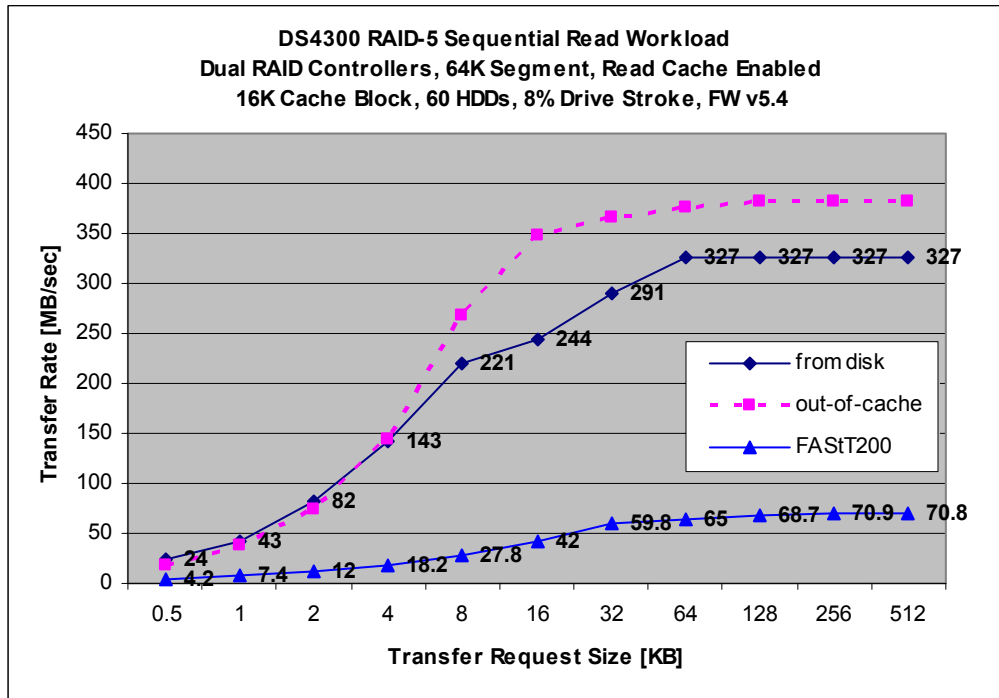
Chart 3. RAID-5 Dual DS4300s Streaming Reads Transfer Rate
