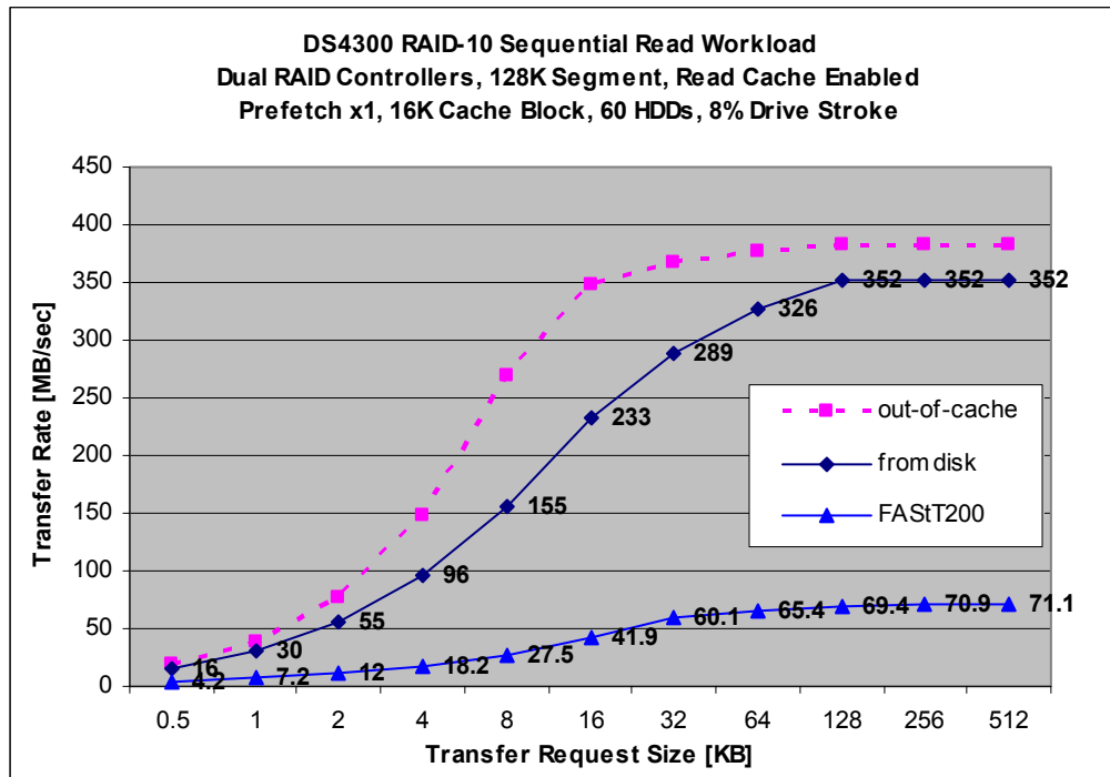
Chart 9. RAID-10 Dual DS4300s Streaming Reads Transfer Rate
