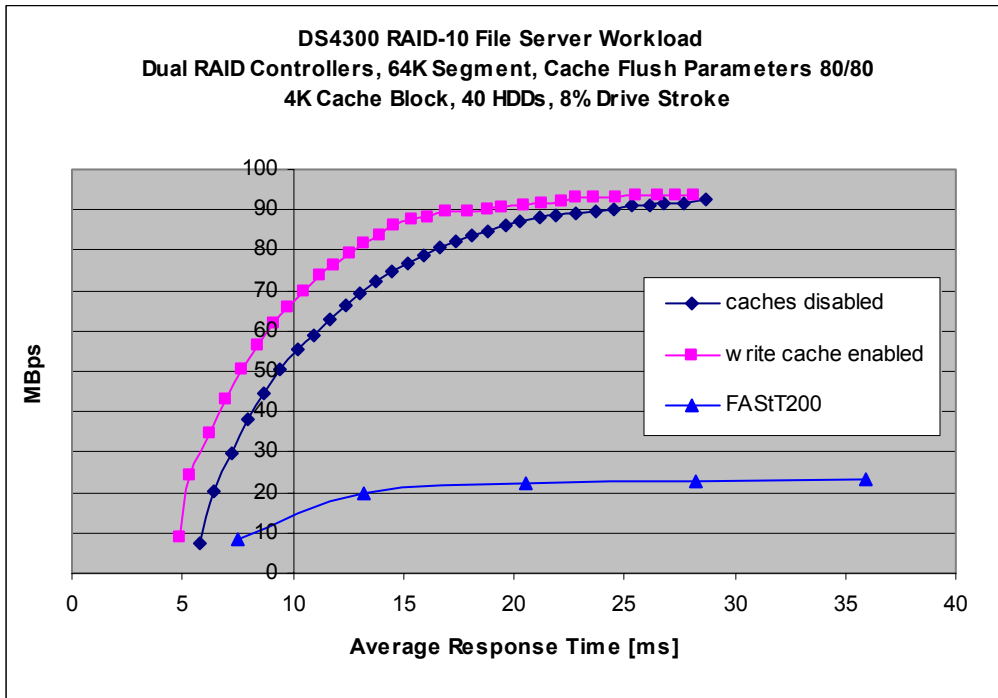
Chart 11. RAID-10 Dual DS4300s File Server vs. Dual FASTt200s
