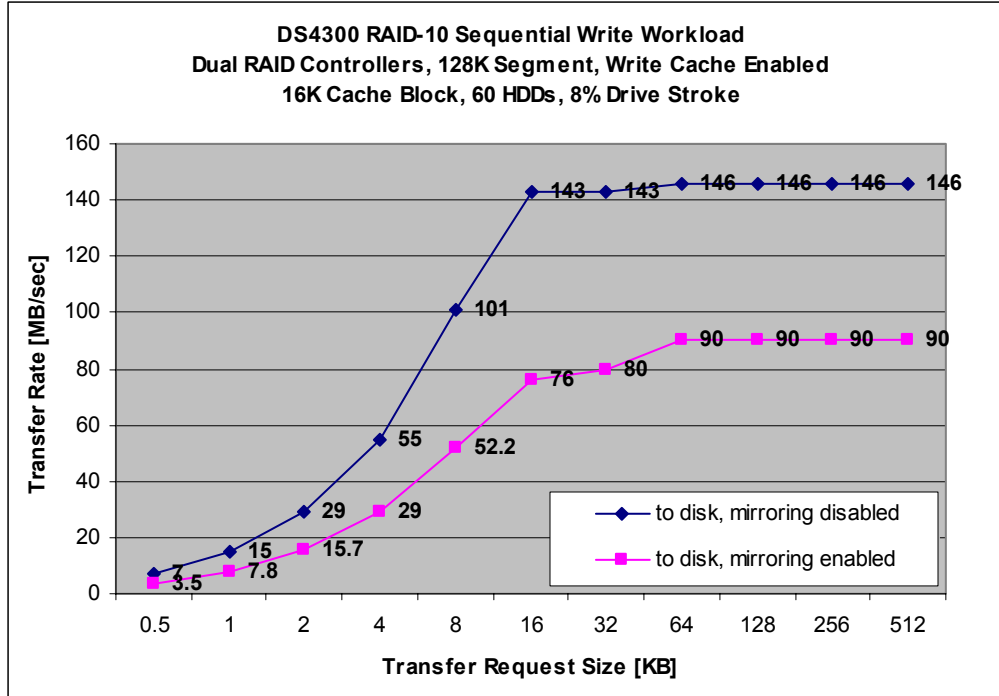
Chart 10. RAID-10 Dual DS4300s Streaming Writes Transfer Rate
