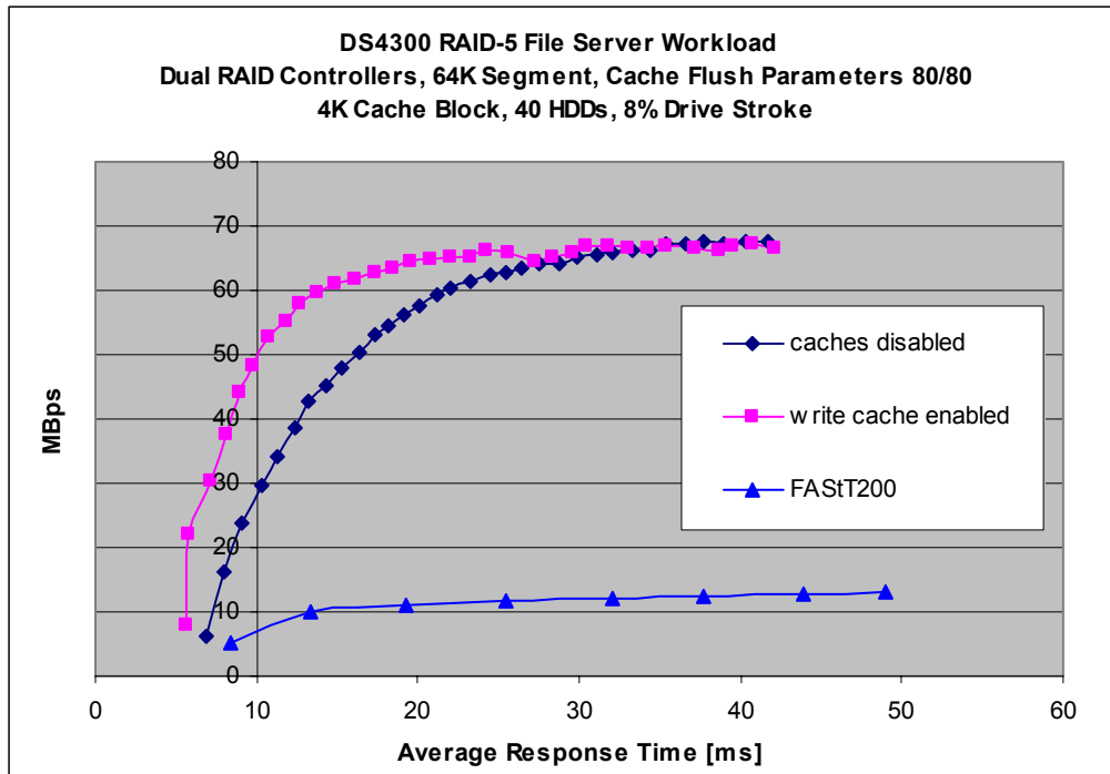
Chart 5. RAID-5 Dual DS4300s File Server vs. Dual FAStT200s
