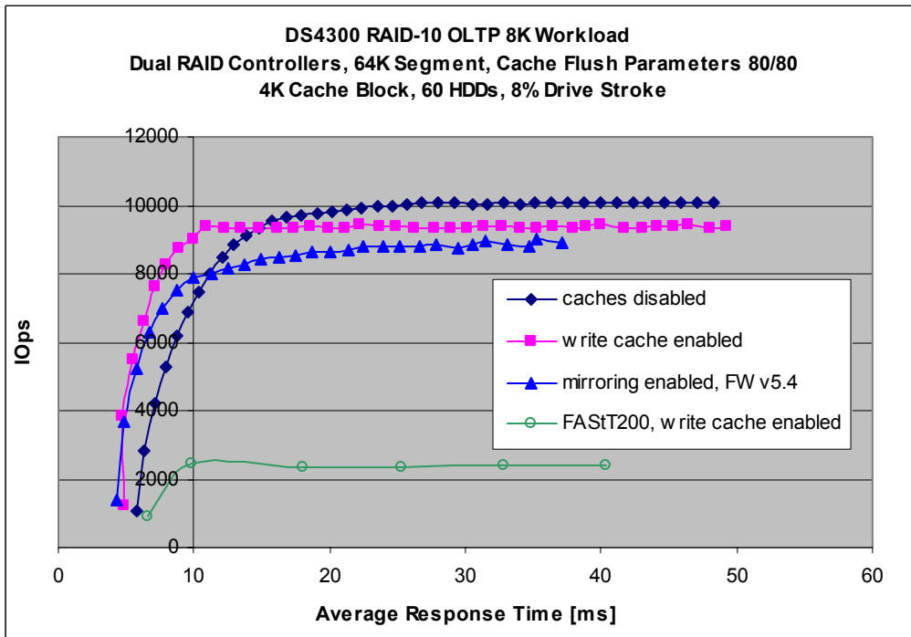
Chart 8. DS4300 RAID-10 OLTP 8K vs. FAStT200
