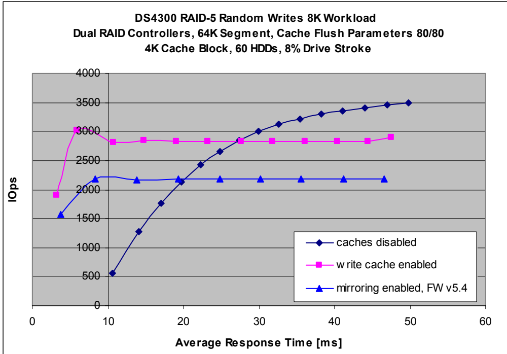
Chart 6. RAID-5 Dual DS4300s Random Writes 8K Workload
