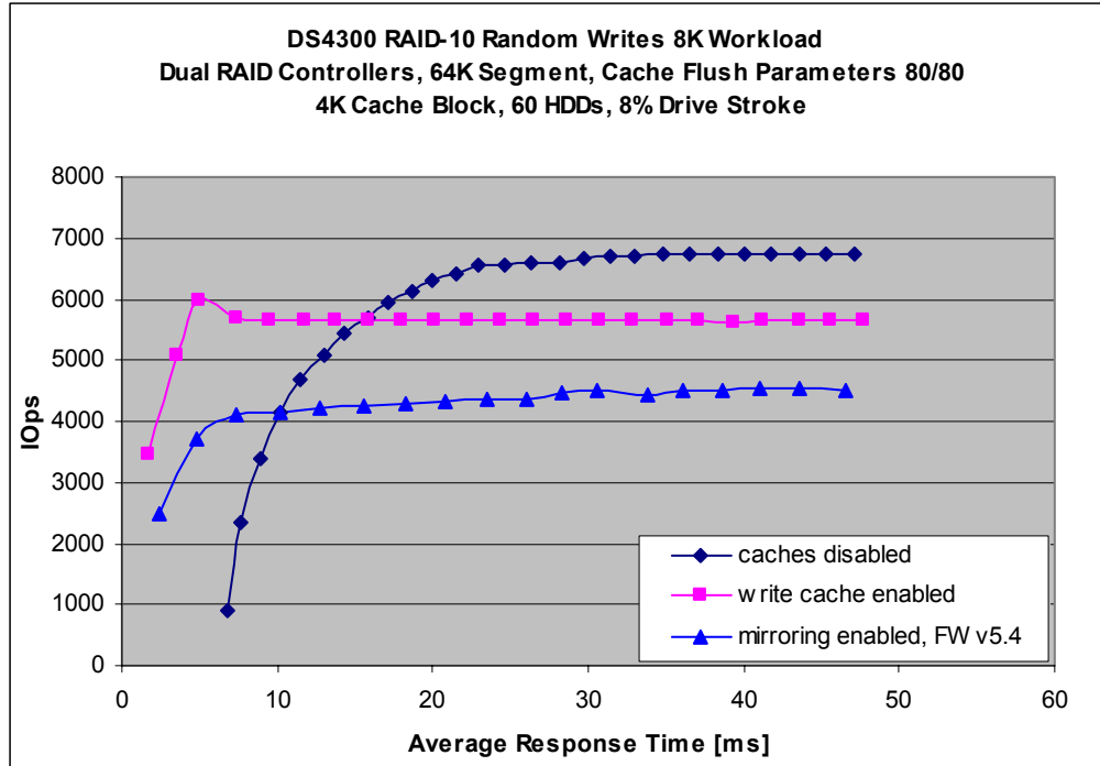
Chart 12. RAID-10 Dual DS4300 Random Writes 8K Workload
