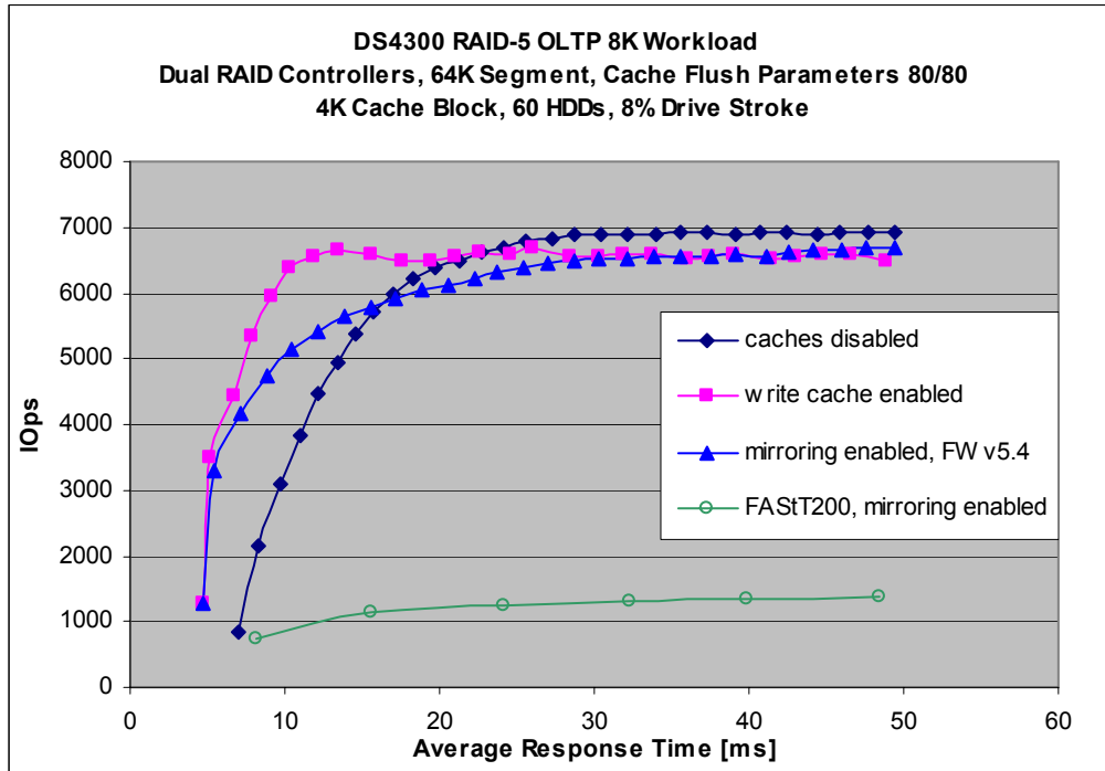
Chart 2. DS4300 RAID-5 OLTP 8K vs. FAStT200 RAID-5 OLTP 8K
