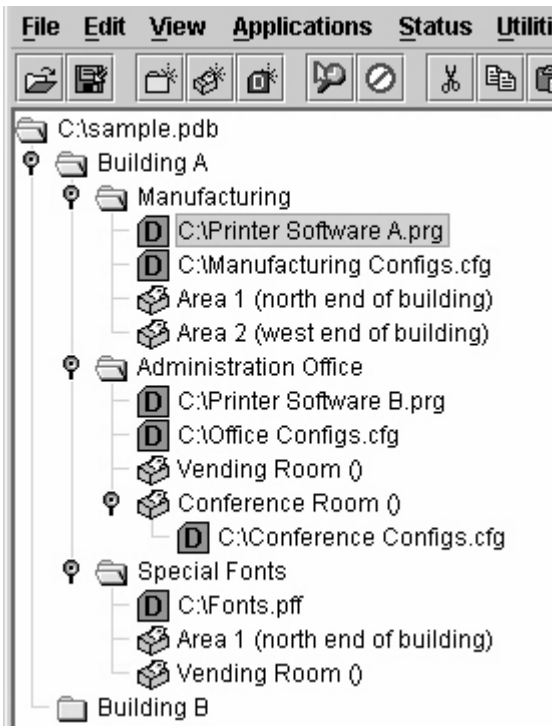
Figure 17. Angled Lines
