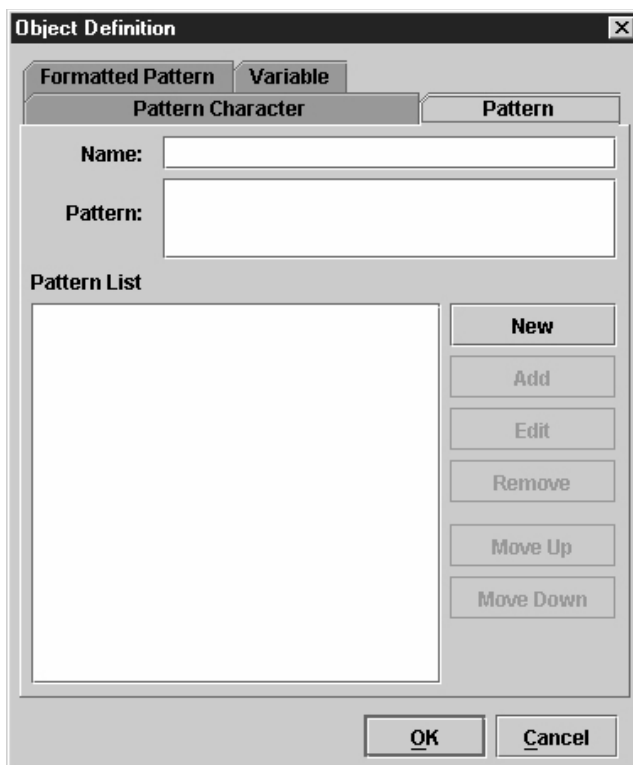
Figure 139. Pattern Tab
