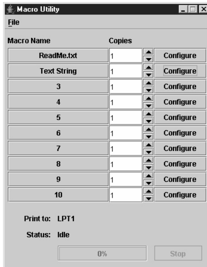
Figure 120. Configured Macros
