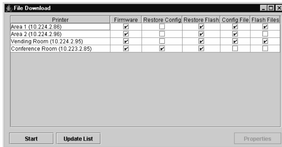
Figure 68. File Download
