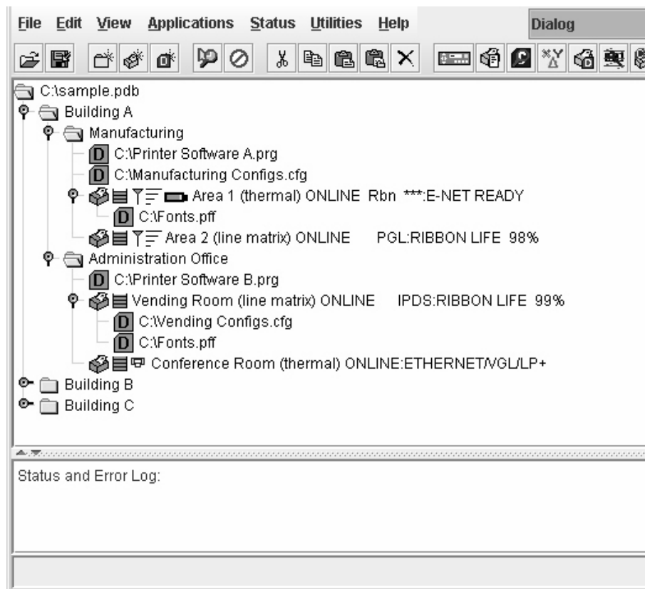
Figure 72. Sample Database
