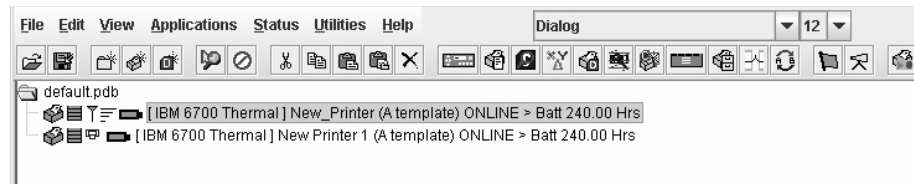
Figure 33. Update Status
