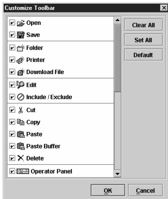
Figure 20. Customize Toolbar
