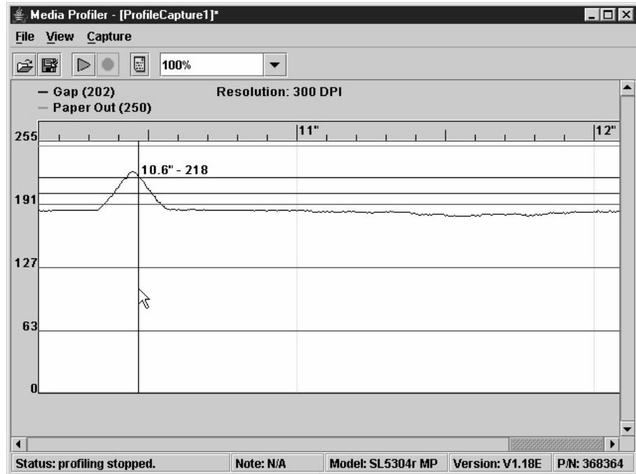
Figure 84. The Crosshair
