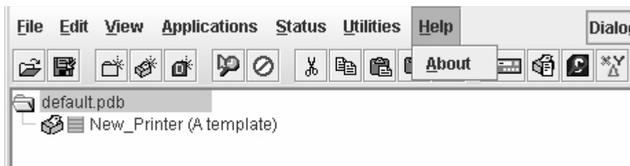
Figure 38. Help Menu
