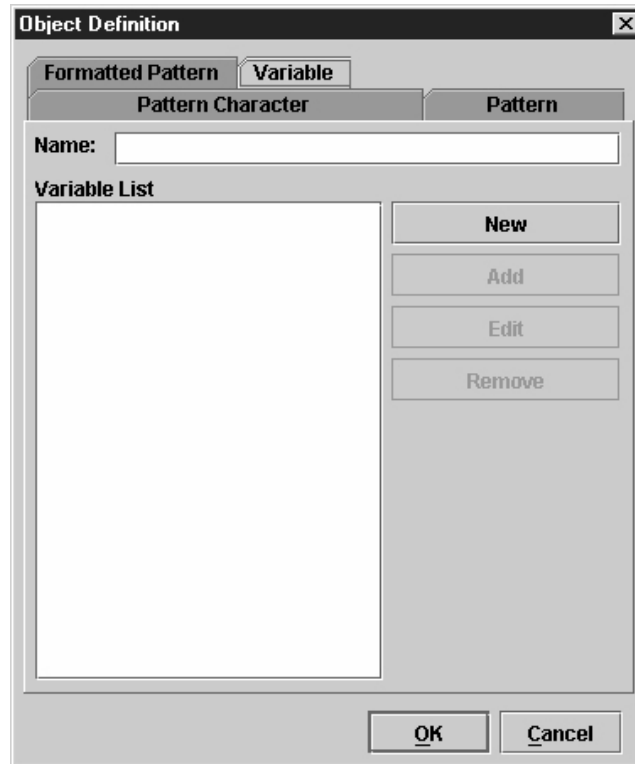
Figure 159. Variable Tab
