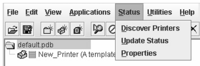
Figure 22. Status Menu
