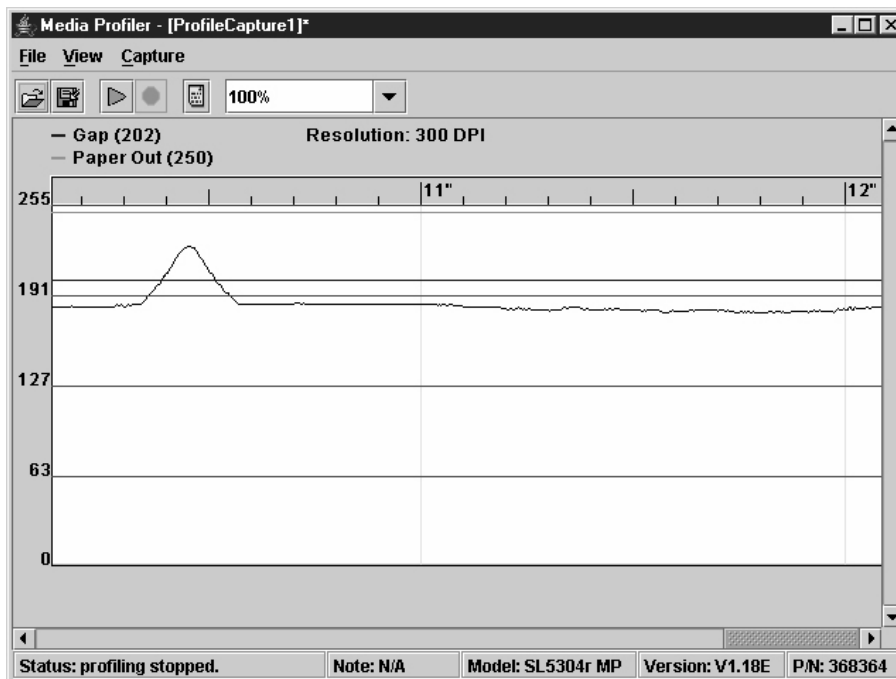
Figure 83. Profiler Graphic
