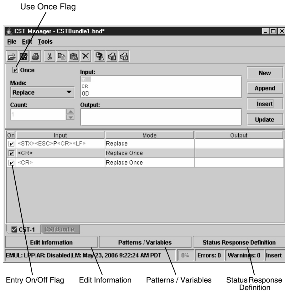
Figure 136. Additional Features
