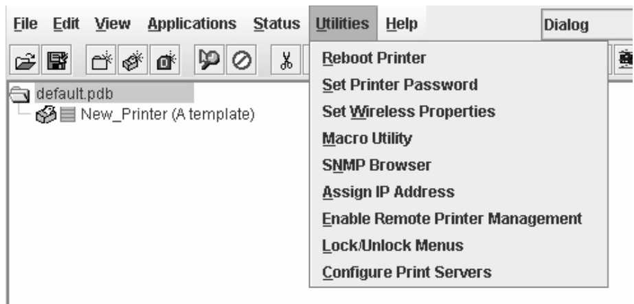
Figure 37. Utilities Menu
