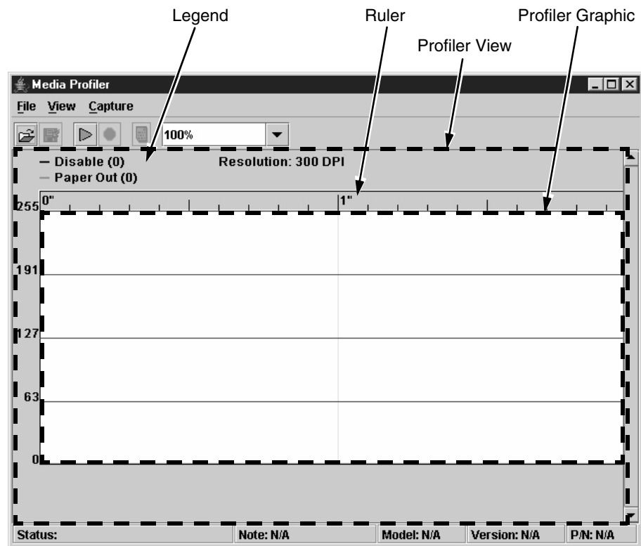
Figure 82. Profiler View
