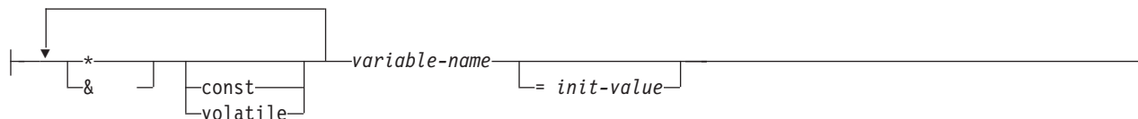
Figure 1. Syntax Diagram
