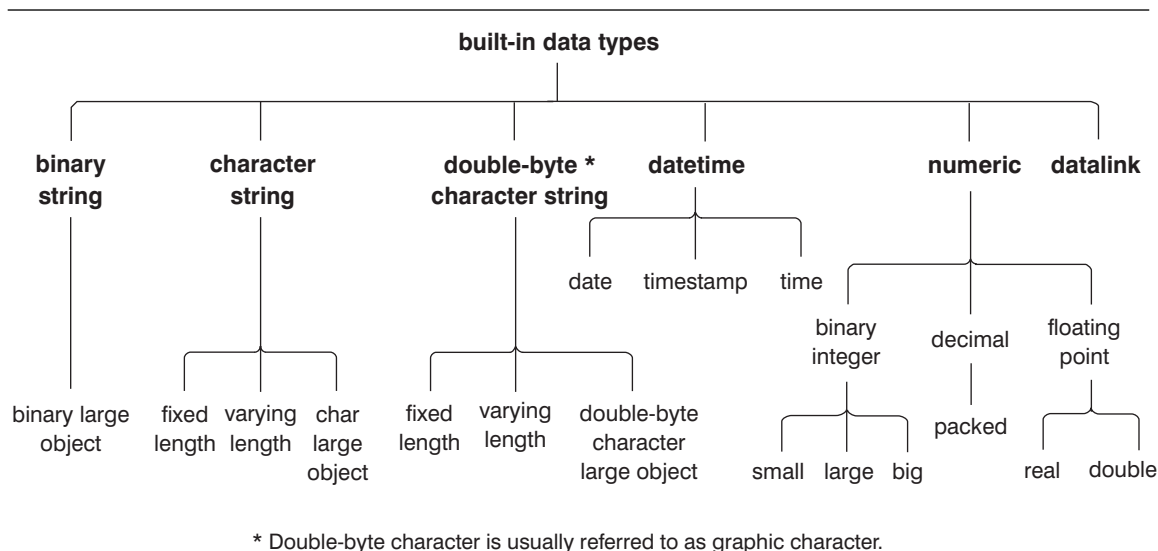
Figure 9. Supported Built-in Data Types
