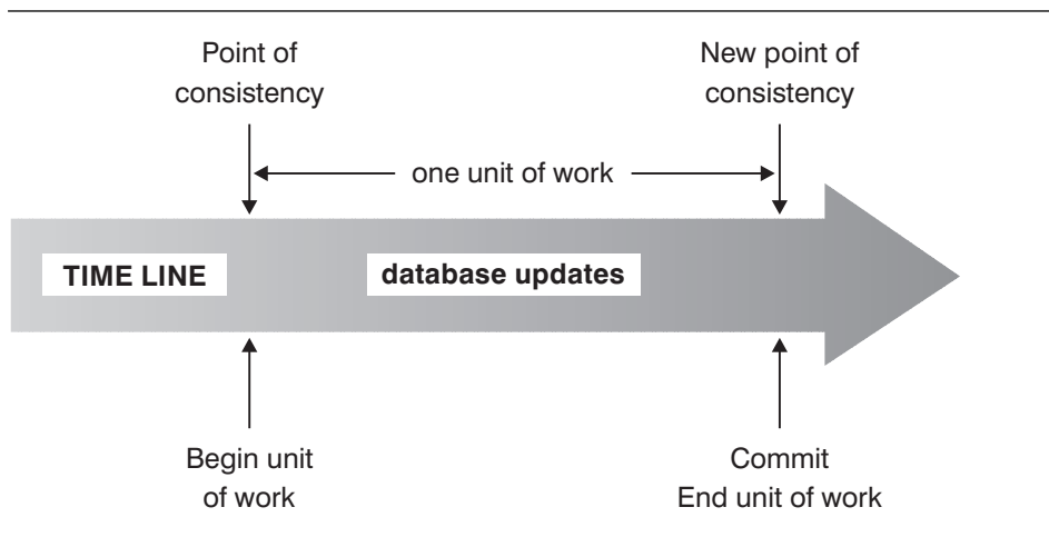
Figure 1. Unit of Work with a Commit Statement
