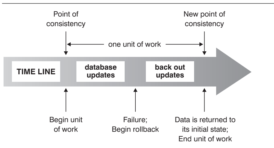
Figure 2. Unit of Work with a Rollback Statement
