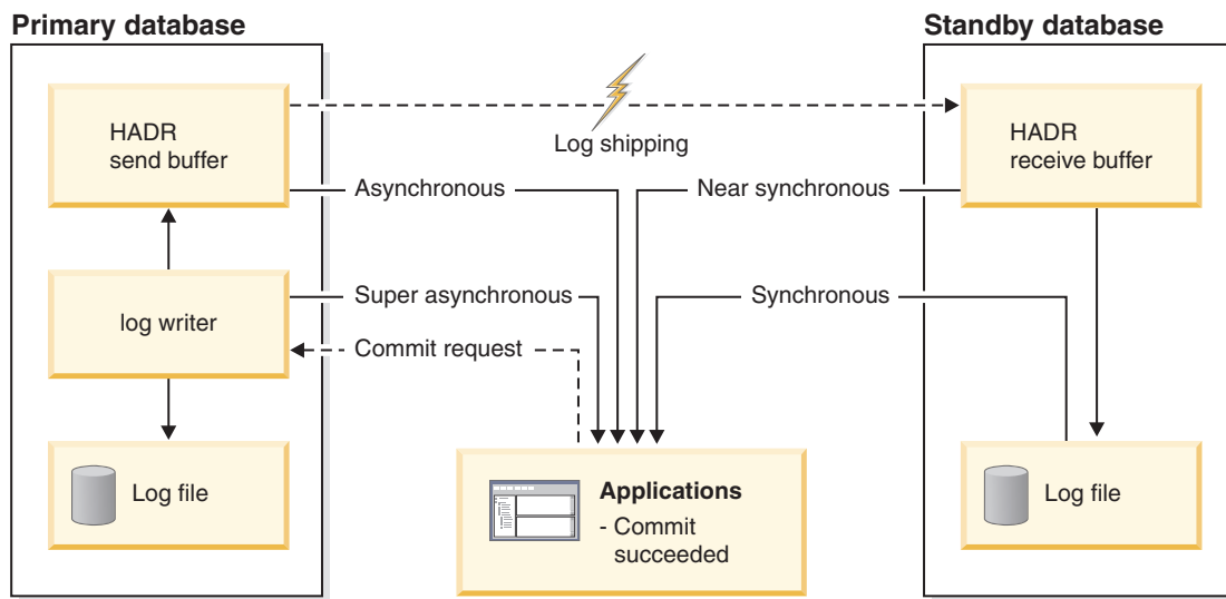
Figure 49. Synchronization modes for high availability and disaster recovery (HADR)
