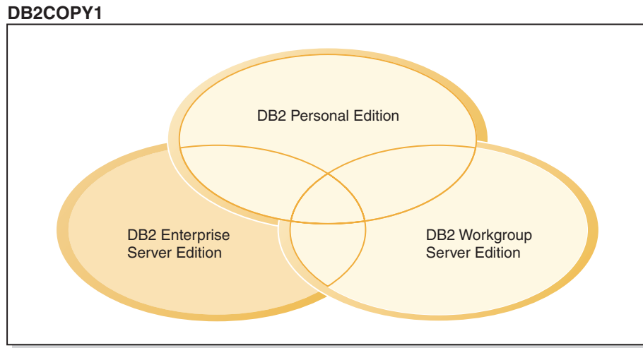
Figure 1. Shared components among different DB2 database products within the same DB2 copy
