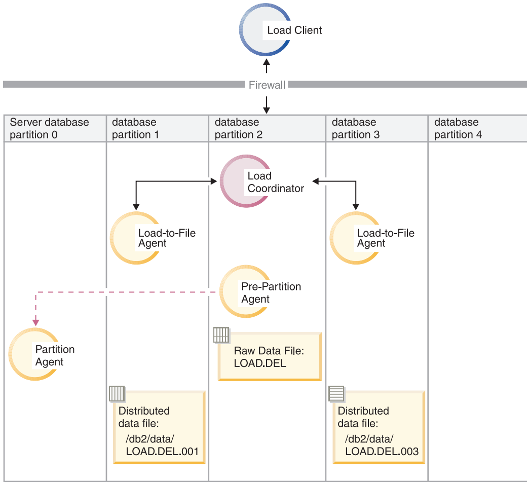
Figure 43. Loading data into database partitions 1 and 3 using one partitioning agent.. This diagram illustrates the behavior that results when the previous command is issued. Data is loaded into database partitions 1 and 3, using 1 partitioning agent running on database partition 0.
