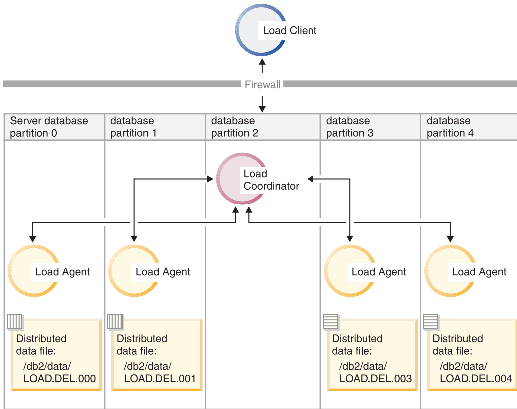
Figure 44. Loading data into all database partitions where a specific table is defined. This diagram illustrates the behavior resulting when the previous command is issued. Distributed data is loaded to all database partitions where TABLE1 is defined.
