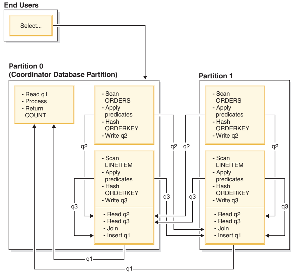
Figure 58. Directed Inner-Table and Outer-Table Join Example
