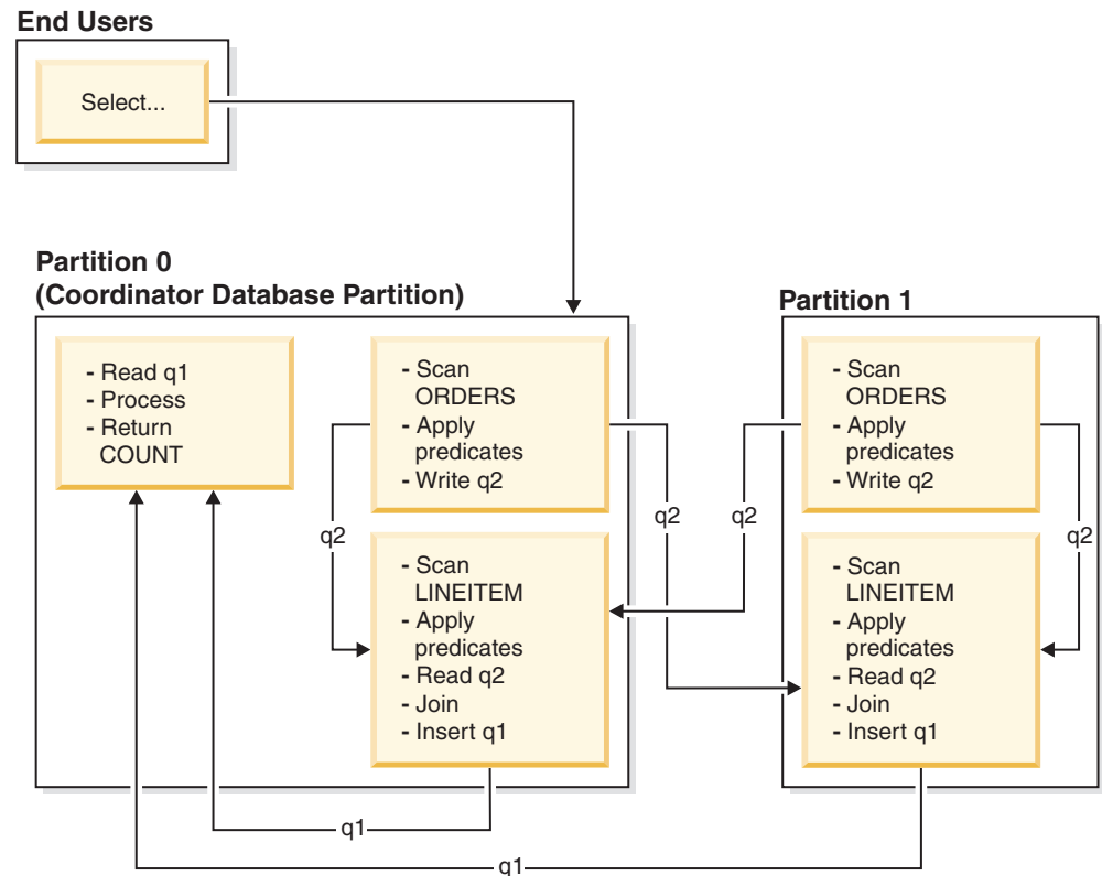
Figure 56. Broadcast Outer-Table Join Example
