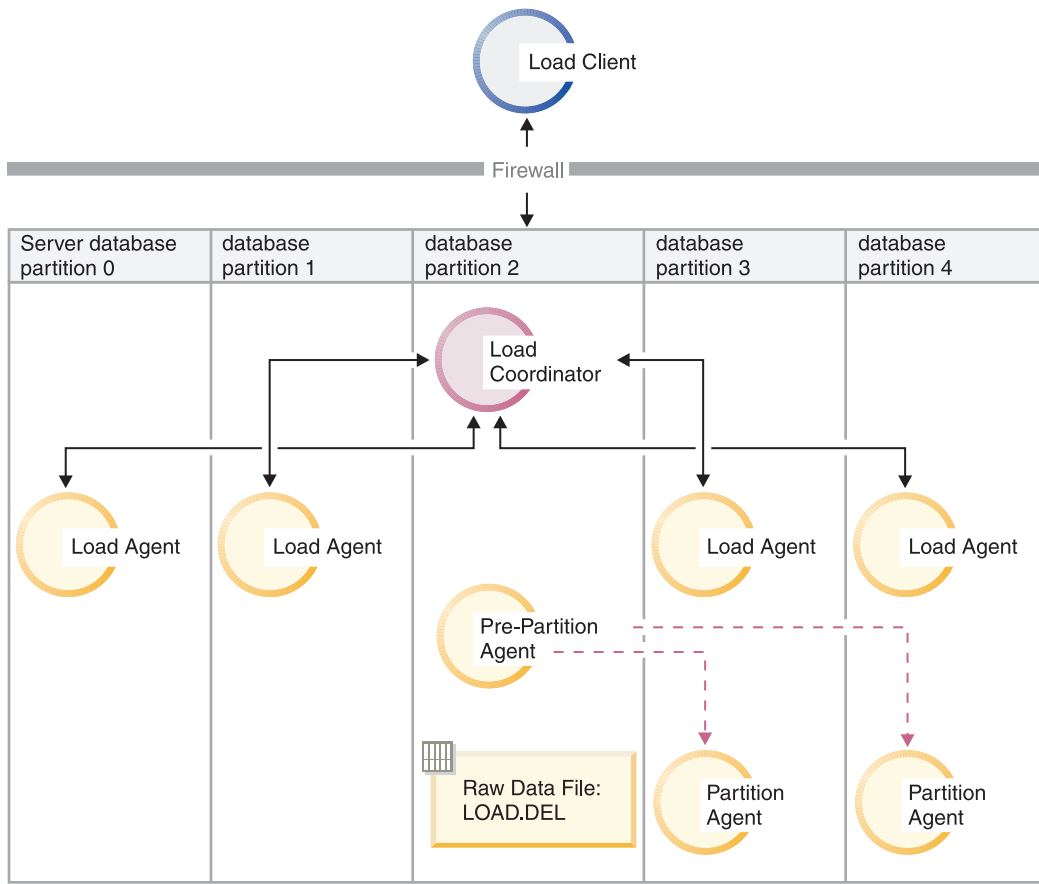
Figure 42. Loading data into database partitions 3 and 4. This diagram illustrates the behavior resulting when the previous command is issued. Data is loaded into database partitions 3 and 4.
