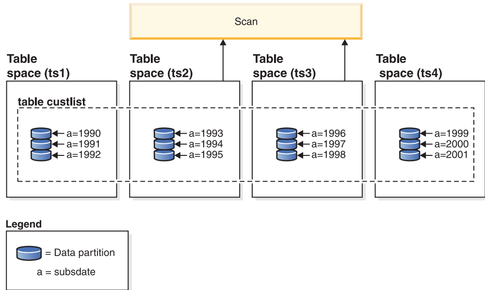
Figure 48. The performance benefits of data partition elimination
