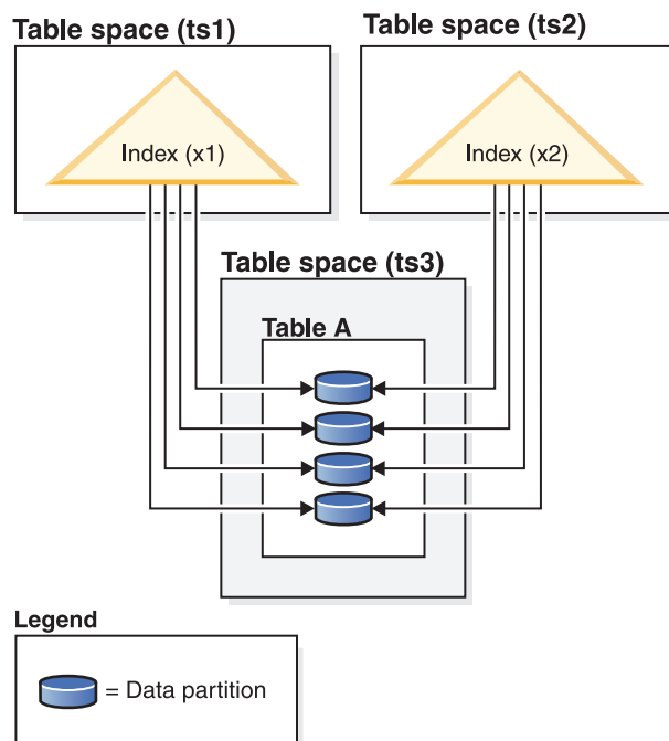
Figure 50. Nonpartitioned indexes on a partitioned table
