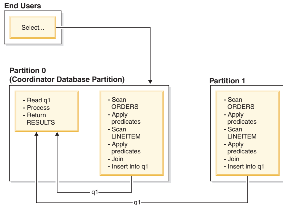
Figure 55. Collocated Join Example
