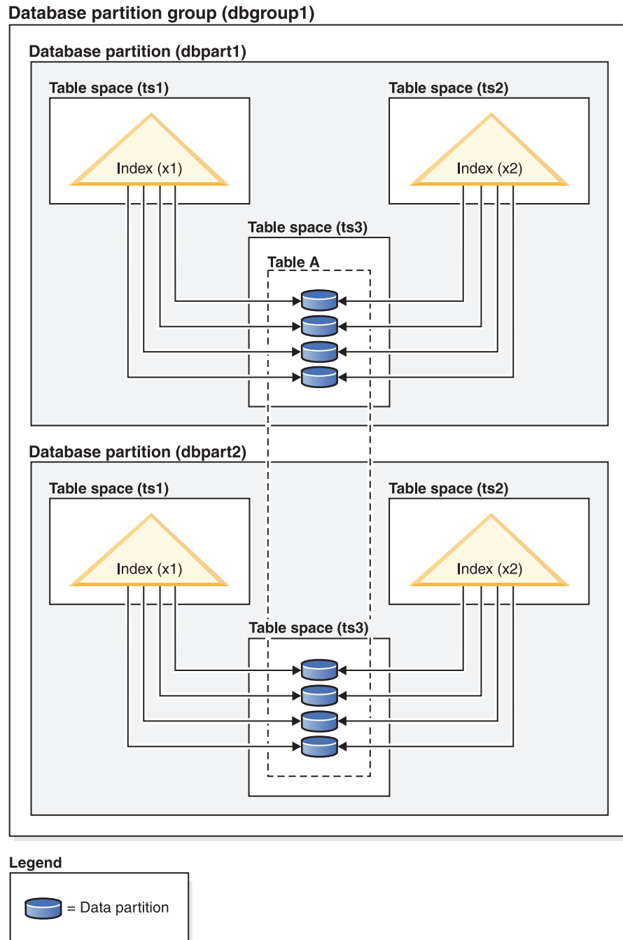
Figure 51. Nonpartitioned index on a table that is both distributed and partitioned
