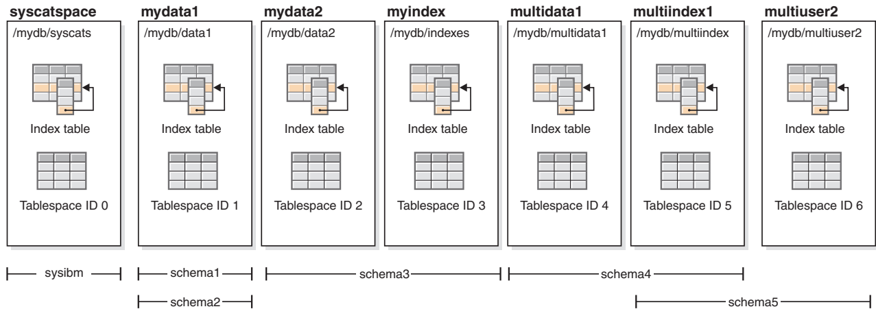
Figure 25. ORIGINALDB database
