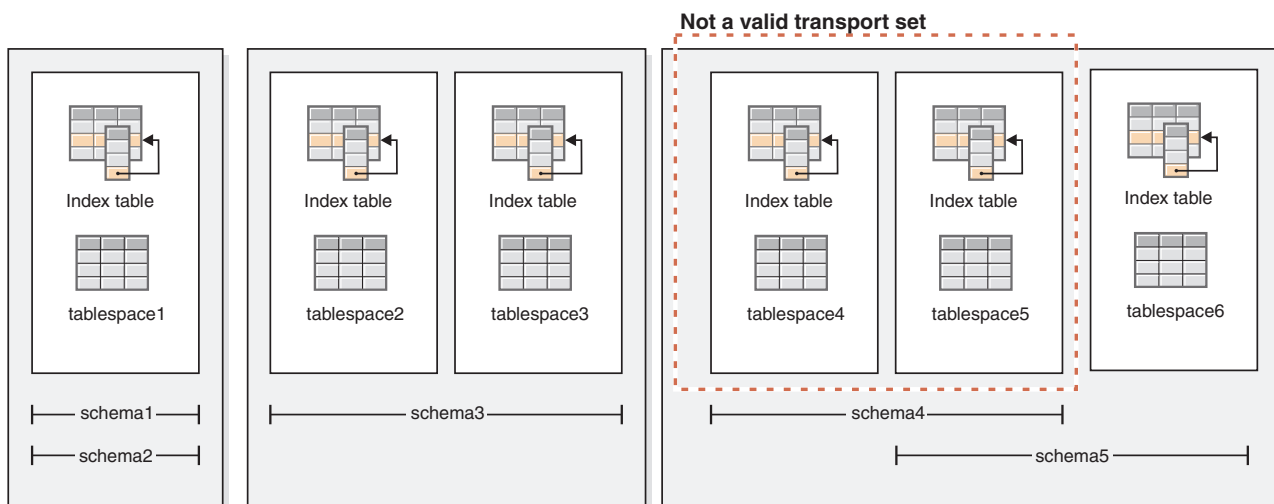
Figure 24. Sets of table spaces and schemas
