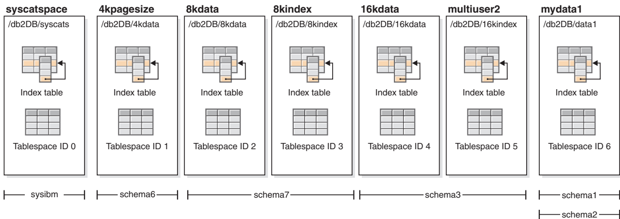
Figure 27. TARGETDB database after transport
