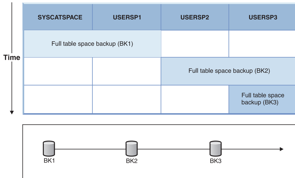
Figure 23. Backup images available for database SAMPLE
