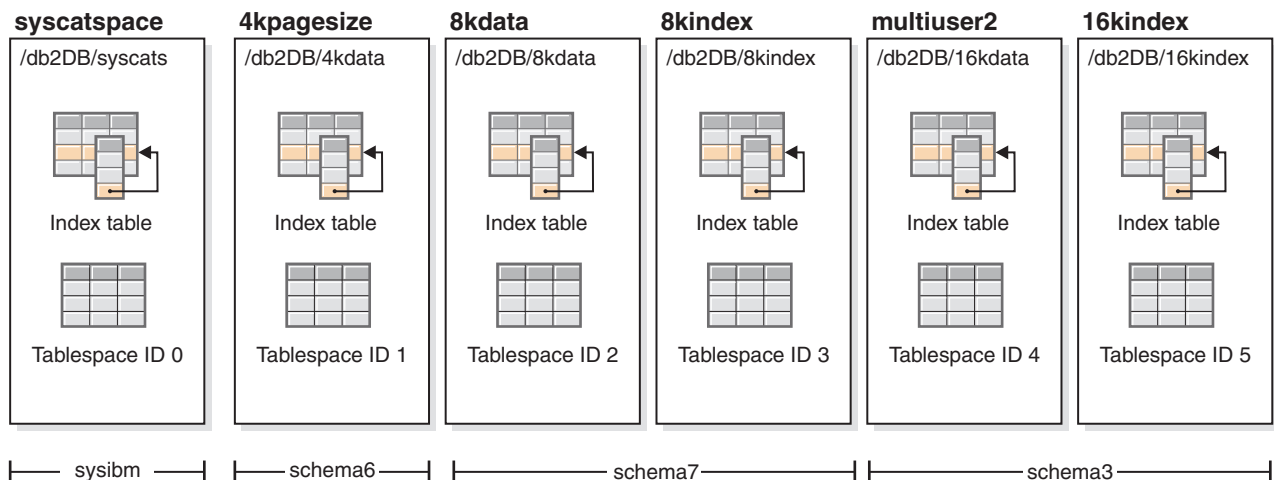
Figure 26. TARGETDB database
