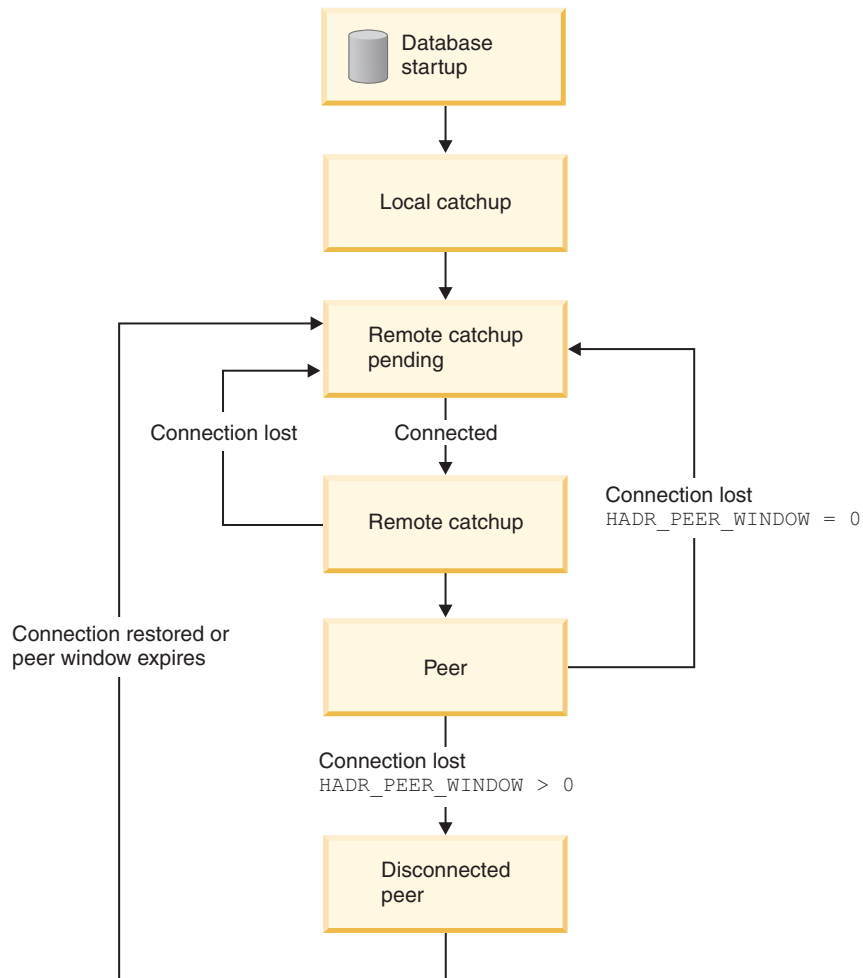
Figure 9. States of the standby database
