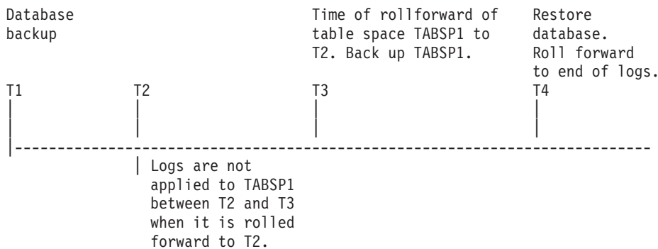
Figure 28. Table Space Backup Requirement
