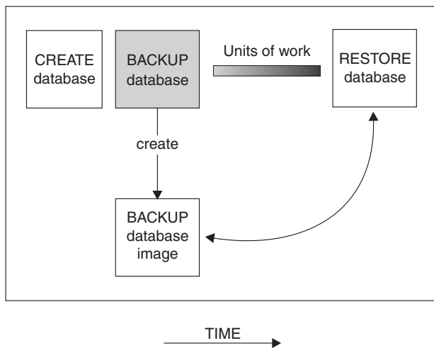
Figure 18. Version Recovery . Shows that units of work from the time of the backup to the time of the failure is lost.
