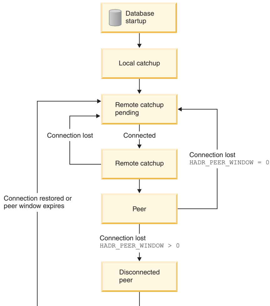
Figure 10. States of the standby database
