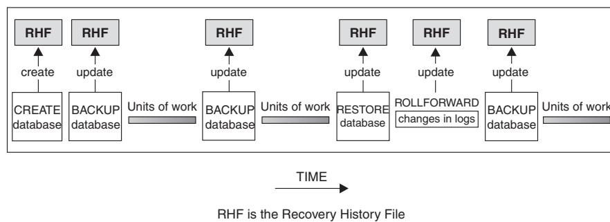
Figure 12. Creating and Updating the Recovery History File
