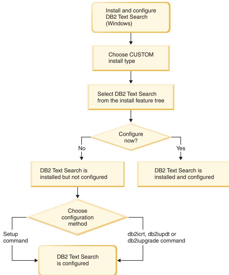
Figure 4. Installing and configuring on Windows platforms
