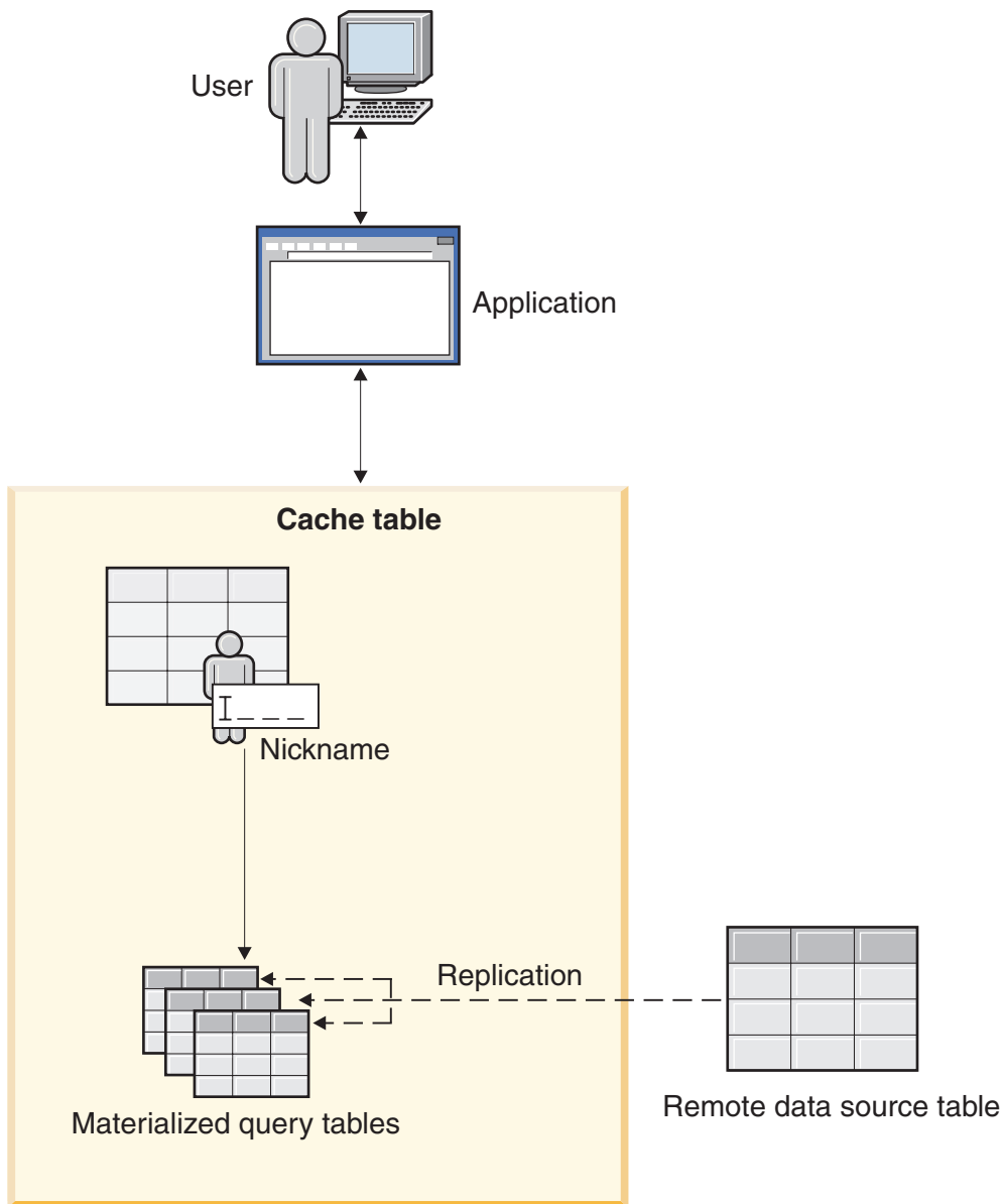
Figure 14. Cache table.
