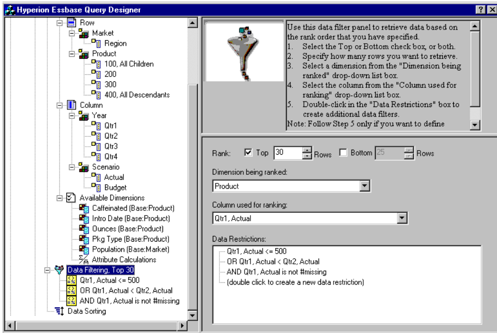
Figure 94: Data Filtering
