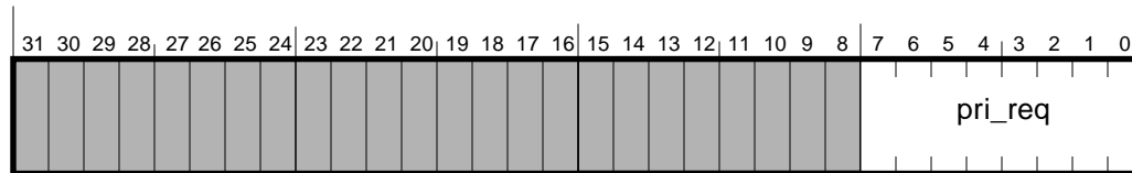
Figure 5-15 — FairnessControl register
