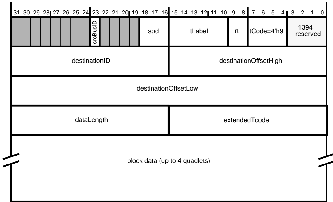
Figure 7-12 — Lock request transmit format
