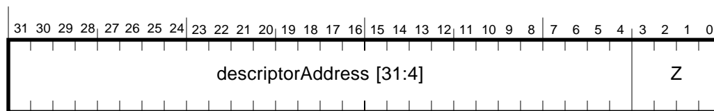
Figure 10-4 — CommandPtr register format
