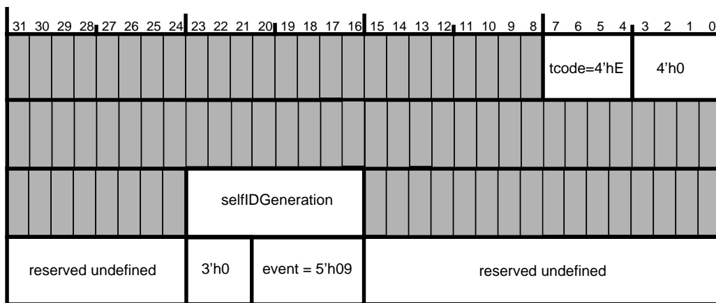
Figure 8-6 — AR Request Context Bus Reset packet format
