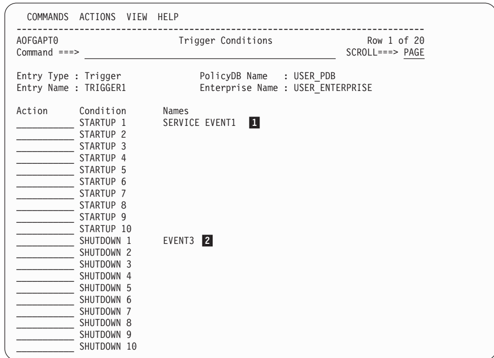
Figure 161. Trigger Conditions Panel
