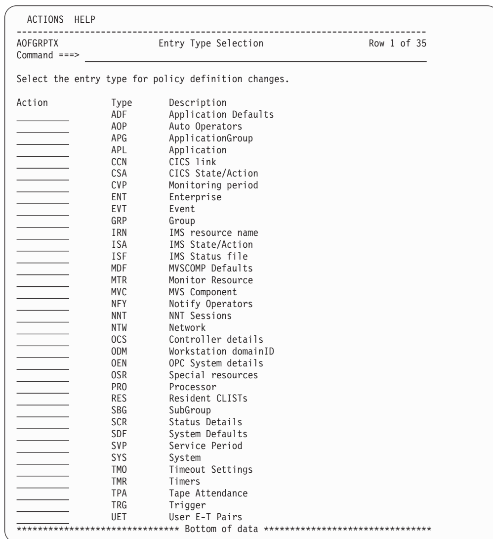
Figure 267. Entry Type Selection Panel
