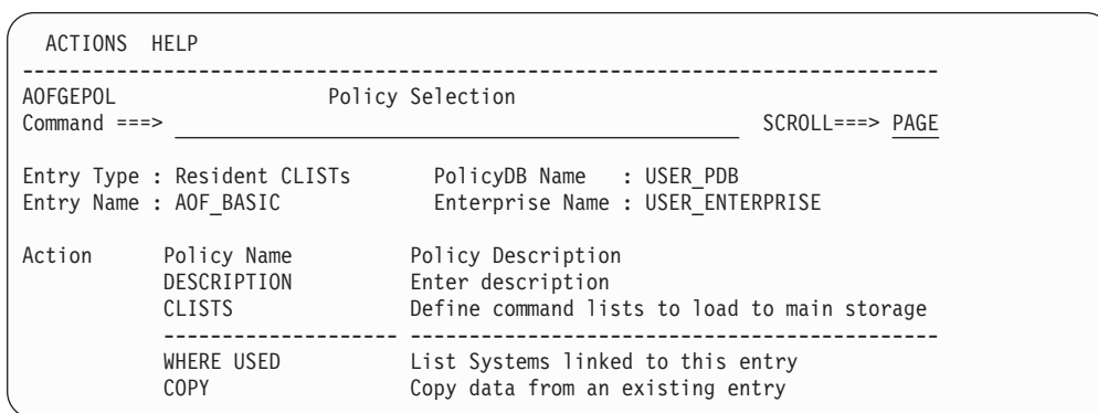
Figure 223. Policy Selection Panel for Resident CLISTs
