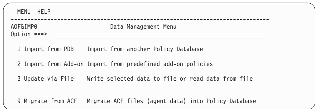
Figure 245. Data Management Menu Panel
