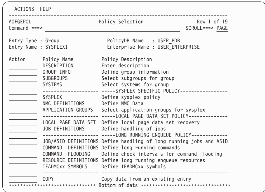
Figure 4. Policy Selection Panel for Sysplex Groups
