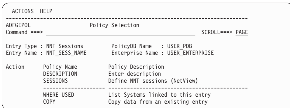
Figure 220. Policy Selection Panel for NNT Sessions
