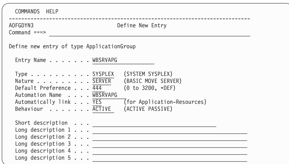
Figure 43. Define New Entry Input Panel for WBSRVAPG
