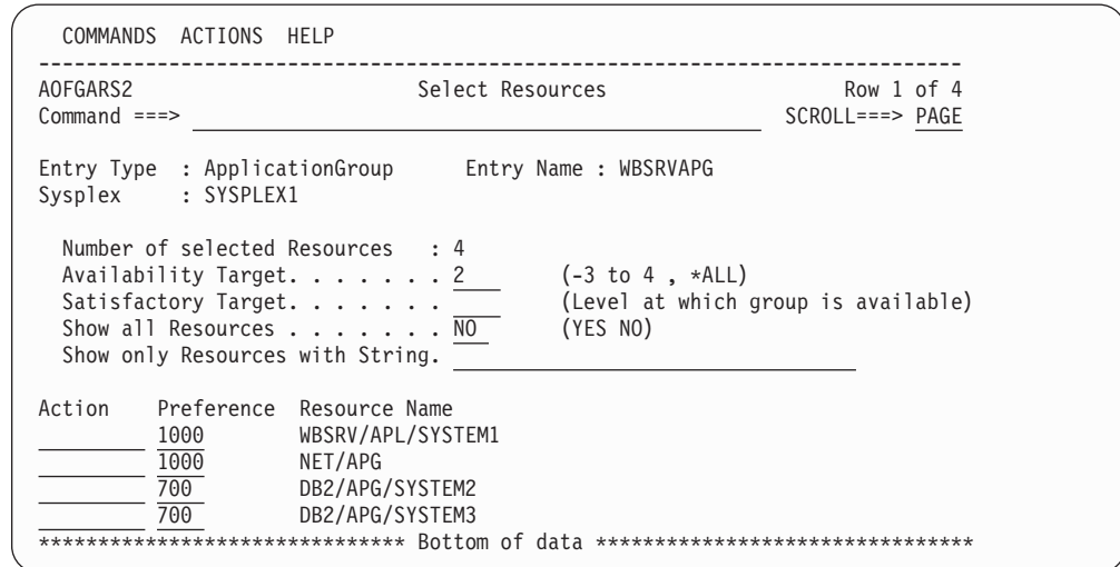
Figure 44. Final Select Resources Panel for WBSRVAPG
