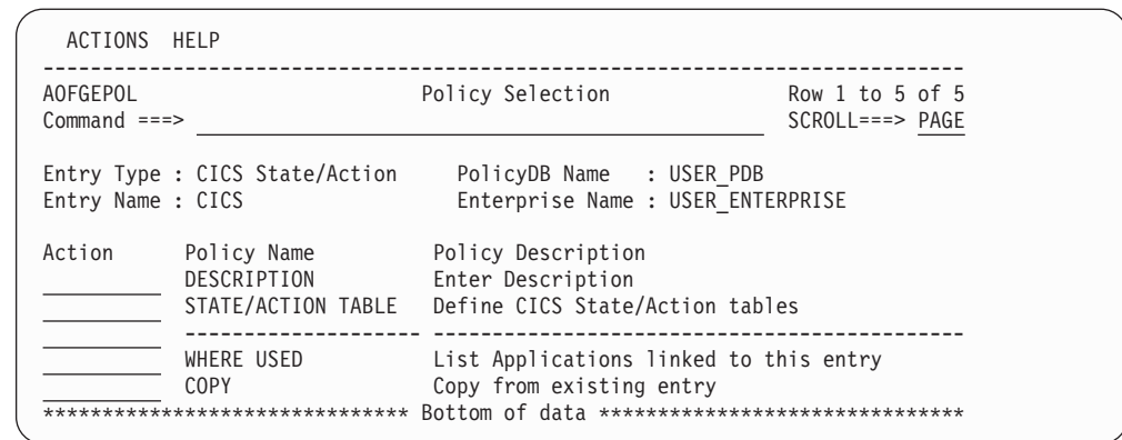
Figure 181. Policy Selection Panel for CICS State/Action Tables
