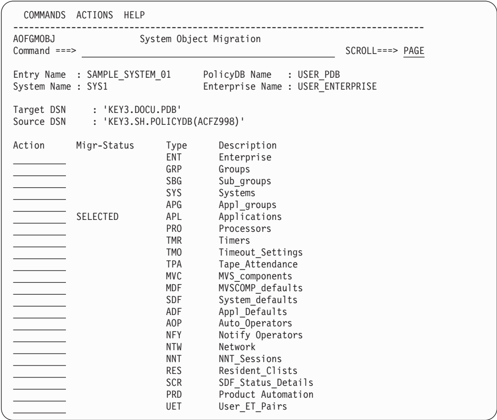
Figure 257. System Object Migration Panel
