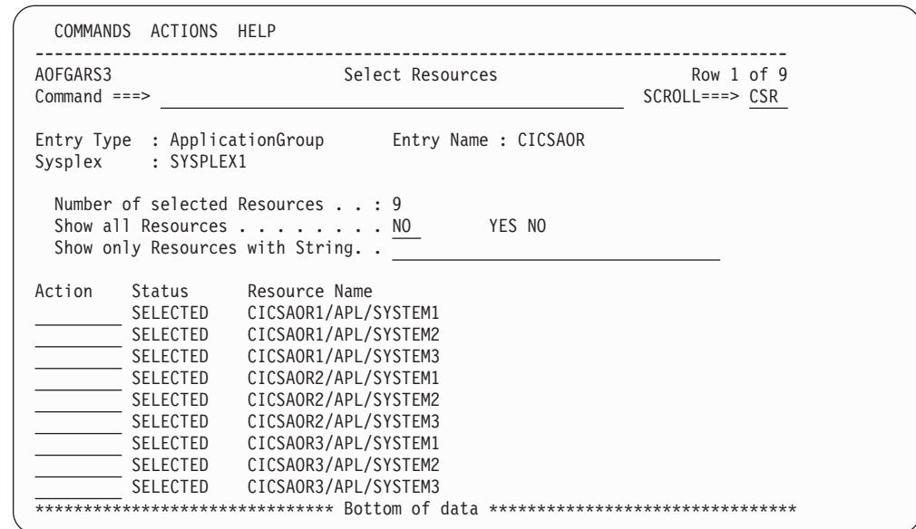
Figure 27. Resources for the CICS AOR Sysplex Application Group
