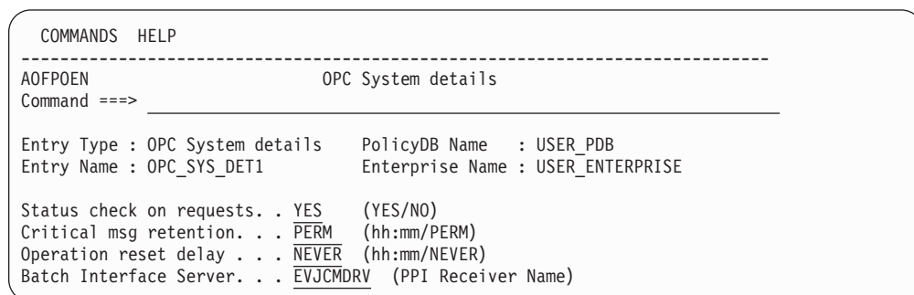
Figure 194. OPC System Details Panel
