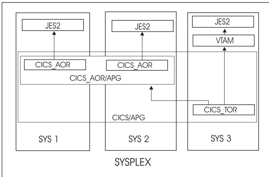
Figure 19. Relationship in a Sysplex
