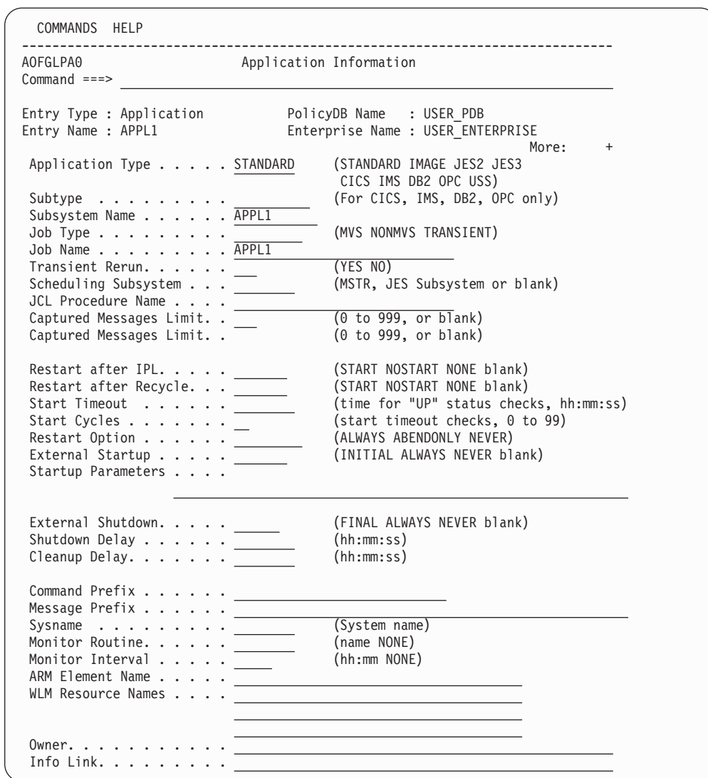
Figure 107. Application Information Panel
