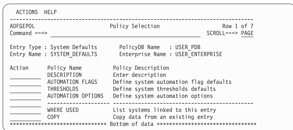
Figure 210. Policy Selection Panel for System Defaults
