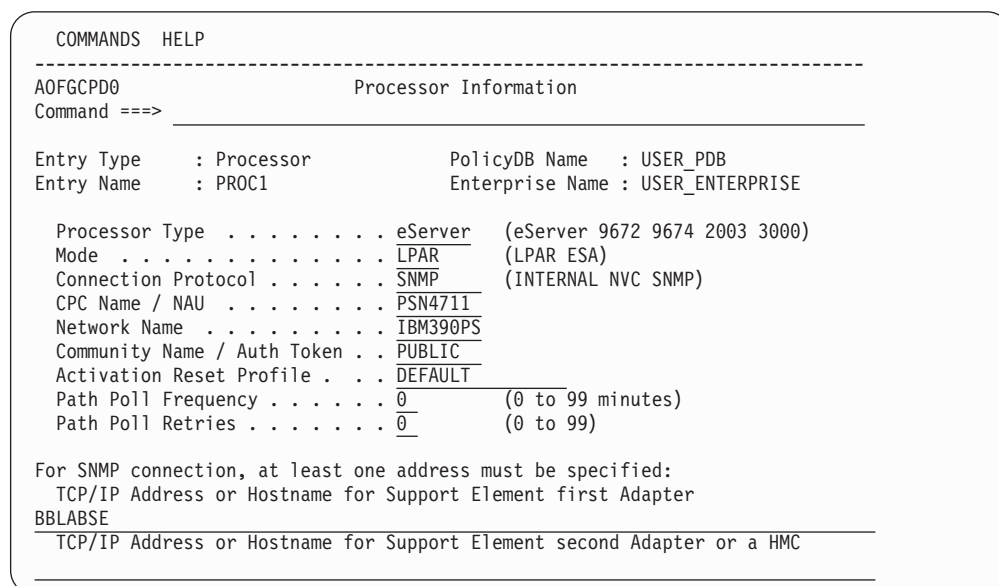
Figure 165. Processor Information Panel
